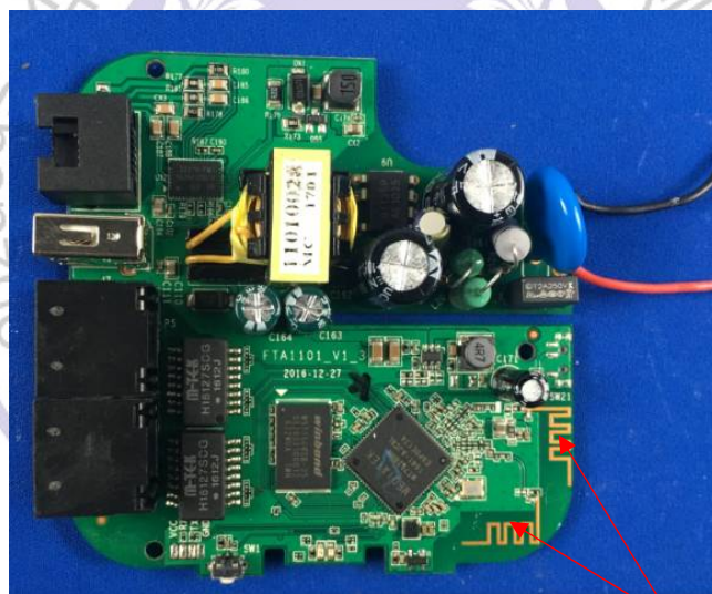
WIFI Antenna
