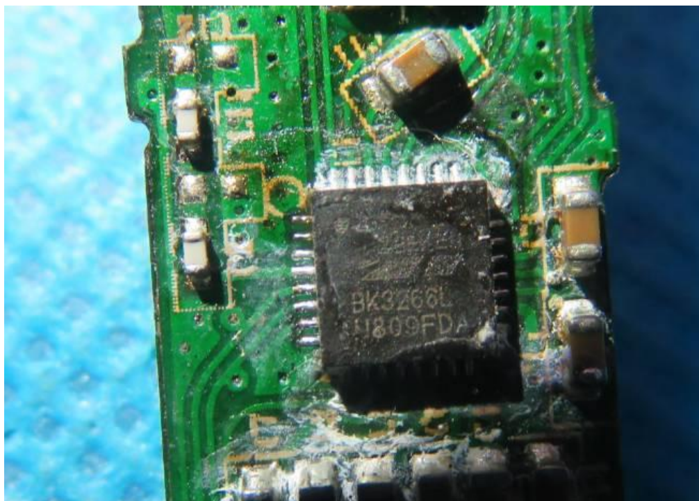
INTERNAL VIEW OF EUT-3
