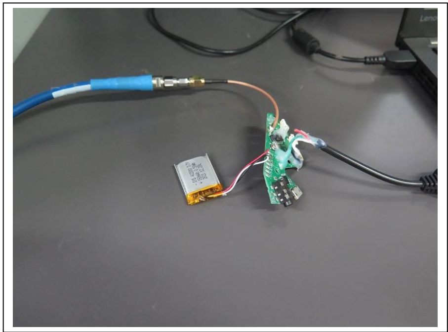
Conducted RF
