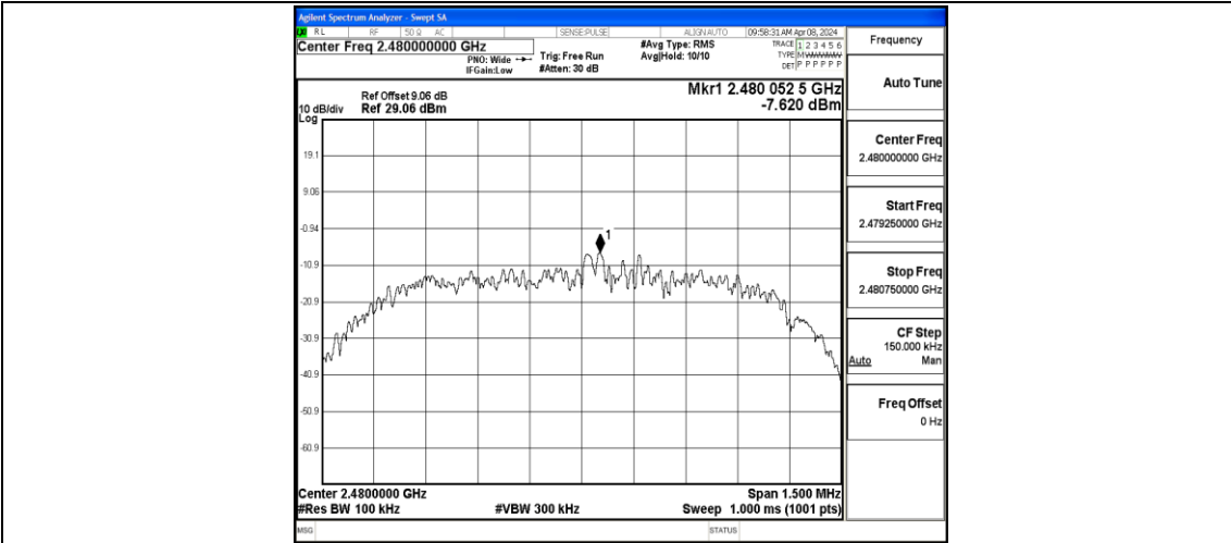
2DH5-Ant1-2480-0~Reference-PASS
