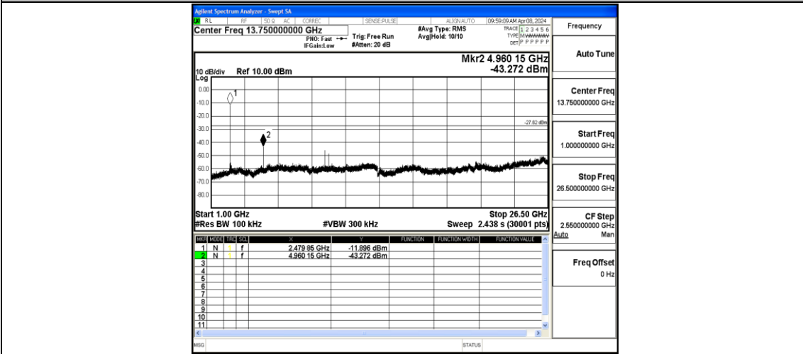
2DH5-Ant1-2480-1000~26500-PASS
