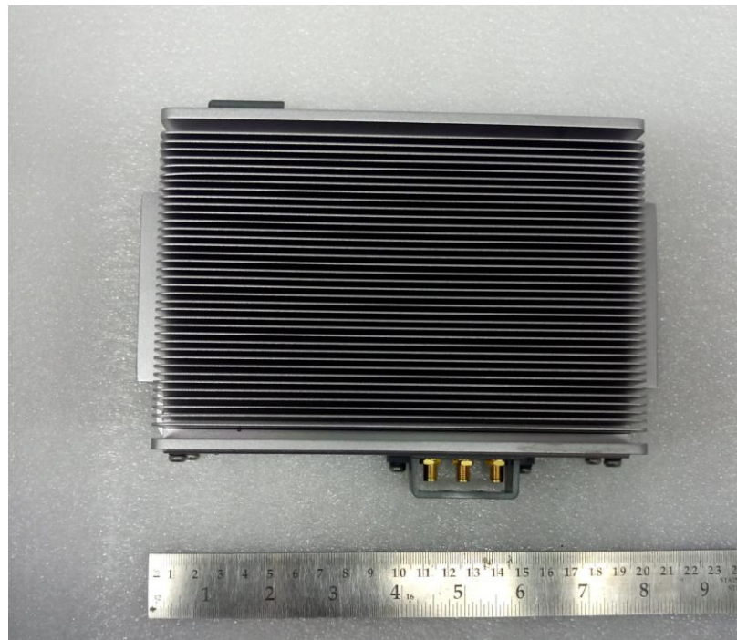
UDU Dimensional View
