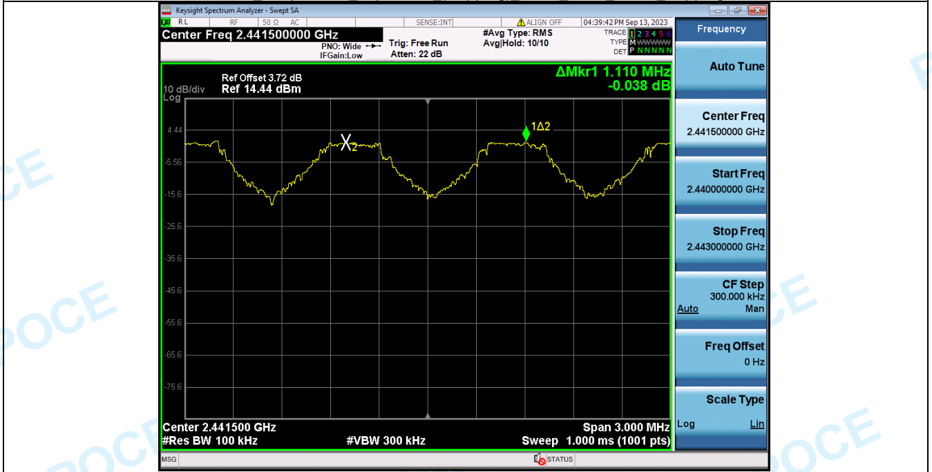
Carrier_Frequencies_Separation_(Hopping)_NVNT_ANT1_2-DH5_Hopping
