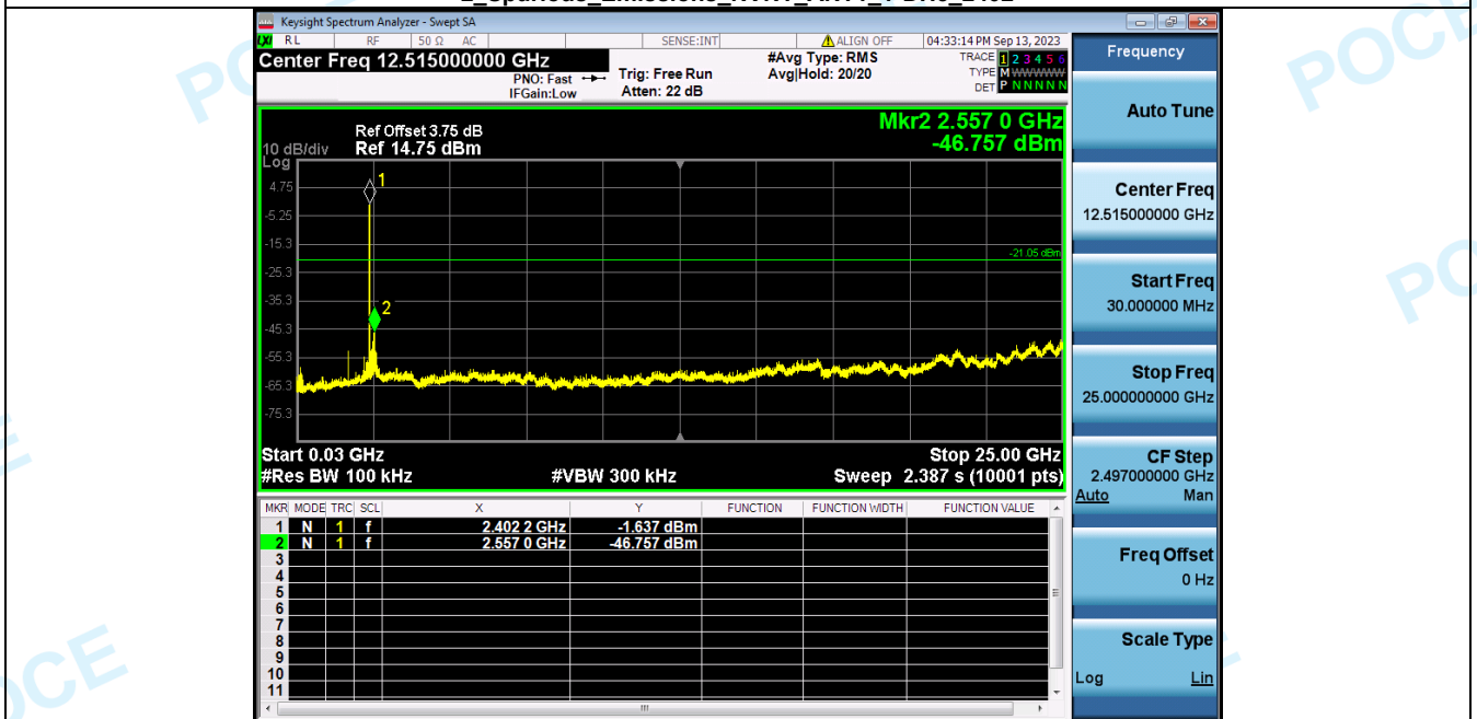
2 Spurious Emissions_NVNT_ANT1_1-DH5_2402
