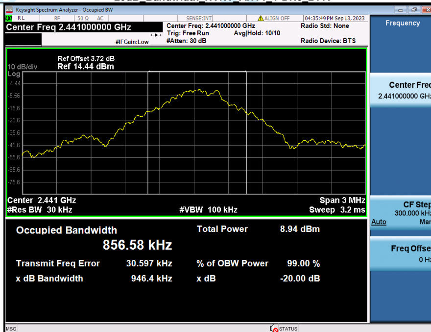
-20dB Bandwidth_NVNT_ANT1_1-DH5_2441
