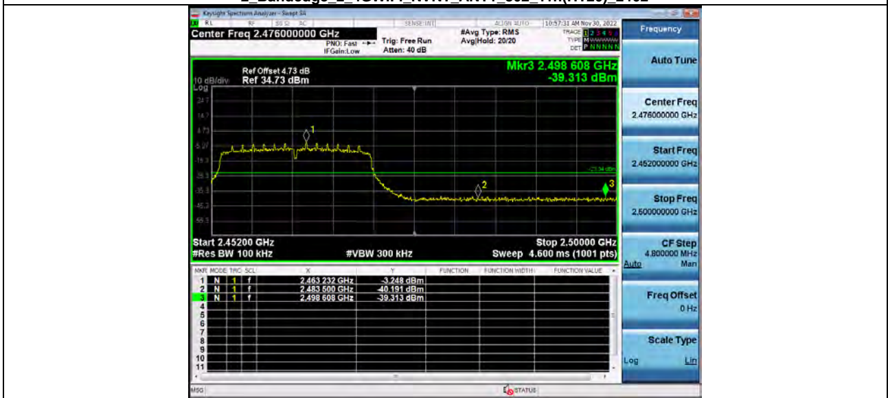
2_Bandedge 2_4GWiFi_NVNT_ANT1_802_11n(HT20)_2462
