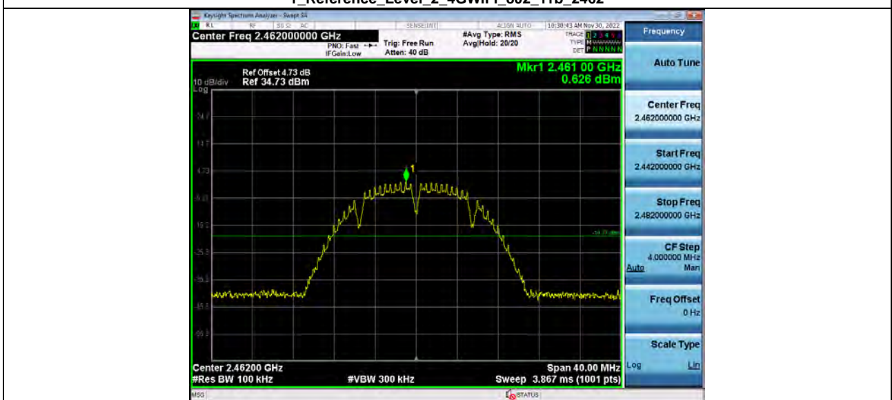
2_Spurious_Emission_2_4GWiFi_NVNT_ANT1_802_11b_2462
