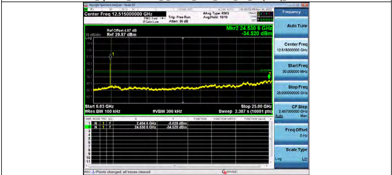
1_Reference_Level_2_4GWiFi_802_11n(HT20)_2437
