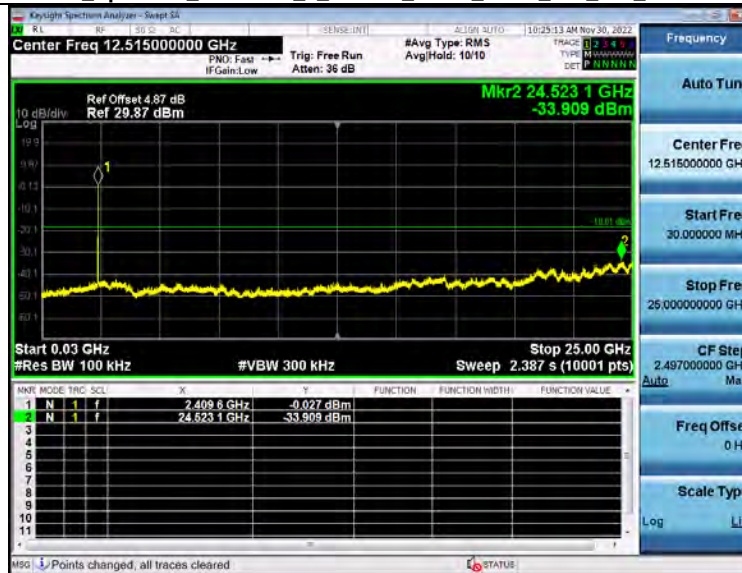
2 Spurious Emission 2_4WiFi_NVNT_ANT1_802_11b_2412
