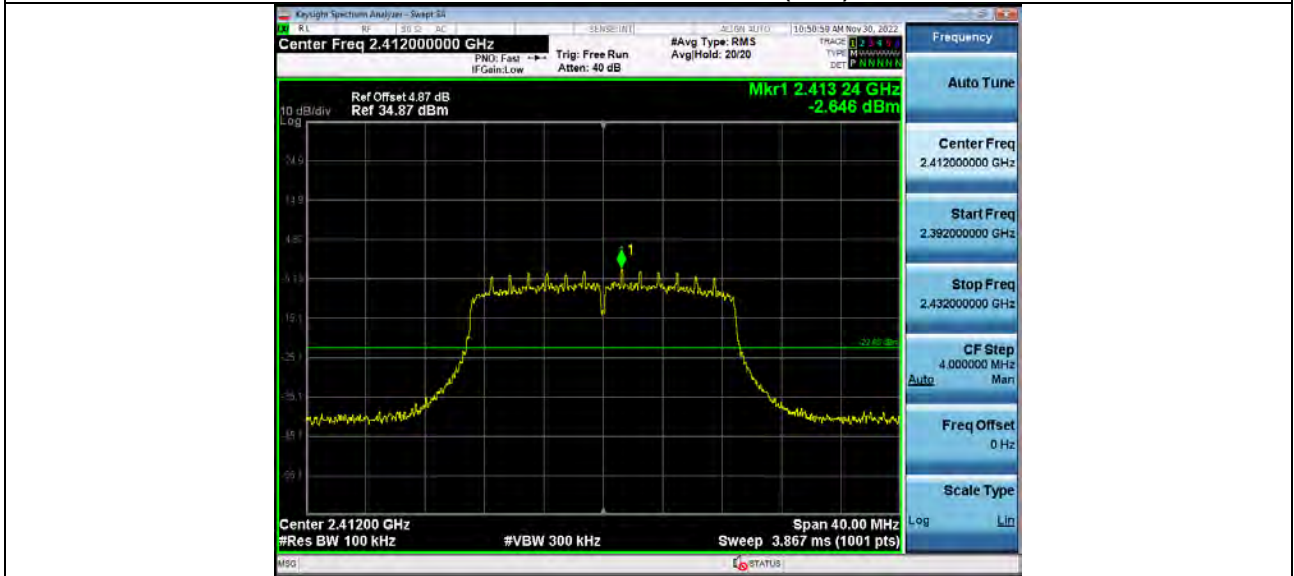
2_Bandedge_2_4GWiFi_NVNT_ANT1_802_11n(HT20)_2412
