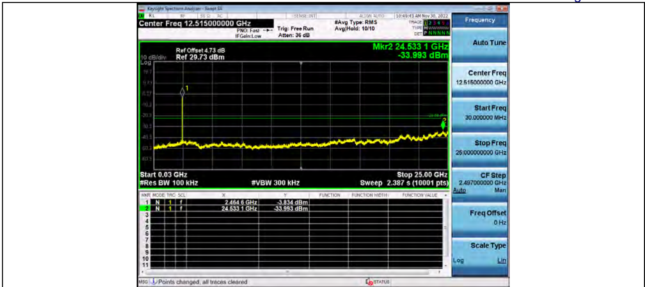
1_Reference_Level_2_4GWiFi_802_11n(HT20)_2412
