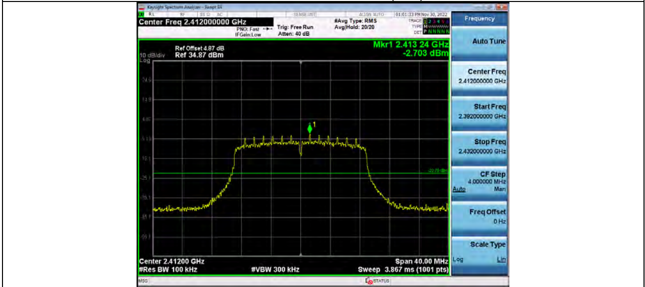
2_Spurious_Emission_2_4GWiFi_NVNT_ANT1_802_11n(HT20)_2412
