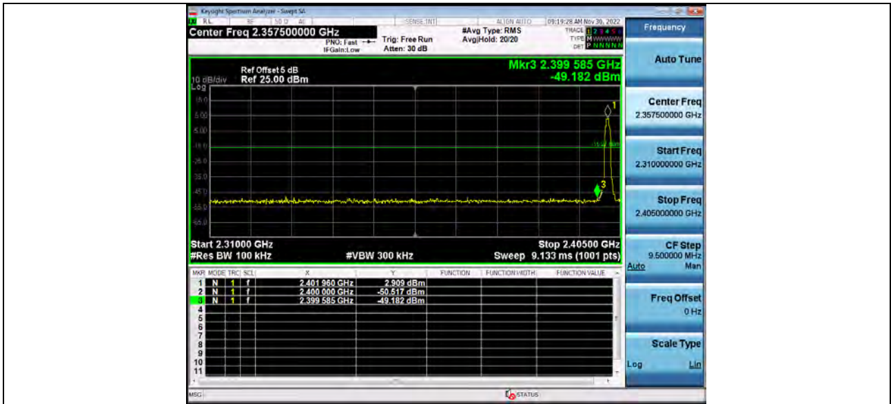
1_Reference_Level_BT_2-DH5_Hopping
