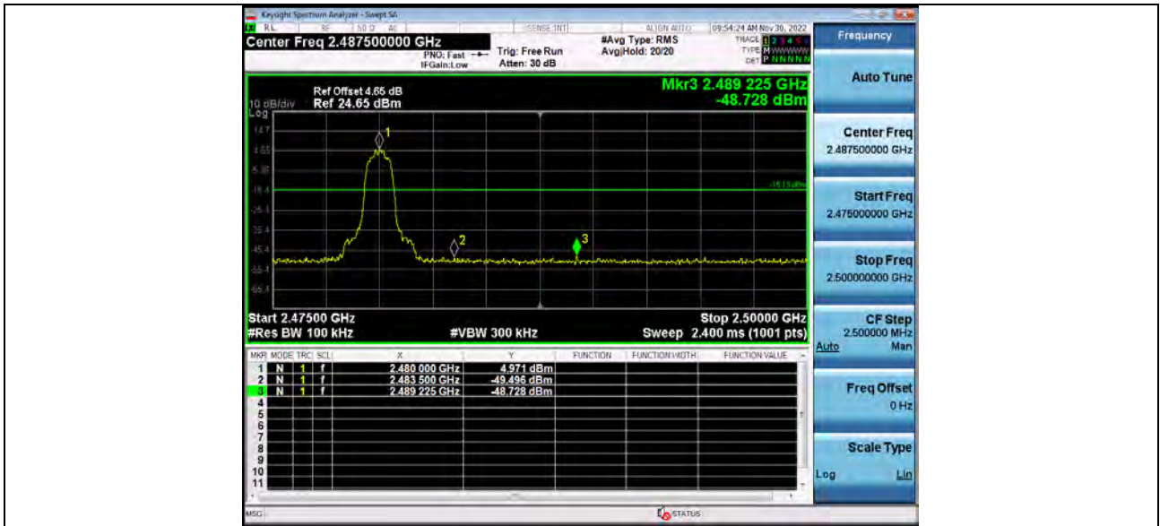
1_Reference_Level_BT_3-DH5_Hopping
