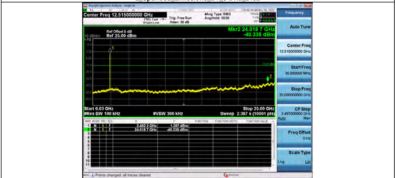
2_Spurious Emissions_BT_3-DH5_2402
