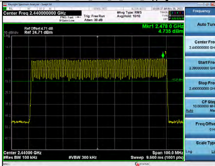
1_Reference_Level_BT_1-DH5_Hopping
