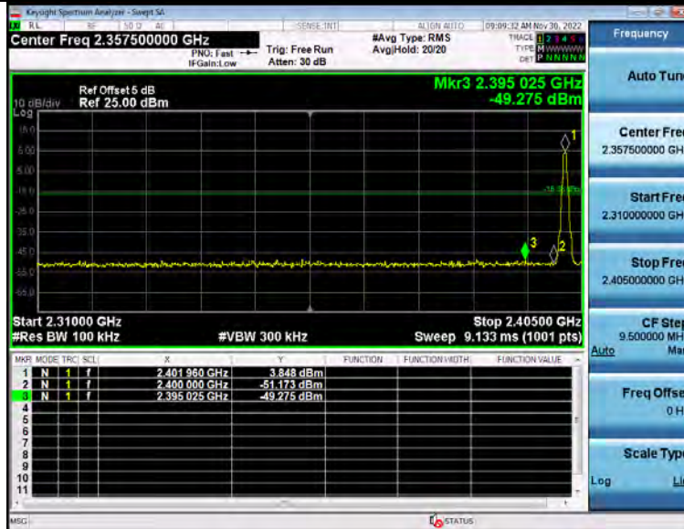
2_Bandedge_BT_1-DH5_2402
