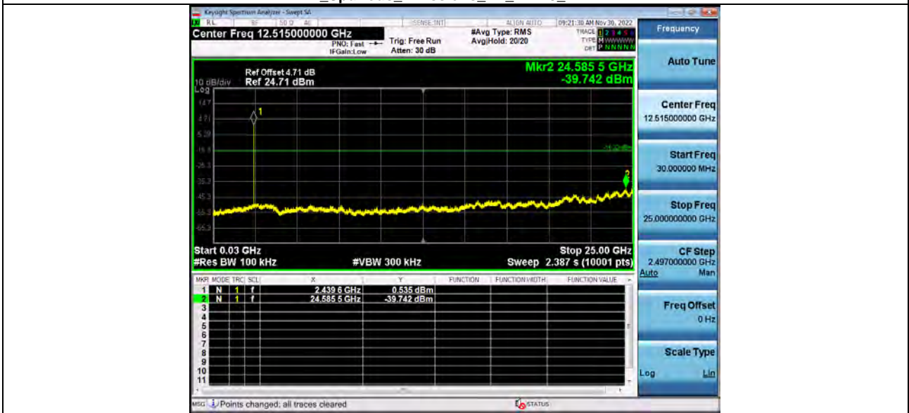
2_Spurious Emissions_BT_2-DH5_2441
