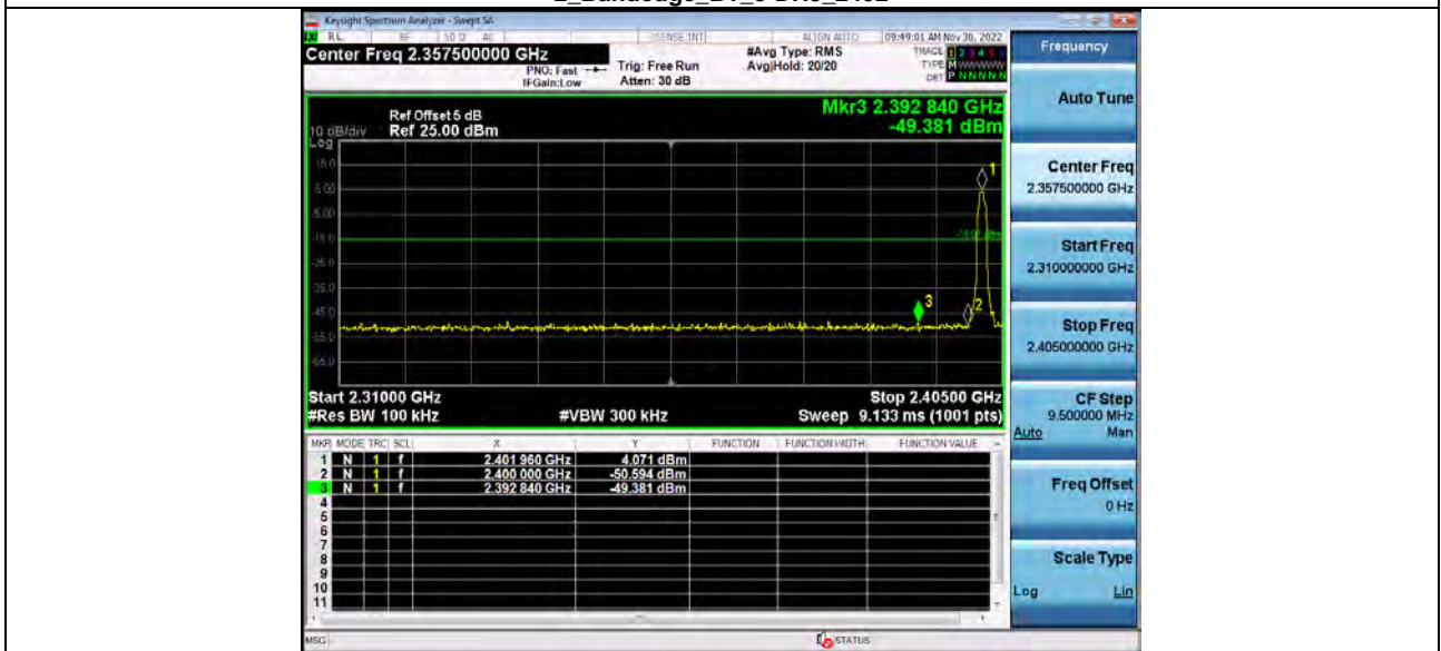
2_Bandedge_BT_3-DH5_2402
