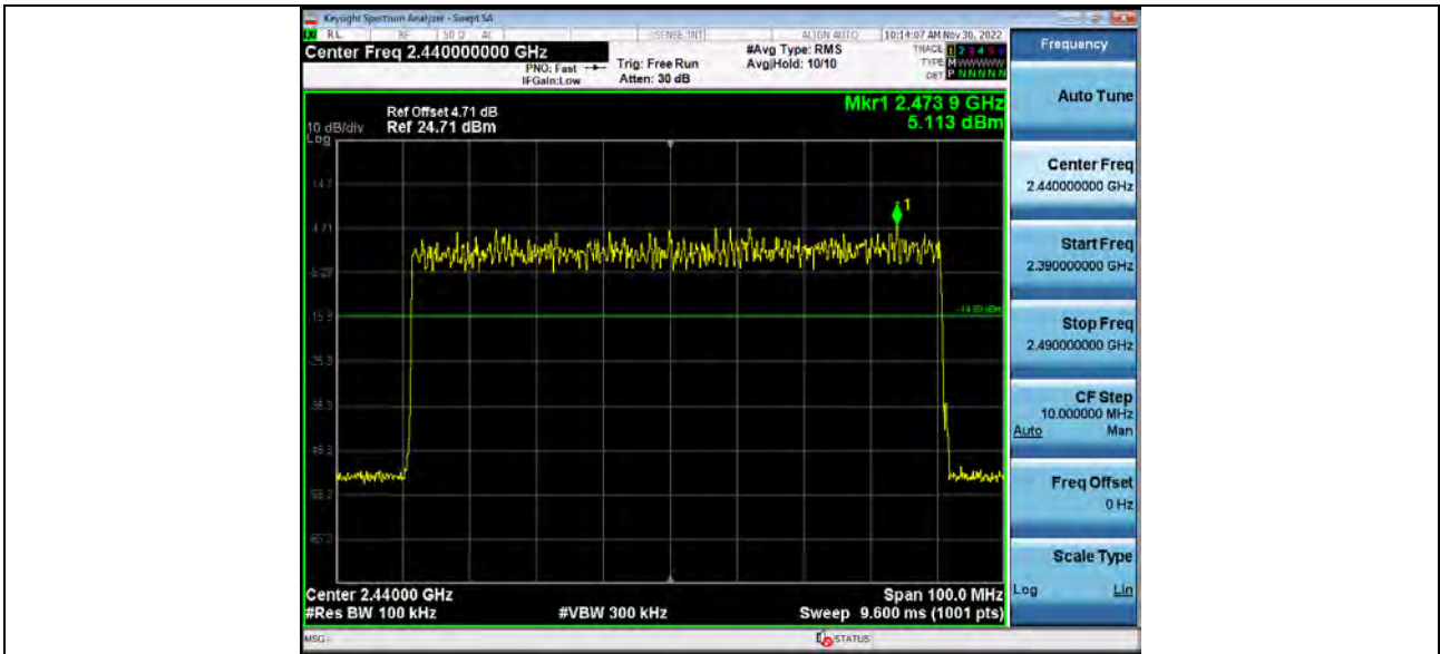
2_Band_Edge_(Hopping)_BT_3-DH5_Hopping
