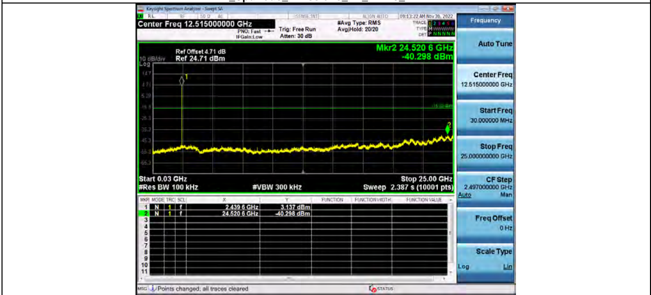
2_Spurious Emissions_BT_1-DH5_2441
