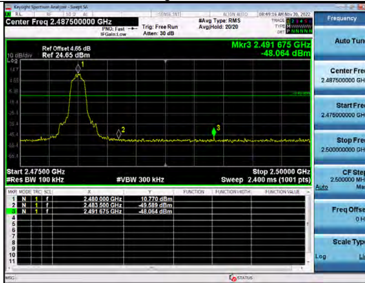
2_Bandedge_BT_2-DH5_2480
