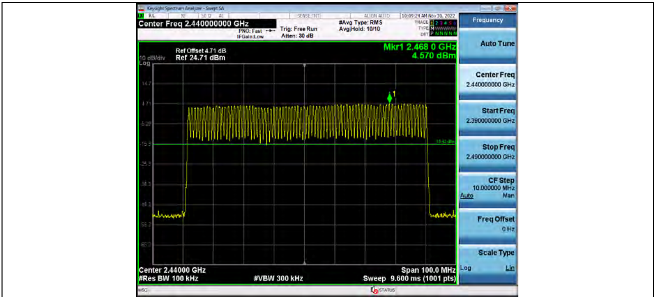
2_Band_Edge_(Hopping)_BT_1-DH5_Hopping
