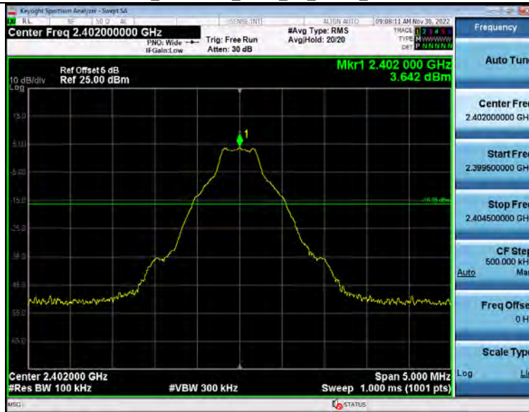
2_Bandedge_BT_1-DH5_2402
