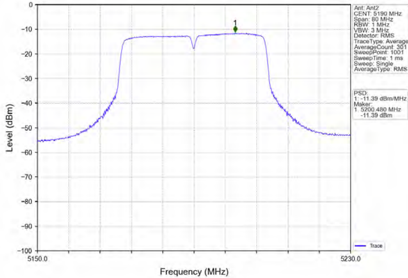
802.11n(HT40)_LCH_5190MHz_MIMO_NTNV
