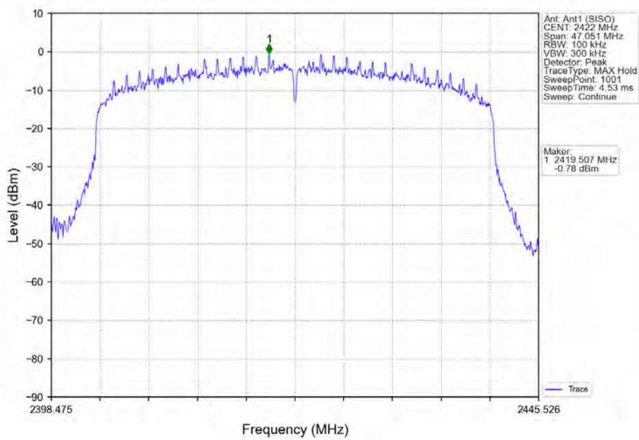
802.11ax(HEW40)_LCH_2422MHz_RU484_Left_Ant1 (SISO)_NTNV
