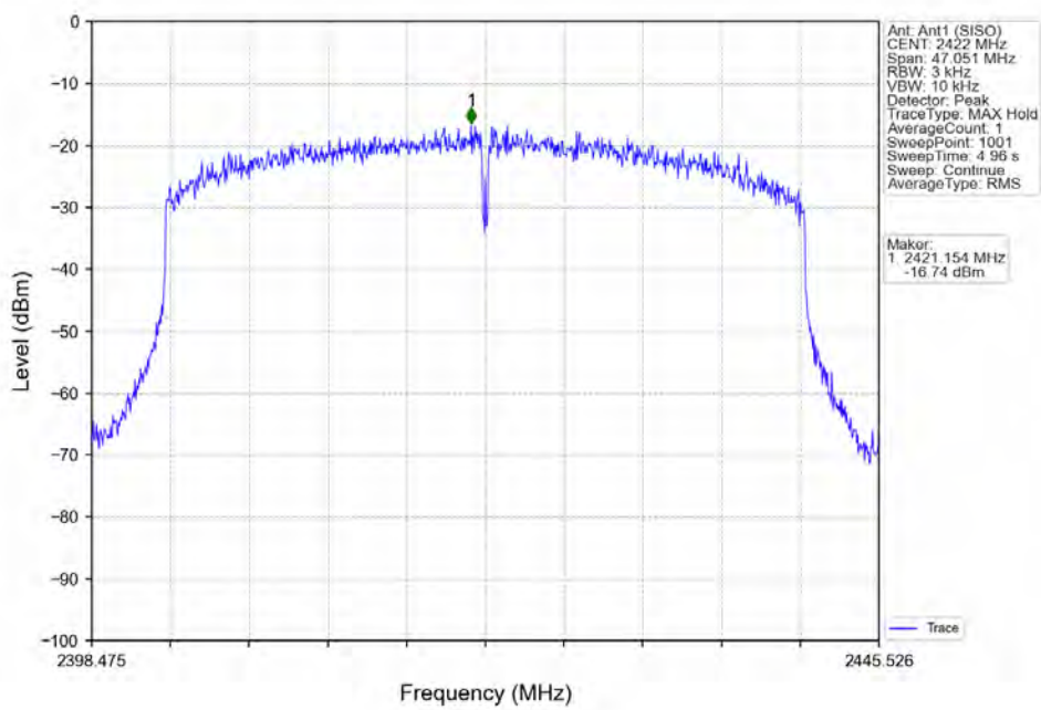
802.11ax(HEW40)_LCH_2422MHz_RU484_Left_Ant1 (SISO)_NTNV
