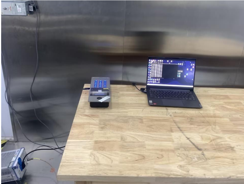
Conducted Emissions at Mains Terminals (150kHz-30MHz)
