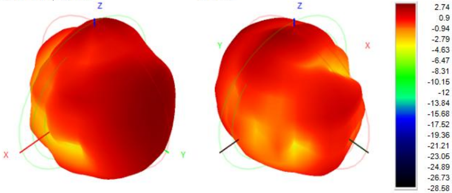
2500.0MHz H+V, Eff: 62.4%
