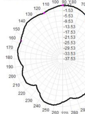
Total(H-XY), Max=2.40dBi, CirD=12.99
