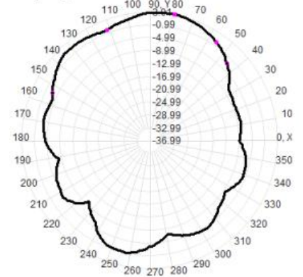
Total(H-XY), Max= 3.01dBi, CirD=13.24
