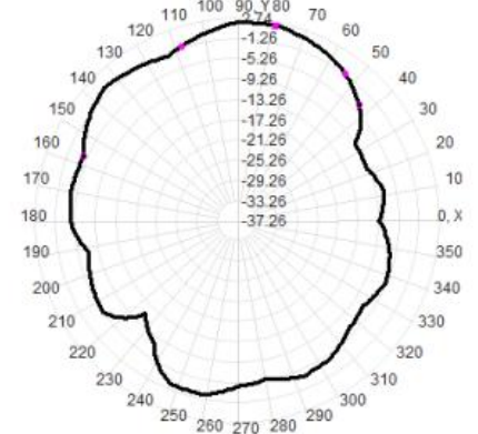
Total(H-XY), Max= 1.96dBi, CirD=13.71
