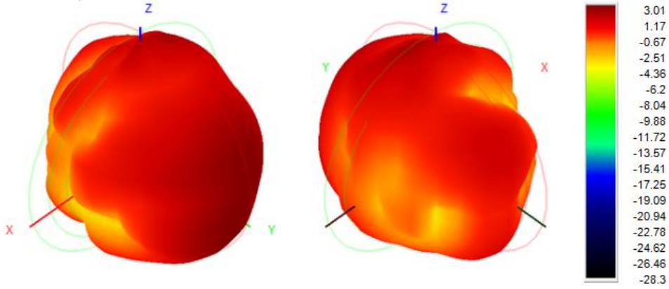
2450.0MHz H+V, Eff: 65.1%
