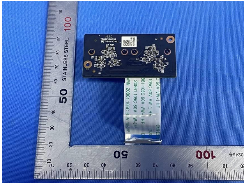
Temperature module 2
