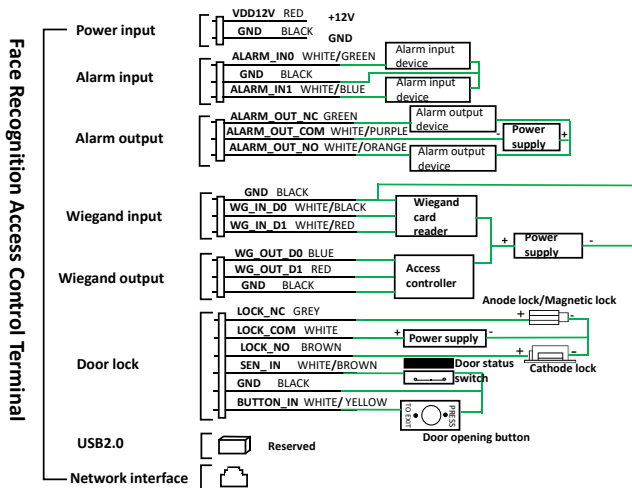
Figure 3-1 Wiring Schematic Diagrams
