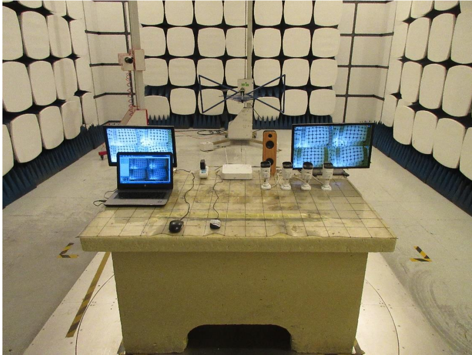
RADIATED EMISSION SET-UP PHOTOS, 30MHz ~ 1GHz
