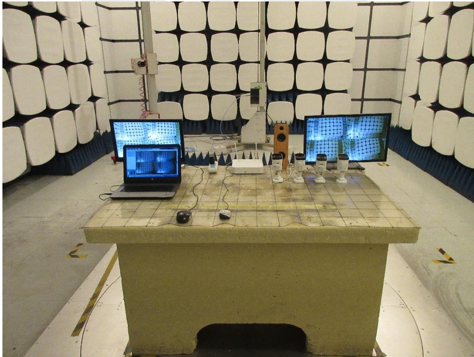
RADIATED EMISSION SET-UP PHOTOS, 1GHz ~ 18GHz
