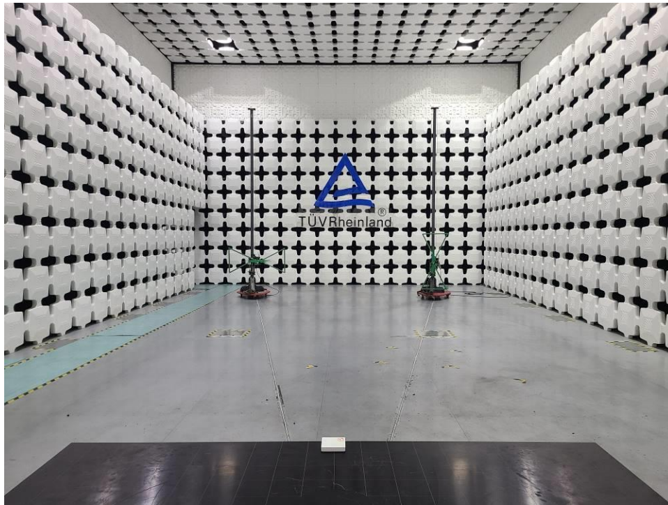
Photograph 3: Set-up photo for Radiated Emission, Below 1GHz
