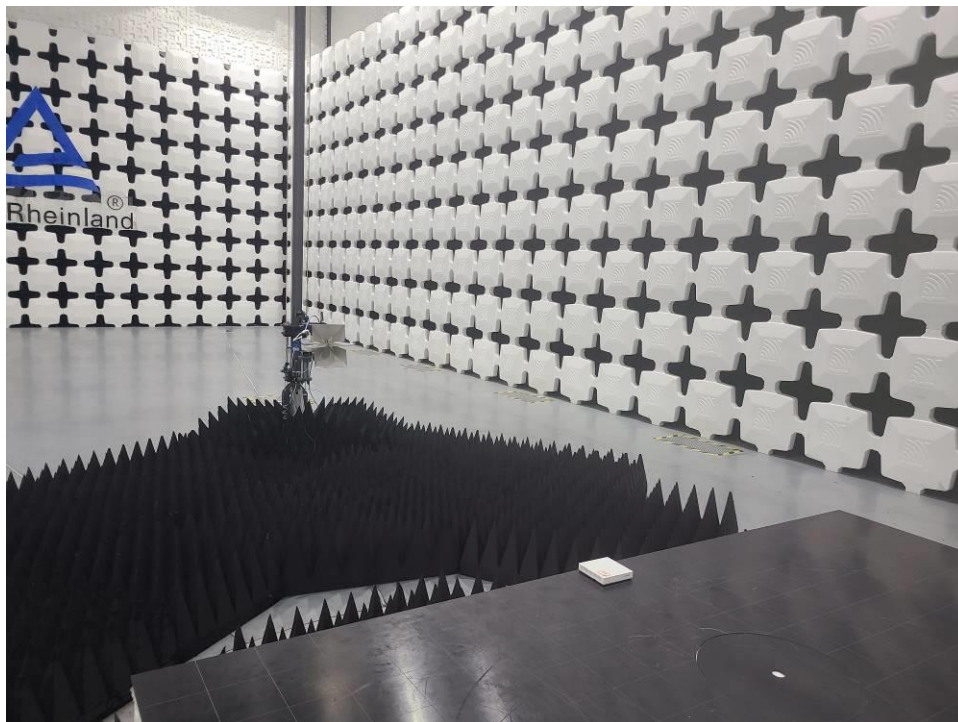
Photograph 4: Set-up photo for Radiated Emission, Above 1GHz
