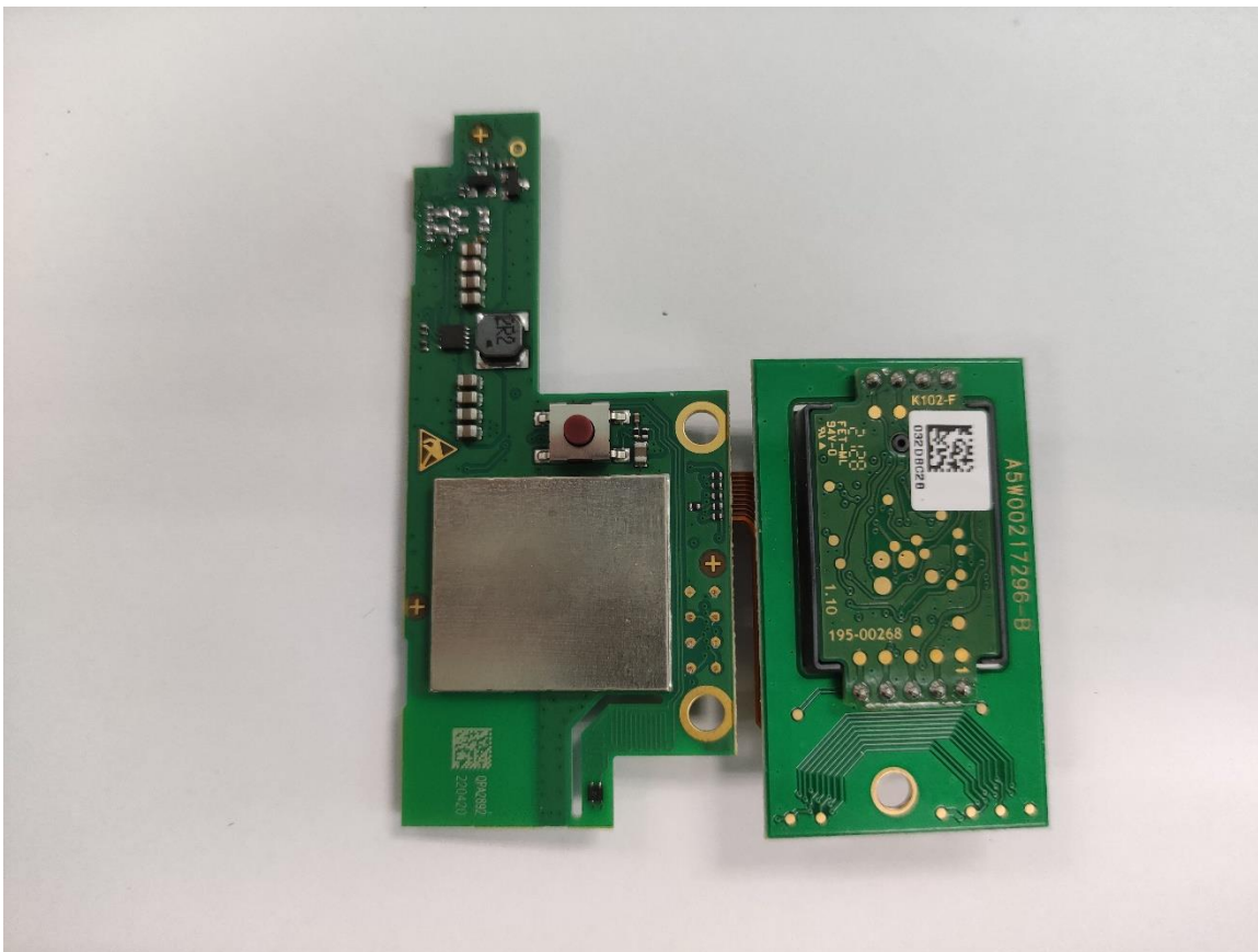
PCB bottom side
