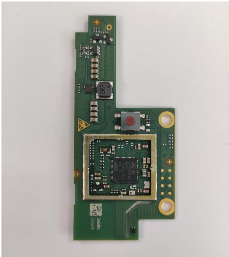
PCB bottom side without shielding
