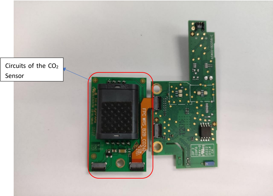
PCB top side
