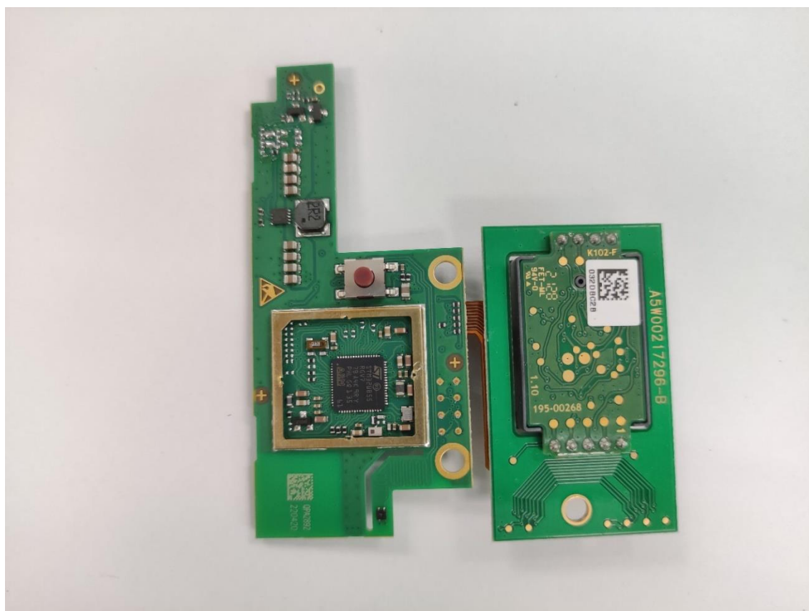
PCB bottom side without shielding
