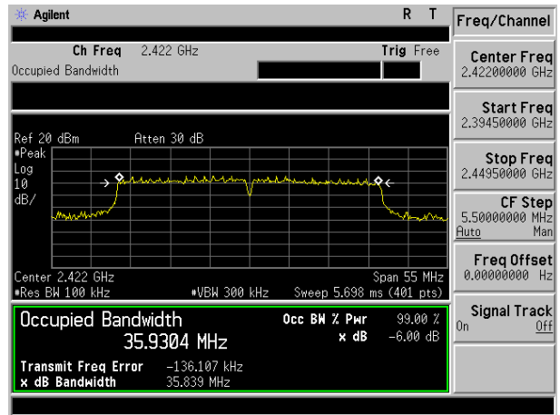
(802.11n40) channel 3
