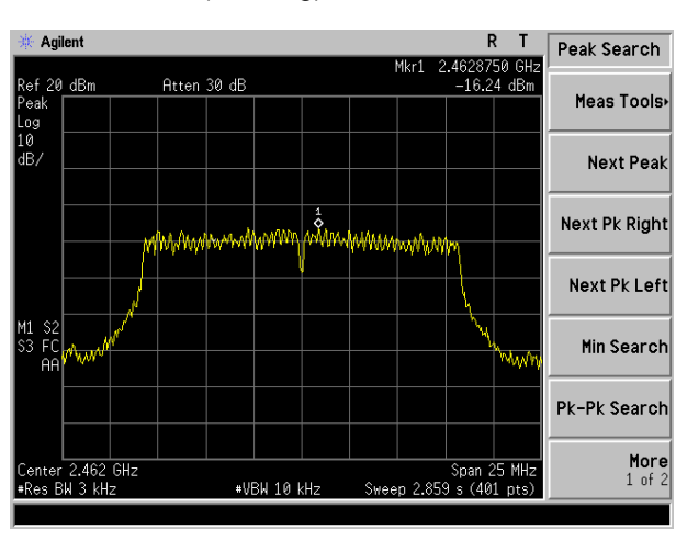
(802.11g) channel 11
