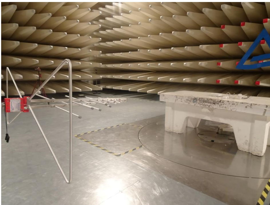
Test Setup
