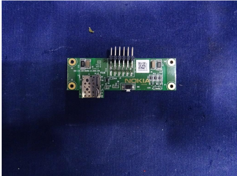
LED-SIM board
