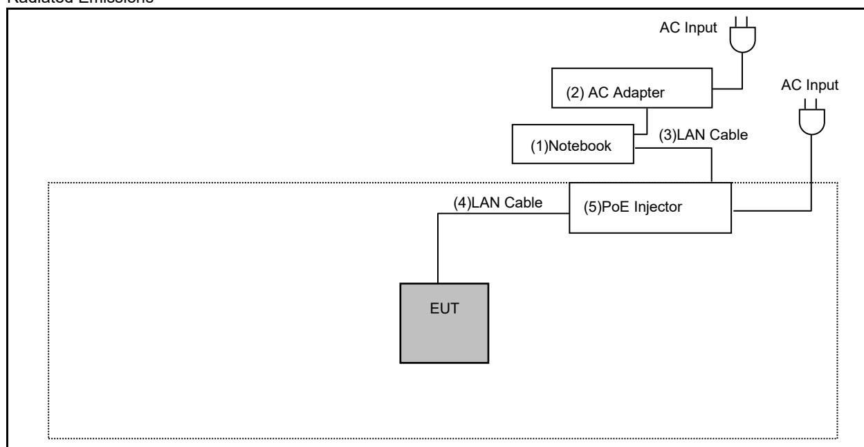
Radiated Emissions
