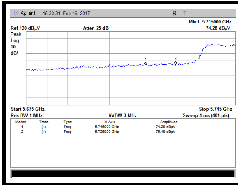
(Channel = 155 Horizontal @ 802.11ac)
