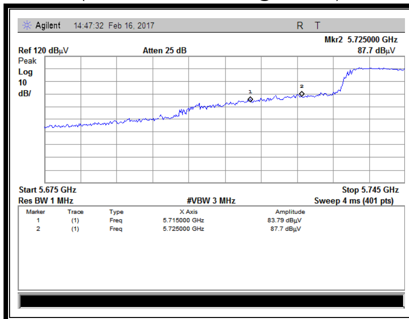
(Channel = 151 Vertical @ 802.11ac)
