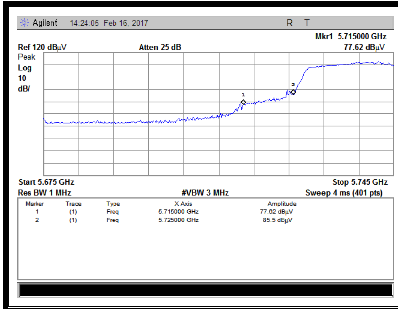
(Channel = 149 Horizontal @ 802.11ac)
