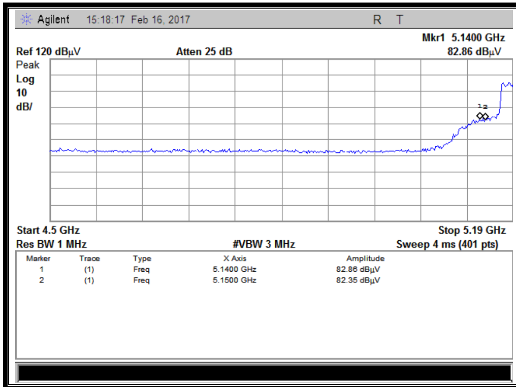
(Channel = 42 PEAK @ 802.11ac)
