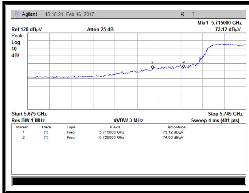
(Channel = 151 Horizontal @ 802.11ac)
