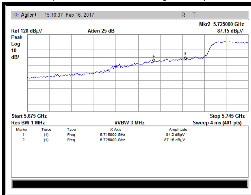
(Channel = 151 Vertical @ 802.11n)
