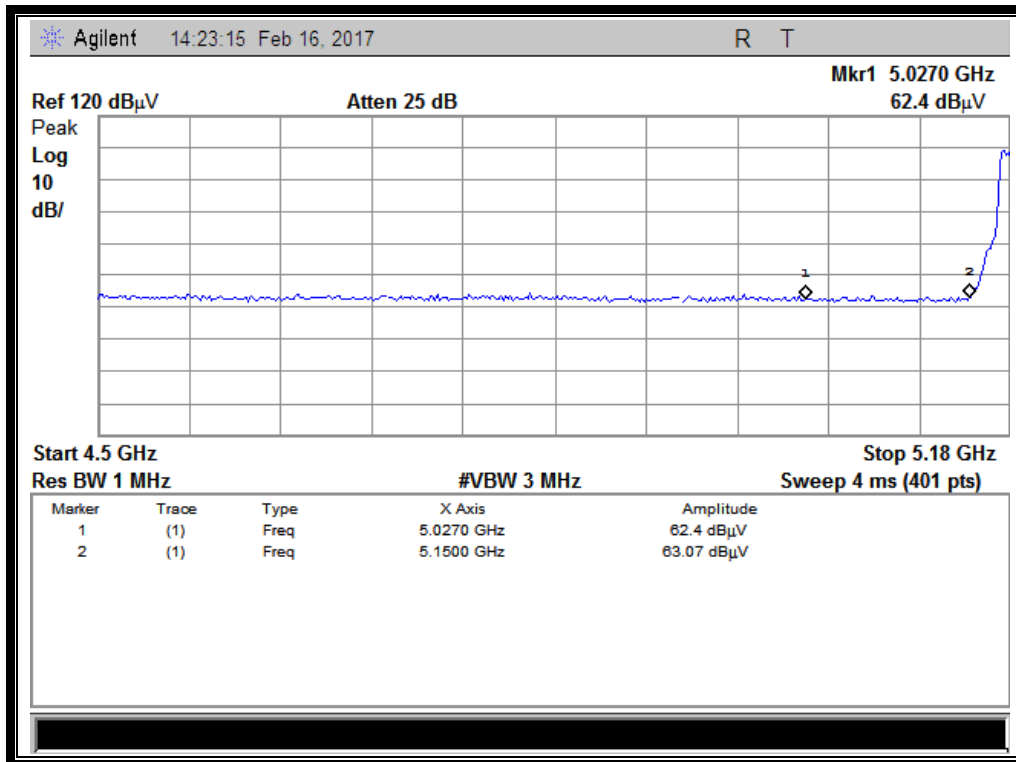
(Channel = 36 PEAK @ 802.11ac)
