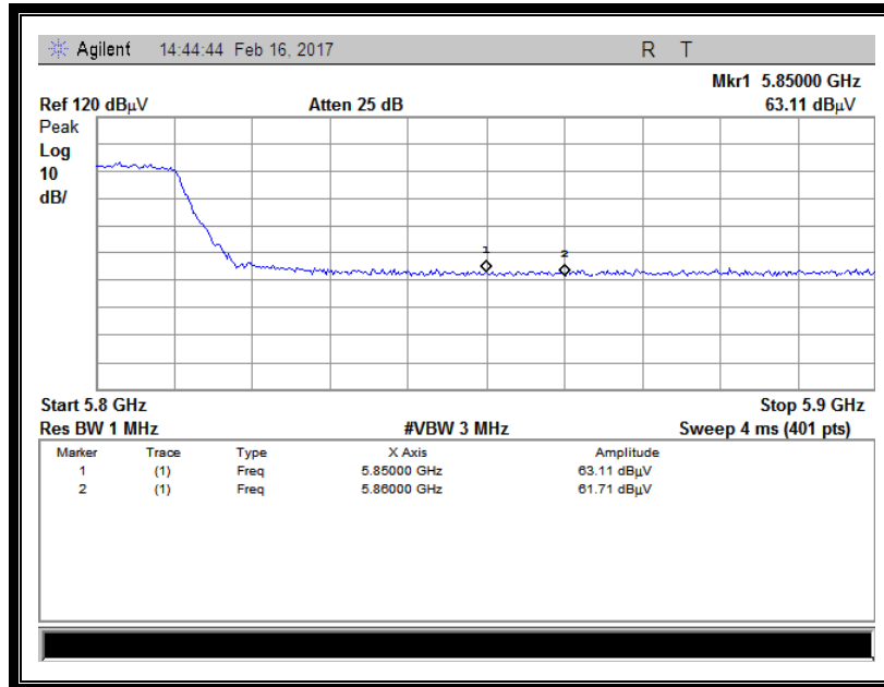
(Channel = 159 Horizontal @ 802.11ac)
