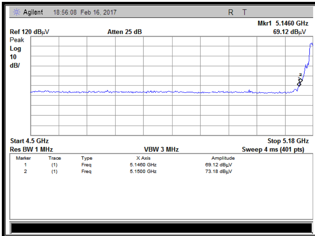
(Channel = 36 PEAK @ 802.11n-20MHz)
