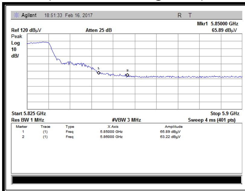
(Channel = 165 Vertical @ 802.11ac)
