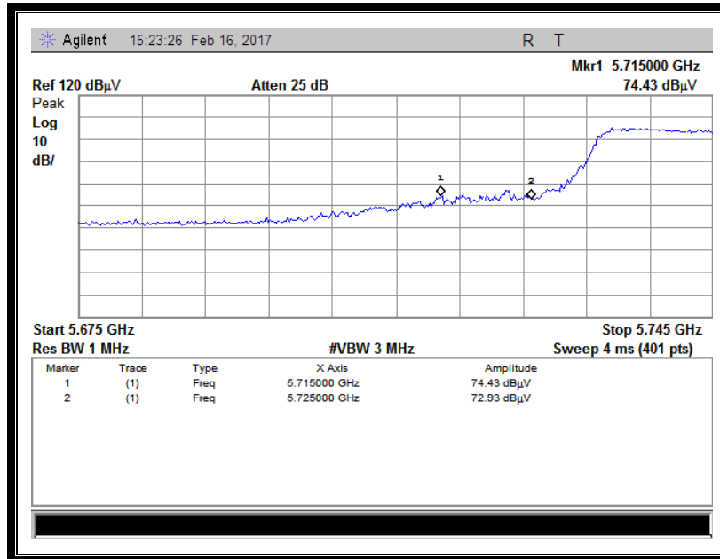
(Channel = 151 Horizontal @ 802.11n)
