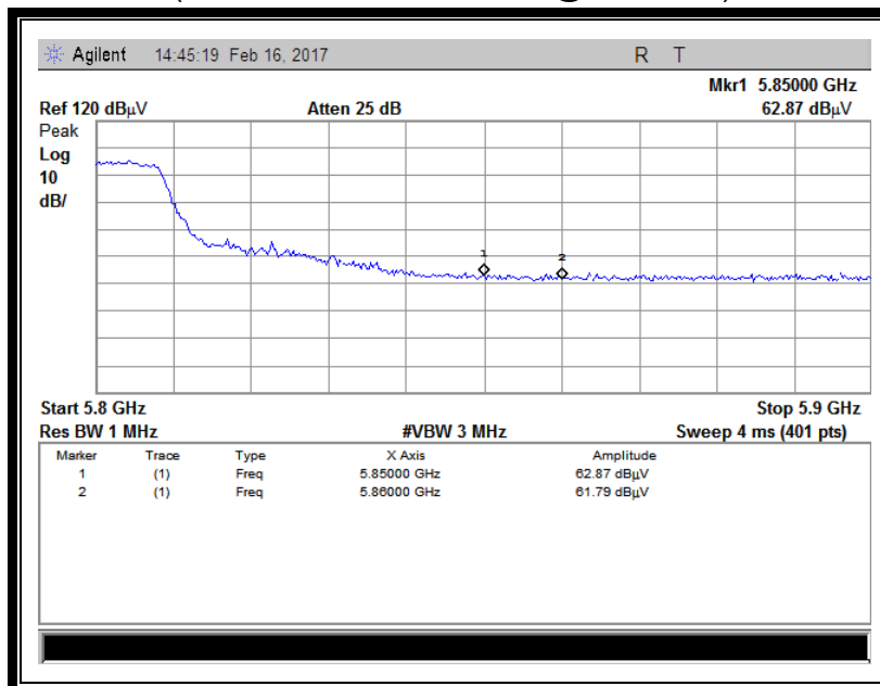
(Channel = 159 Vertical @ 802.11ac)
