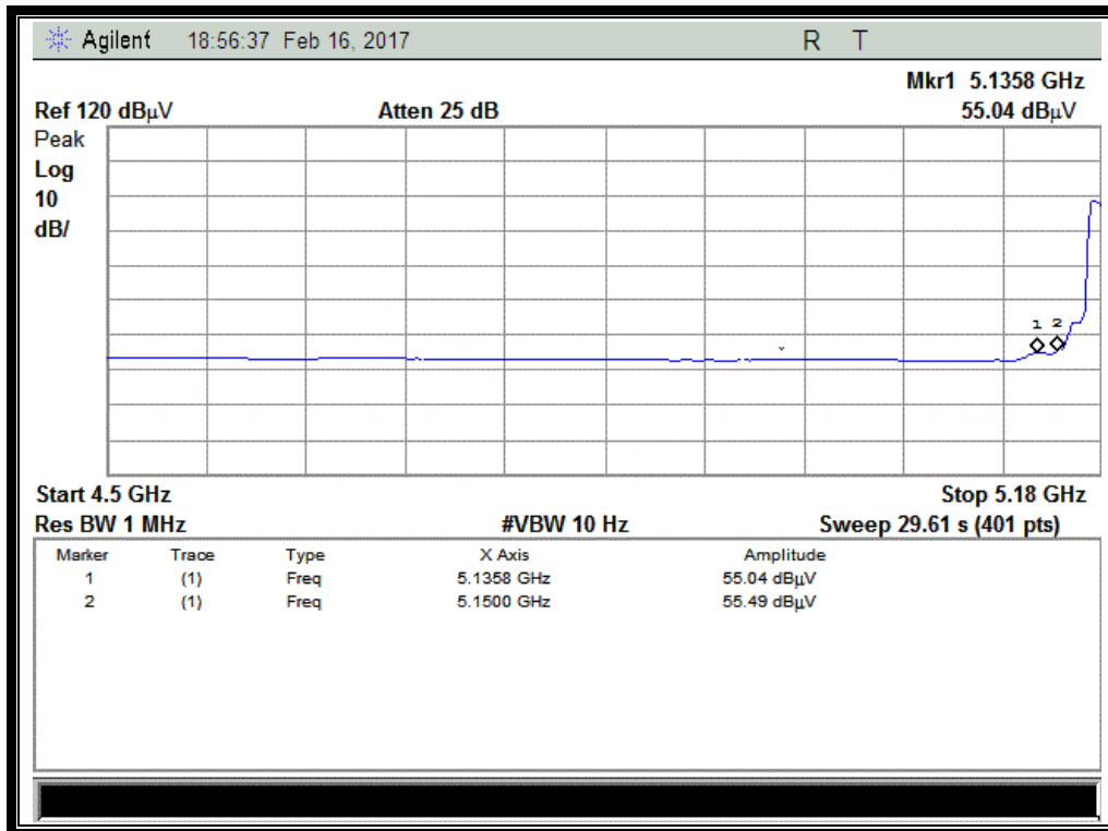
(Channel = 36 AVG @ 802.11n-20MHz)
