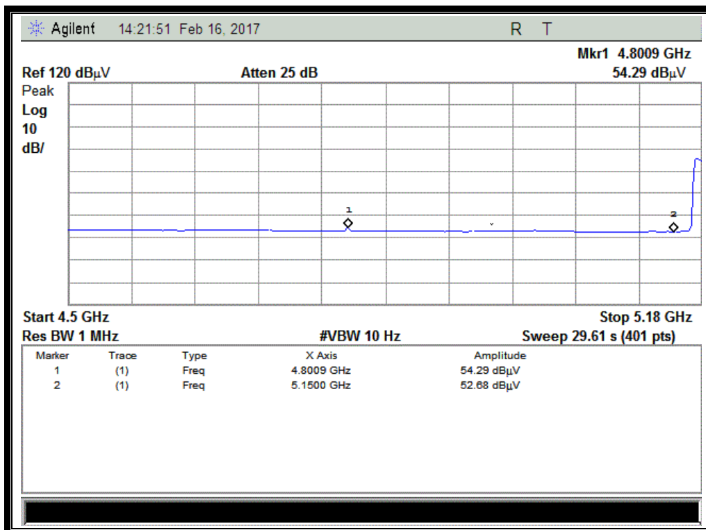
(Channel = 36 AVG @ 802.11ac)
