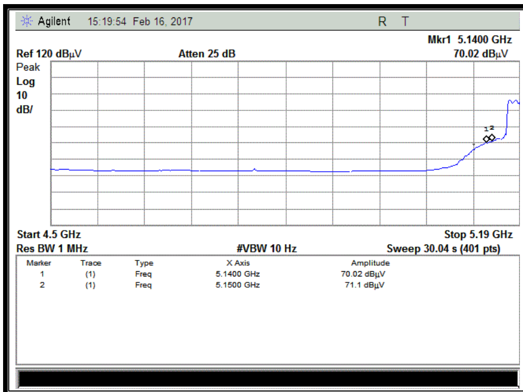
(Channel = 42 AVG @ 802.11ac)
