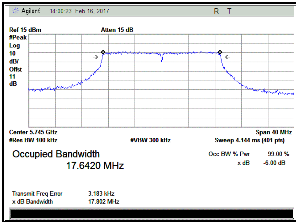
(Channel 149: 5745MHz @ 802.11ac)
