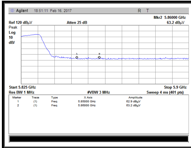
(Channel = 165 Horizontal @ 802.11ac)
