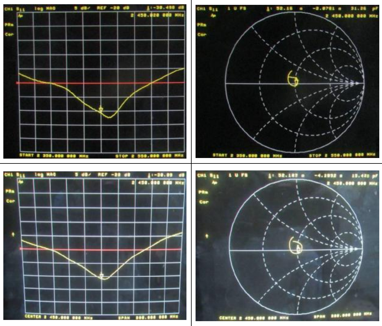
Dipole Verification Data
