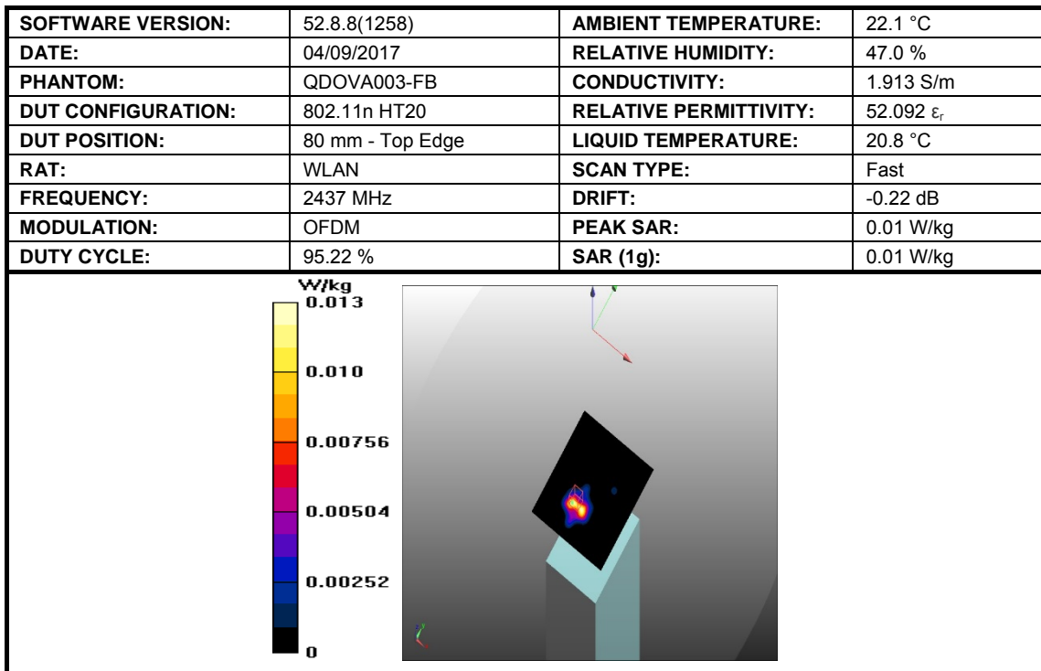
Figure 5: SAR Body Testing Results for Easy Scan:Go Bovine Scanner at 2437 MHz.
