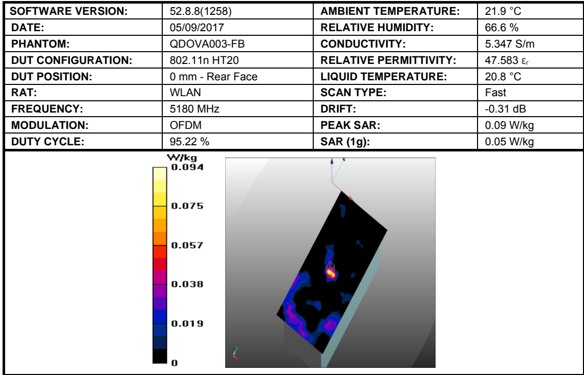
Figure 15: SAR Body Testing Results for Easy Scan:Go Bovine Scanner at 5180 MHz.
