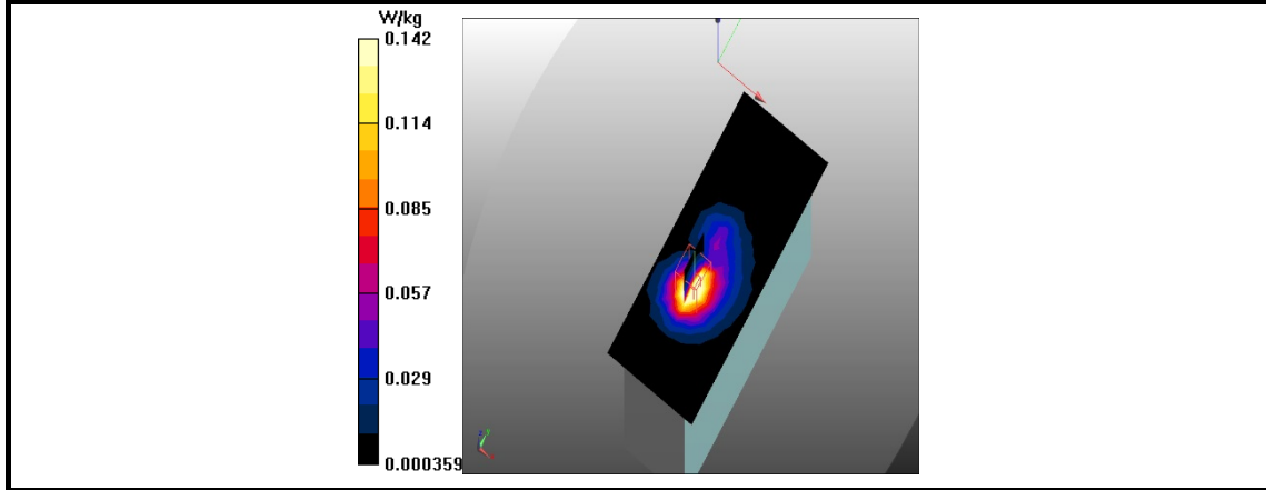
Figure 12: SAR Body Testing Results for Easy Scan:Go Bovine Scanner at 2437 MHz.
