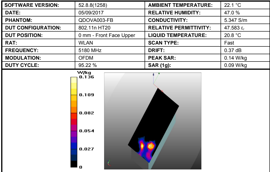
Figure 13: SAR Body Testing Results for Easy Scan:Go Bovine Scanner at 5180 MHz.
