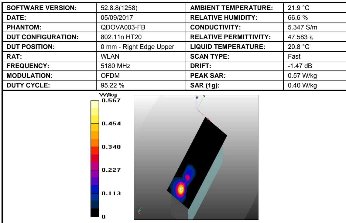
Figure 20: SAR Body Testing Results for Easy Scan:Go Bovine Scanner at 5180 MHz.
