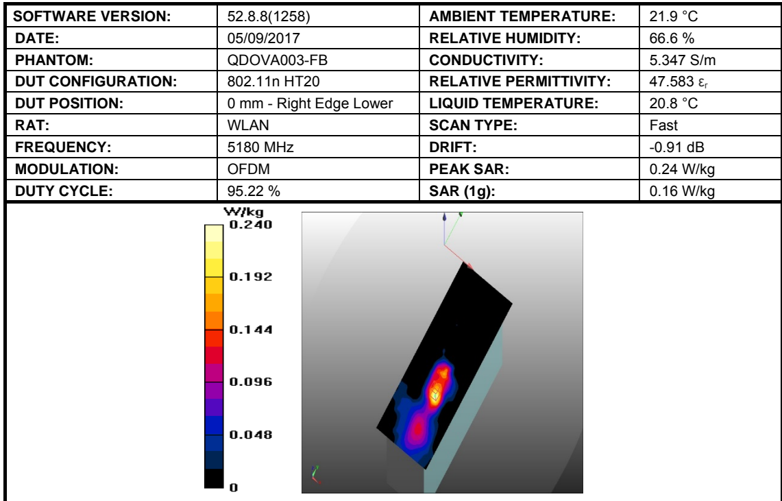
Figure 21: SAR Body Testing Results for Easy Scan:Go Bovine Scanner at 5180 MHz.
