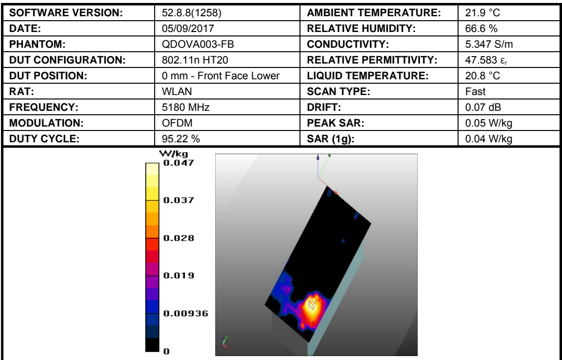
Figure 14: SAR Body Testing Results for Easy Scan:Go Bovine Scanner at 5180 MHz.
