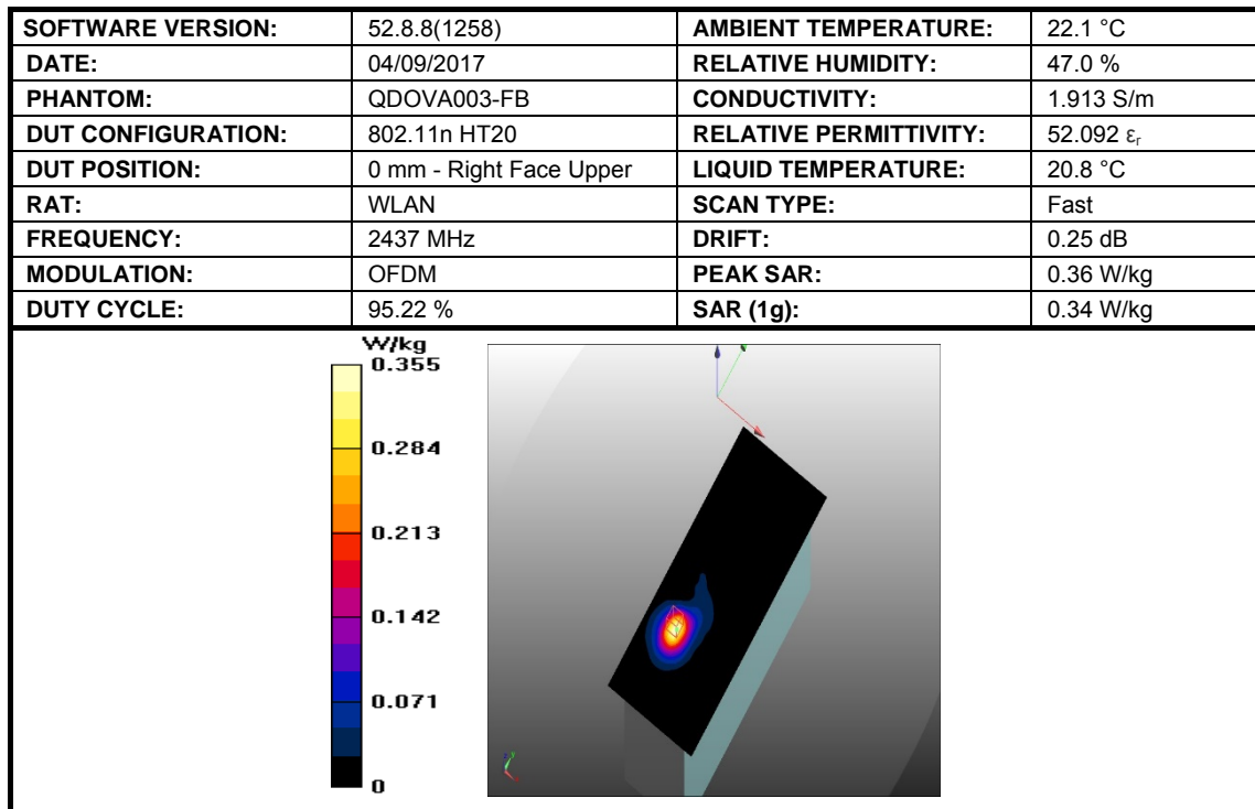
Figure 9: SAR Body Testing Results for Easy Scan:Go Bovine Scanner at 2437 MHz.
