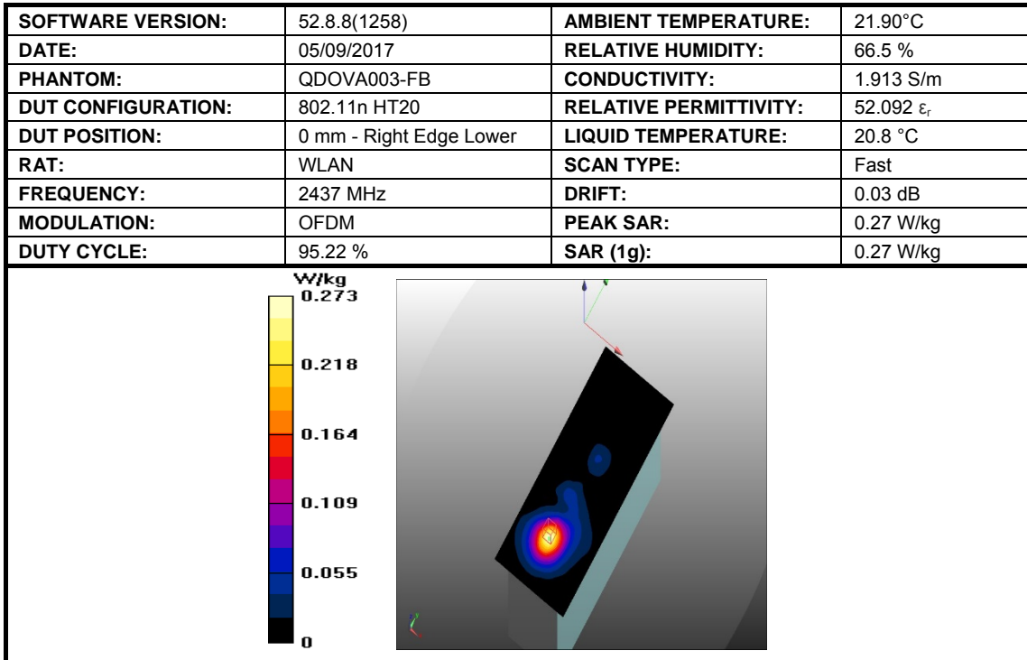
Figure 10: SAR Body Testing Results for Easy Scan:Go Bovine Scanner at 2437 MHz.
