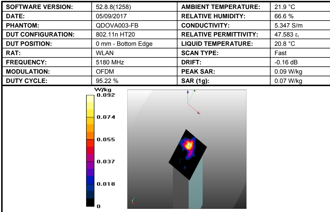
Figure 17: SAR Body Testing Results for Easy Scan:Go Bovine Scanner at 5180 MHz.
