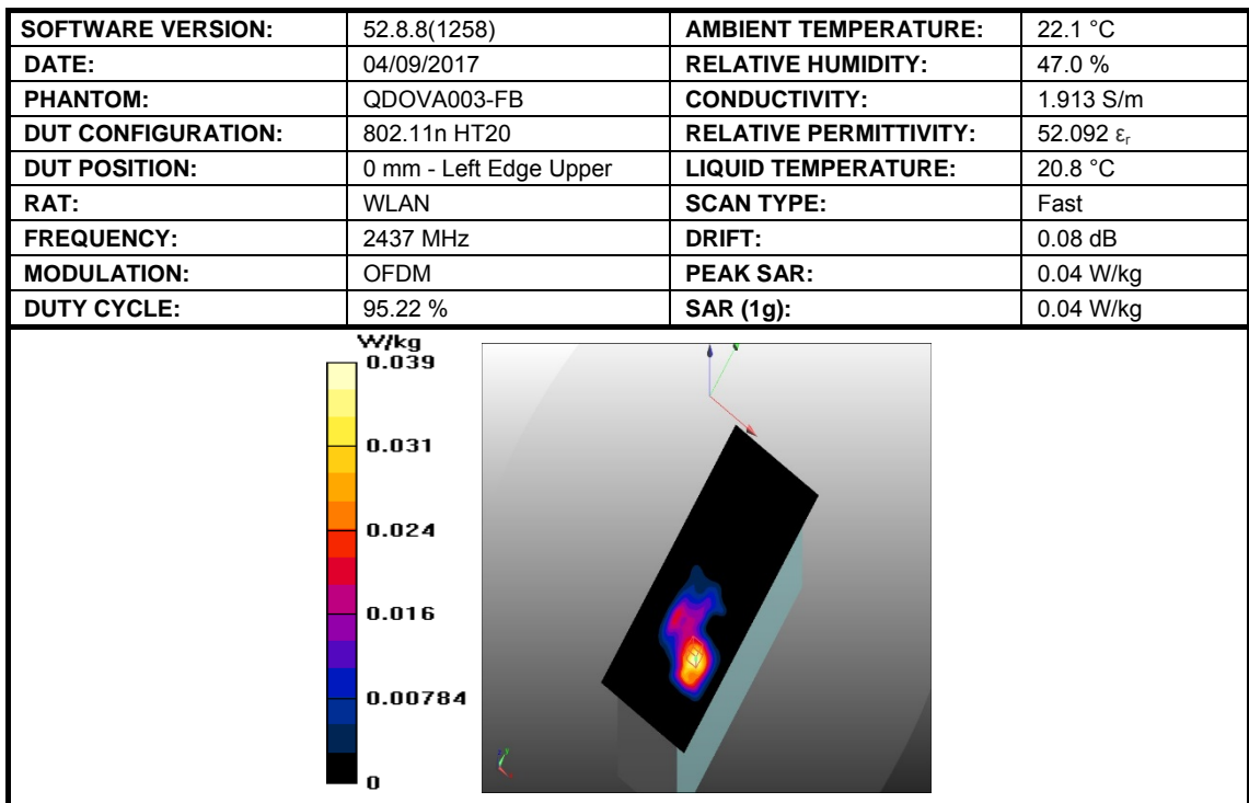
Figure 7: SAR Body Testing Results for Easy Scan:Go Bovine Scanner at 2437 MHz.
