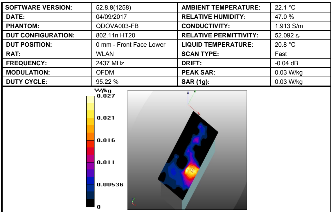
Figure 3: SAR Body Testing Results for Easy Scan:Go Bovine Scanner at 2437 MHz.
