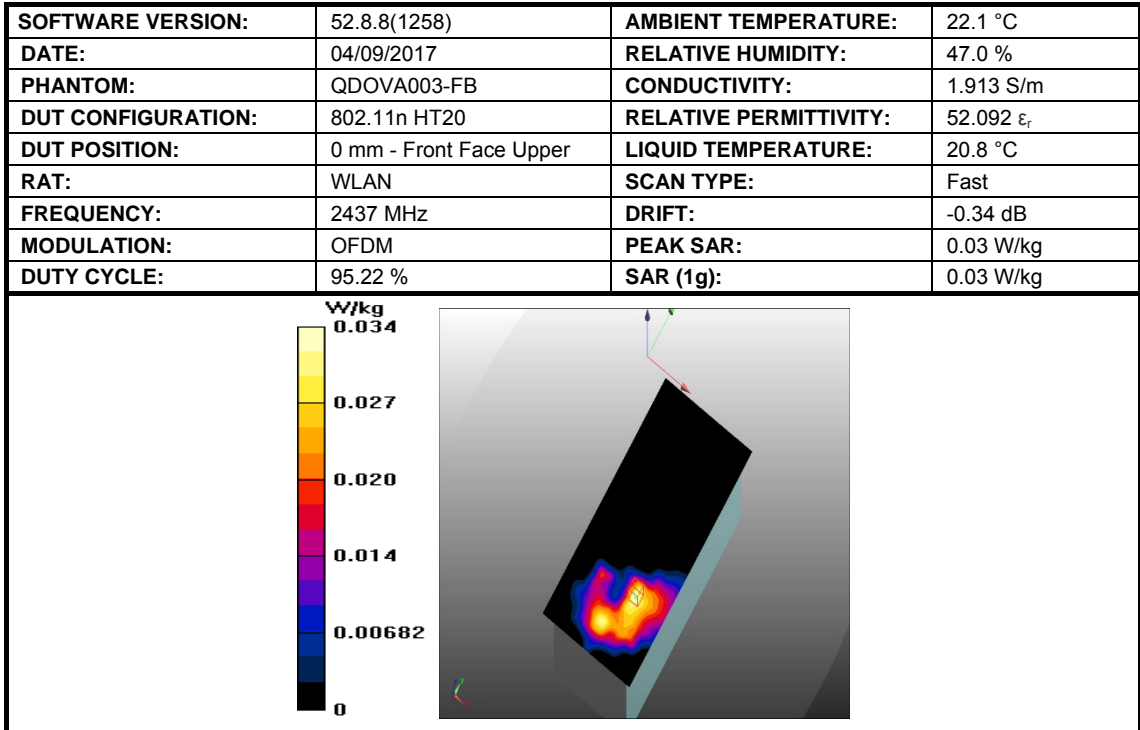
Figure 2: SAR Body Testing Results for Easy Scan:Go Bovine Scanner at 2437 MHz.
