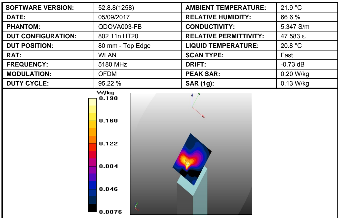
Figure 16: SAR Body Testing Results for Easy Scan:Go Bovine Scanner at 5180 MHz.
