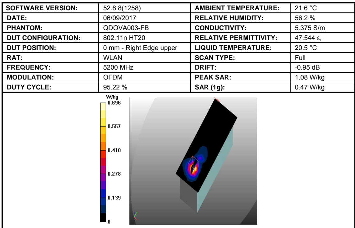
Figure 24: SAR Body Testing Results for Easy Scan:Go Bovine Scanner at 5200 MHz.
