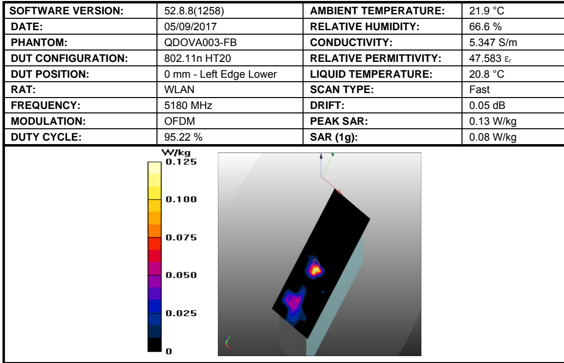
Figure 19: SAR Body Testing Results for Easy Scan:Go Bovine Scanner at 5180 MHz.
