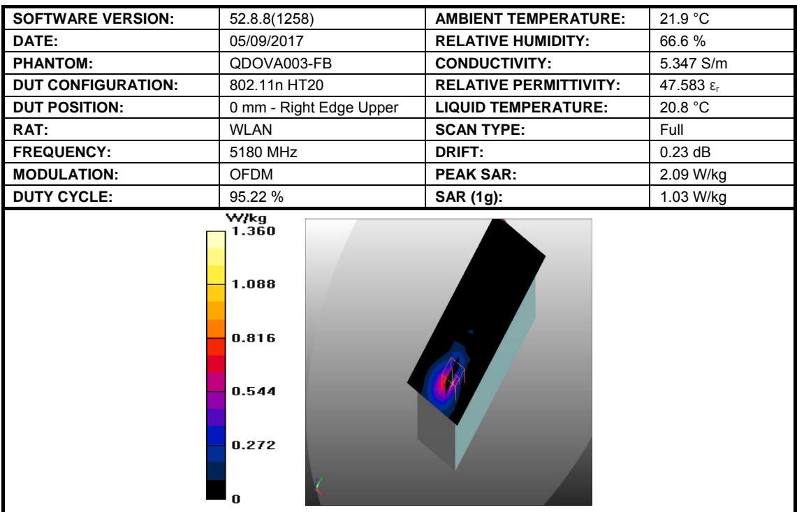
Figure 22: SAR Body Testing Results for Easy Scan:Go Bovine Scanner at 5180 MHz.
