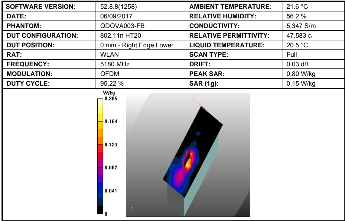
Figure 23: SAR Body Testing Results for Easy Scan:Go Bovine Scanner at 5180 MHz.
