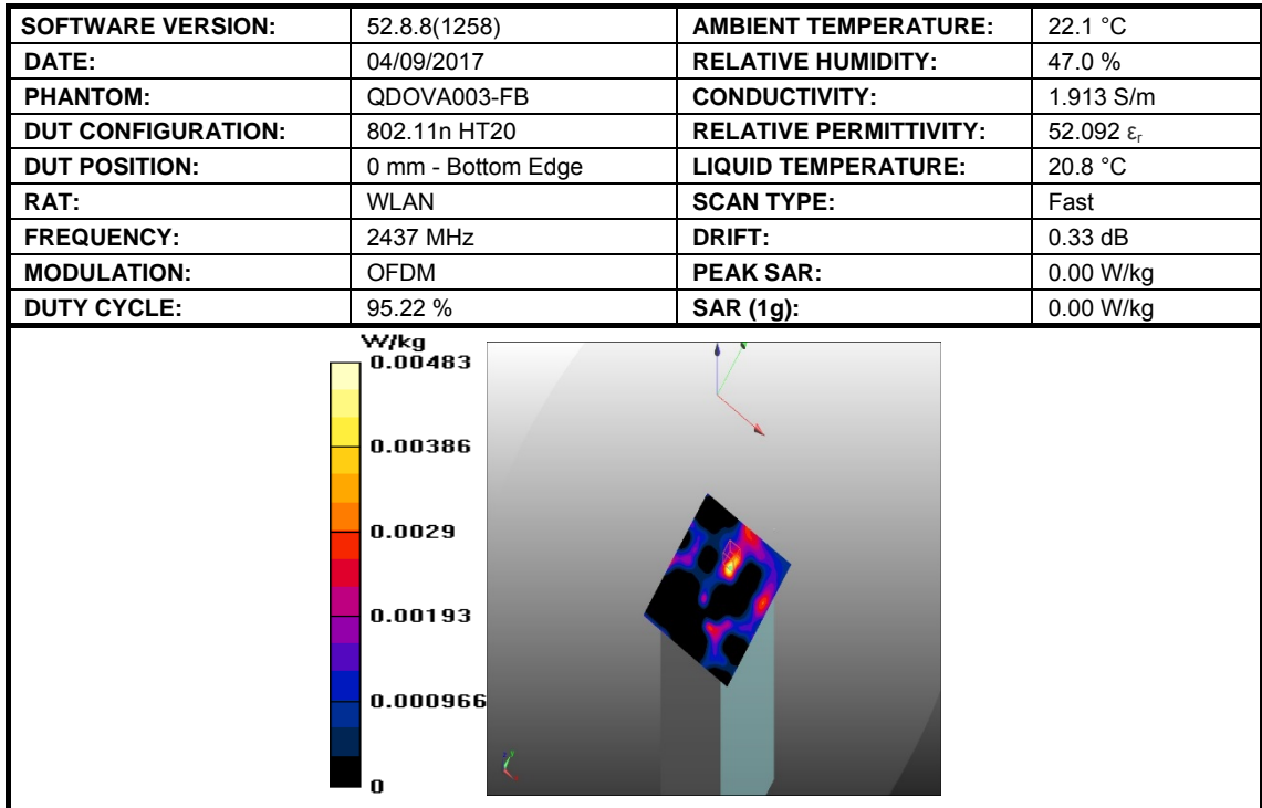
Figure 6: SAR Body Testing Results for Easy Scan:Go Bovine Scanner at 2437 MHz.
