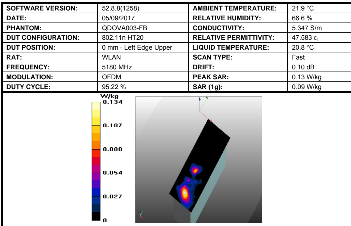
Figure 18: SAR Body Testing Results for Easy Scan:Go Bovine Scanner at 5180 MHz.
