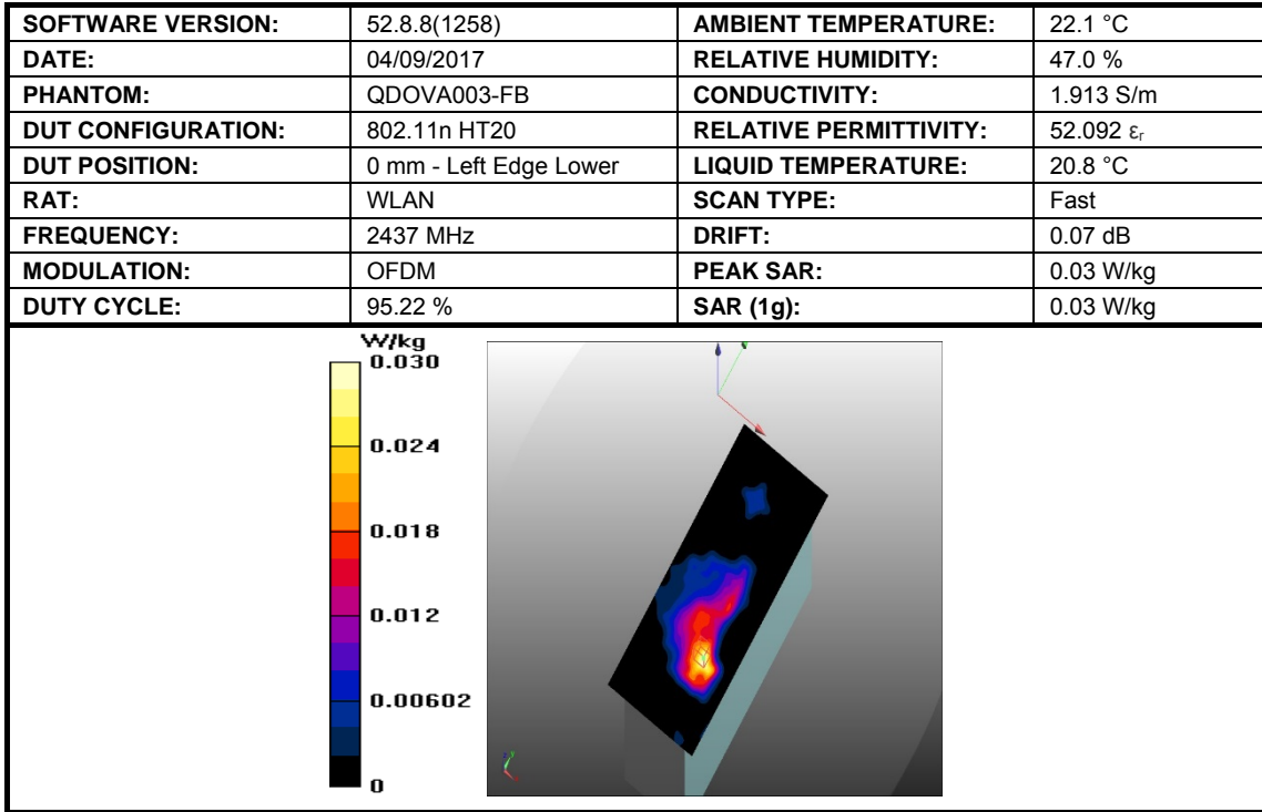
Figure 8: SAR Body Testing Results for Easy Scan:Go Bovine Scanner at 2437 MHz.
