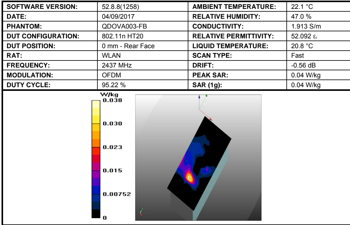
Figure 4: SAR Body Testing Results for Easy Scan:Go Bovine Scanner at 2437 MHz.
