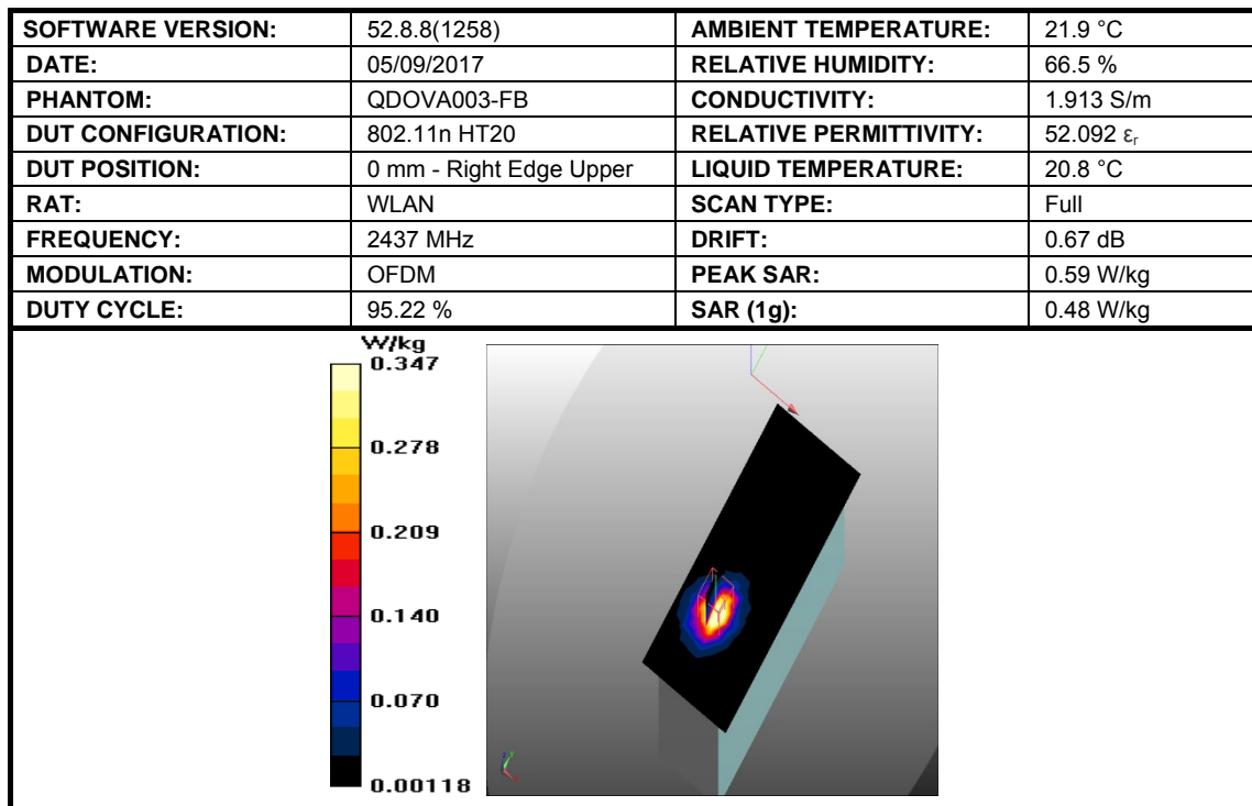
Figure 11: SAR Body Testing Results for Easy Scan:Go Bovine Scanner at 2437 MHz.
