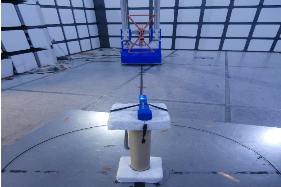
Radiated Emissions 30 MHz to 1 GHz
