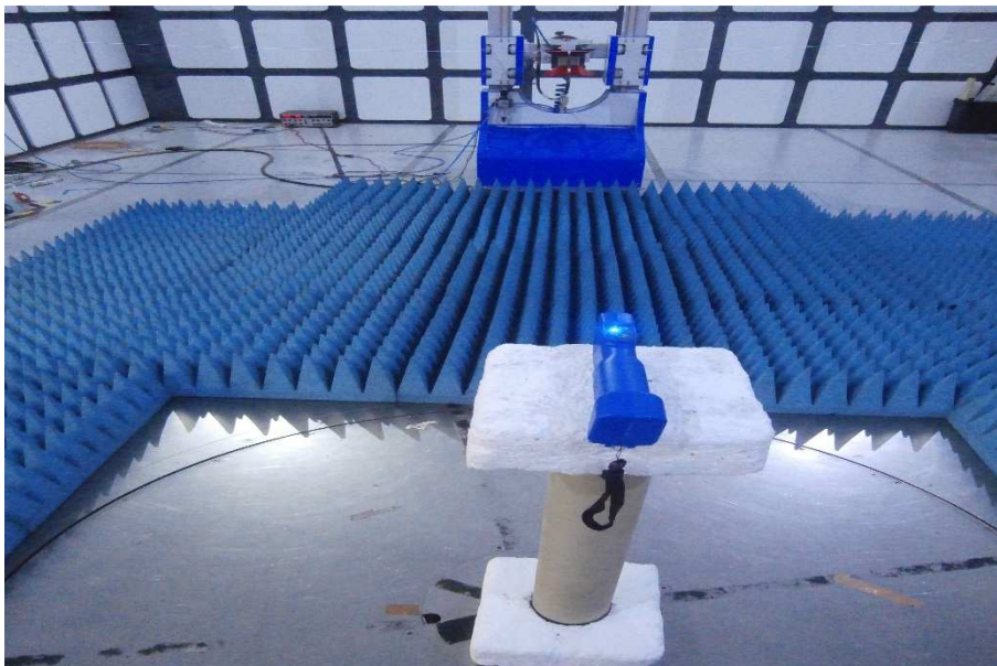
Radiated Emissions 8 GHz to 18 GHz
