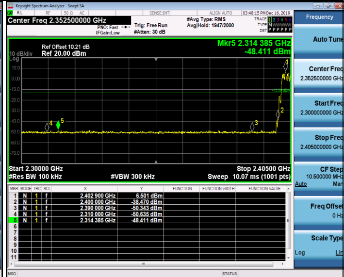
Channel 0 / 2402 MHz – Hopping
