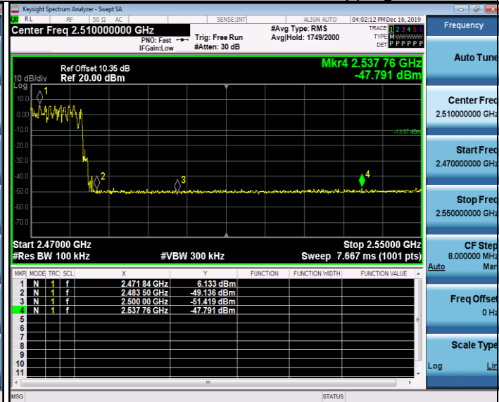
Channel 78 / 2480 MHz – Hopping
