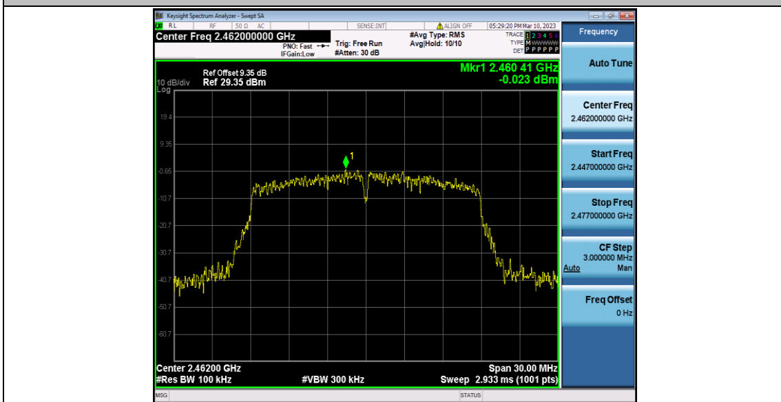
11N20SISO_Ant0_2462_0~Reference
