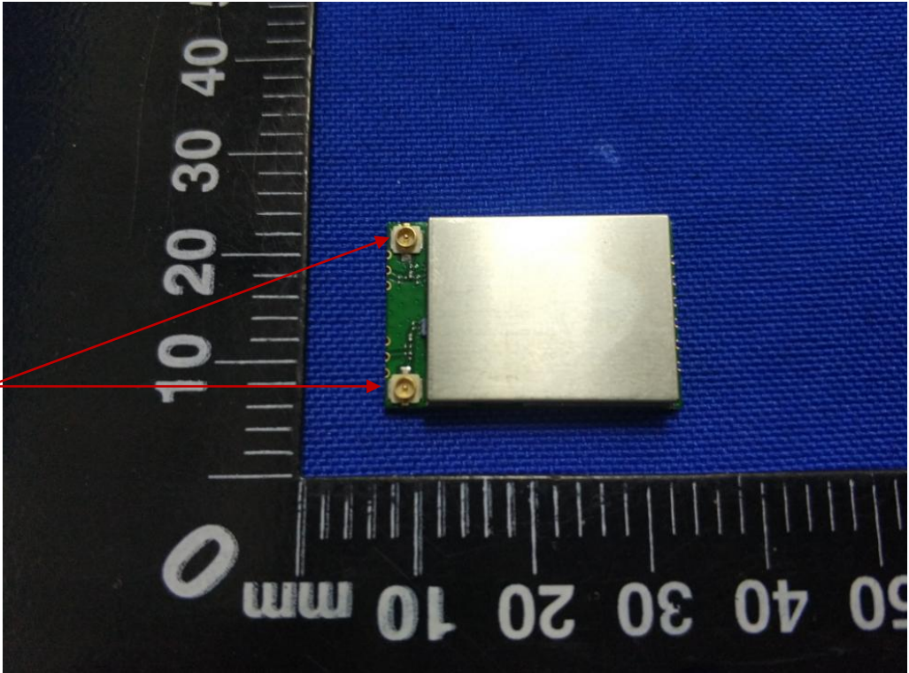
Wifi Antenna
