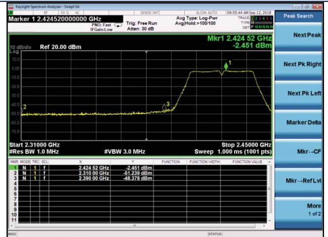
Channel 3 / 2422 MHz – Peak
