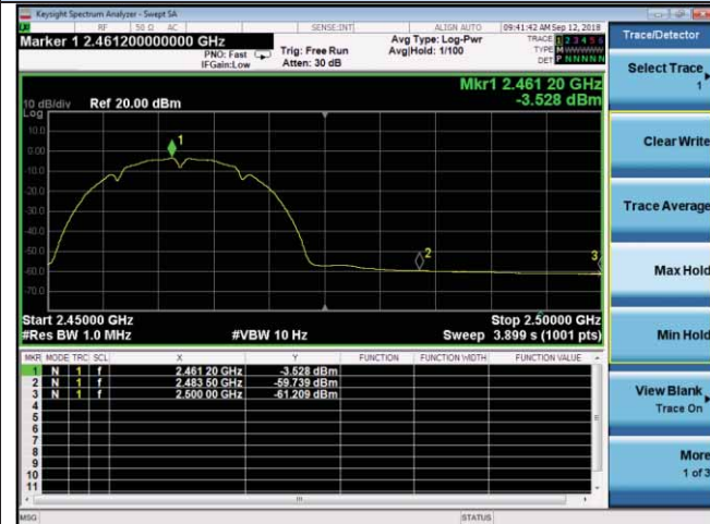
Channel 11 / 2462 MHz – Average IEEE 802.11n HT20
