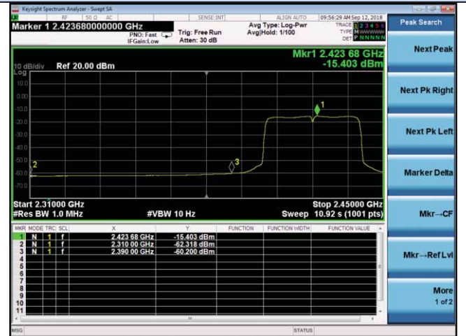
Channel 3 / 2422 MHz – Average
