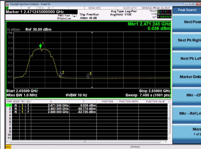
Channel 11 / 2462 MHz – Average IEEE 802.11n HT20
