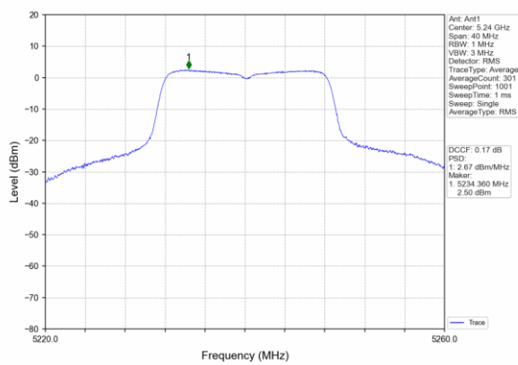
(802.11a20) PSD plot on channel 48 5240MHz
