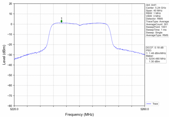
(802.11ac20) PSD plot on channel 48 5240MHz
