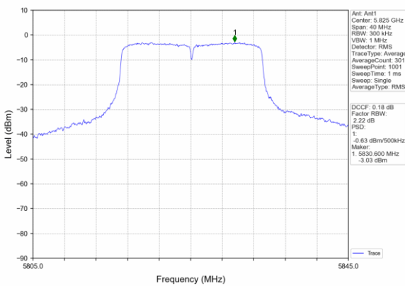
(802.11ac20) PSD plot on channel 165 5825MHz
