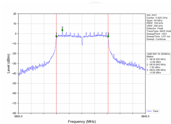
(802.11a20) 6dB Bandwidth plot on channel 165
