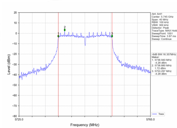
(802.11a20) 6dB Bandwidth plot on channel 149
