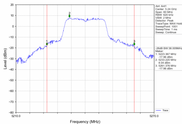
(802.11 n20) 26dB Bandwidth plot on channel 48
