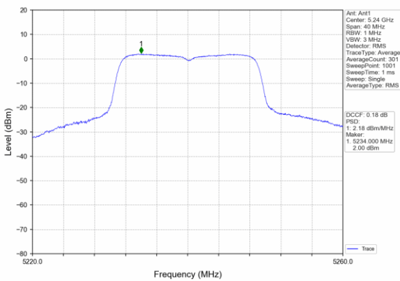
(802.11n20) PSD plot on channel 48 5240MHz
