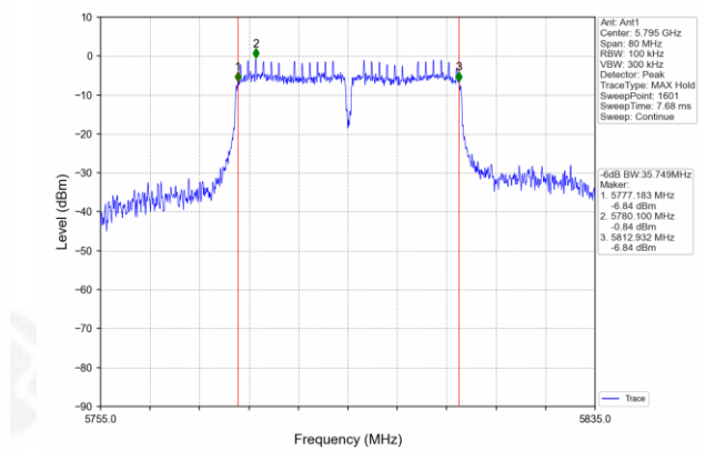
(802.11 n40) 6dB Bandwidth plot on channel 159
