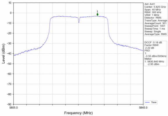
(802.11n20) PSD plot on channel 165 5825MHz
