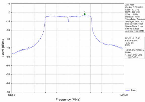
(802.11a20) PSD plot on channel 165 5825MHz
