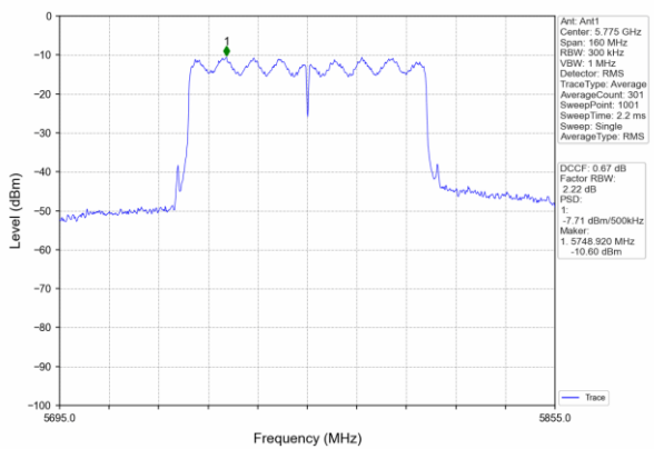
(802.11ac80) PSD plot on channel 155 5775MHz
