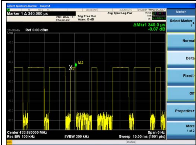
Duty Cycle 3#
