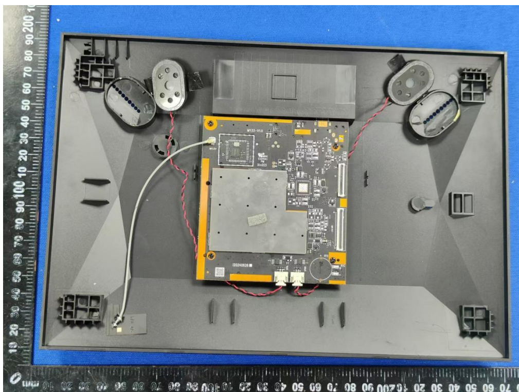
Internal view of unit(Model:USAFDPF10BK)
