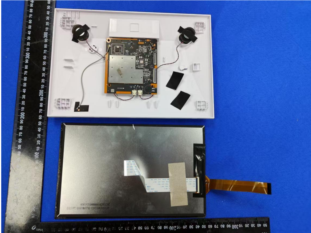
Internal view of unit(Model: USAFDPF10BW)
