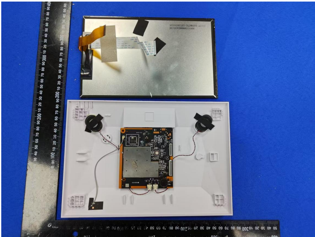
Internal view of unit(Model: AFDPF10BW)
