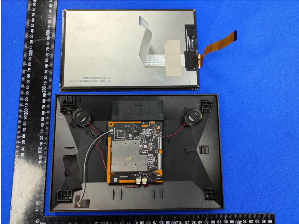
Internal view of unit(Model:AFDPF10BK)
