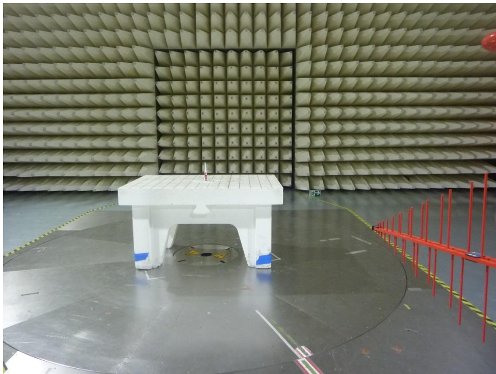
Figure 1: Test Setup for Radiated Emissions 30MHz to 1000MHz
