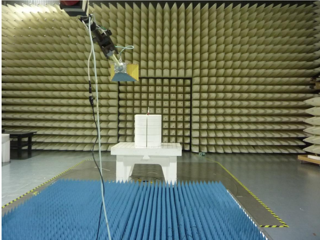
Figure 2: Test Setup for Radiated Emissions 1GHz to 18GHz
