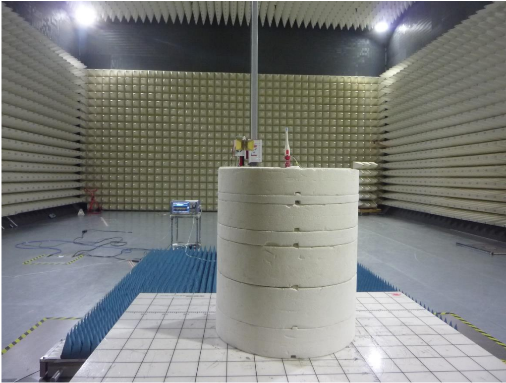
Figure 3: Test Setup for Radiated Emissions 1GHz to 18GHz
