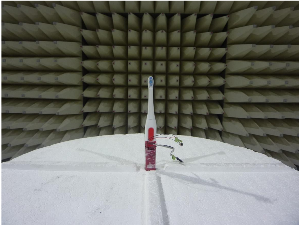
Figure 4: EUT (Z-Axis)
