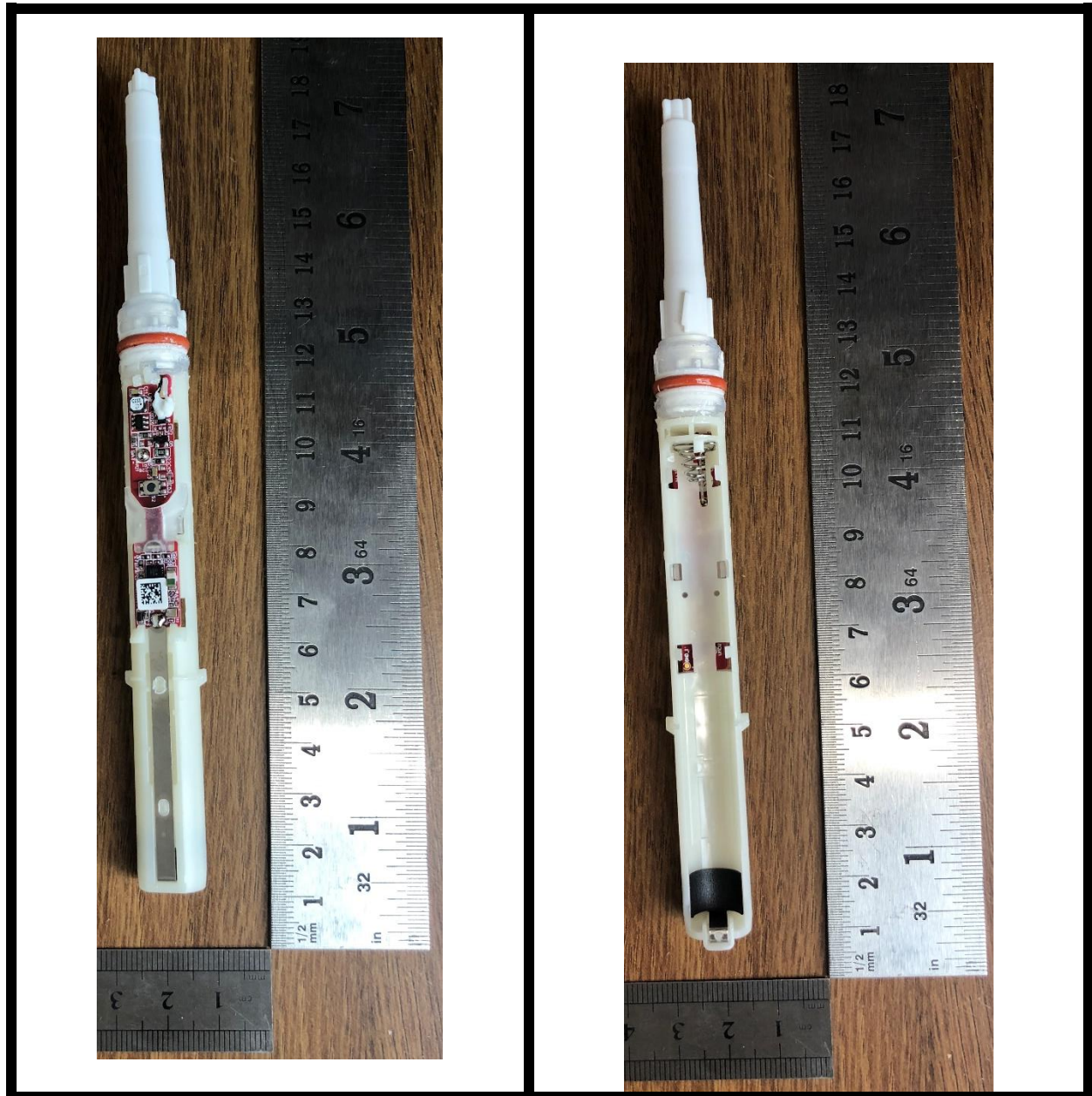
Internal Front
