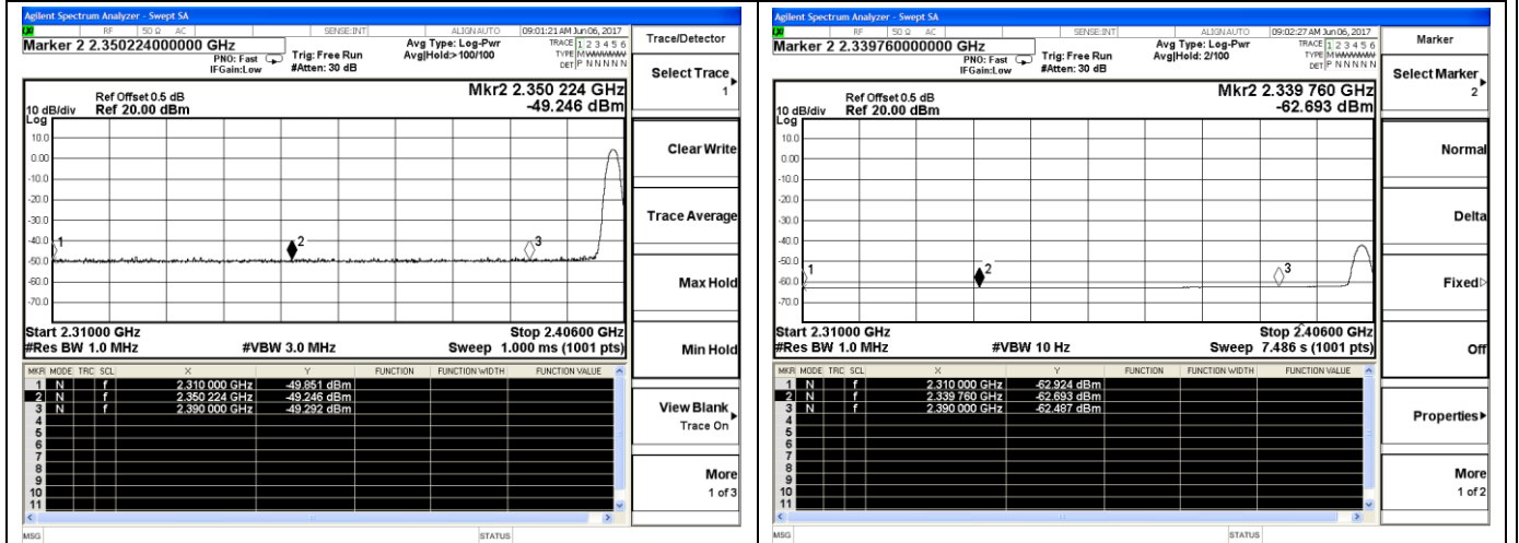
Low Channel / 2404MHz - Peak
