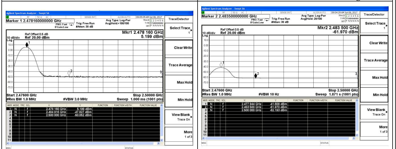
High Channel / 2478MHz - Peak
