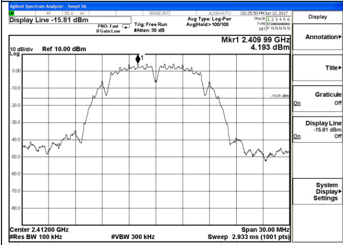
802.11b Low channel Reference
