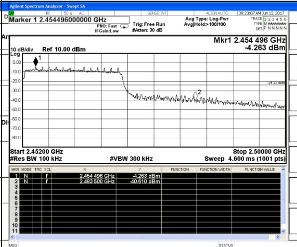
802.11n(HT40)-High channel
