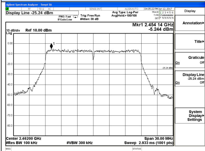
802.11n-HT20 High channel Reference
