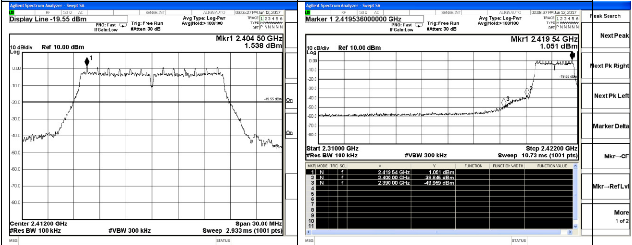
802.11g - Low channel Reference
