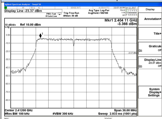
802.11n-HT20 Low channel Reference
