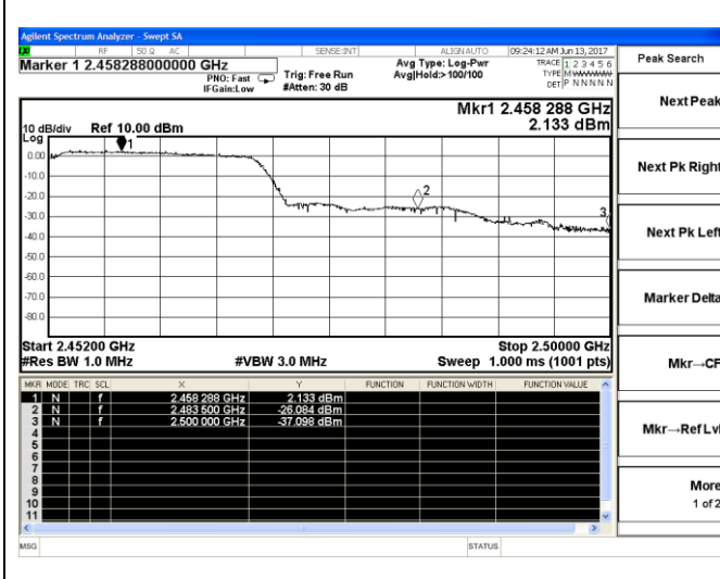
802.11n-HT40 High channel(Peak)
