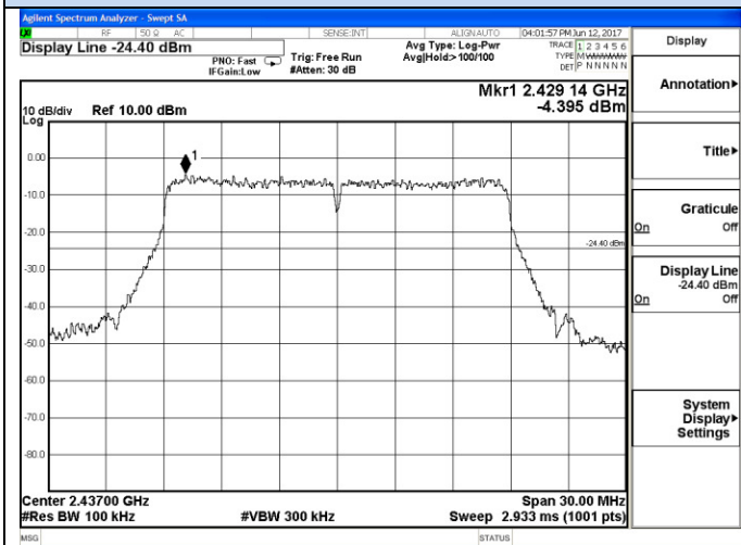
802.11n-HT20 Middle channel Reference
