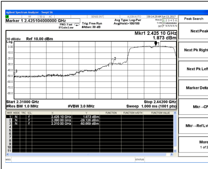
802.11n-HT40 Low channel(Peak)
