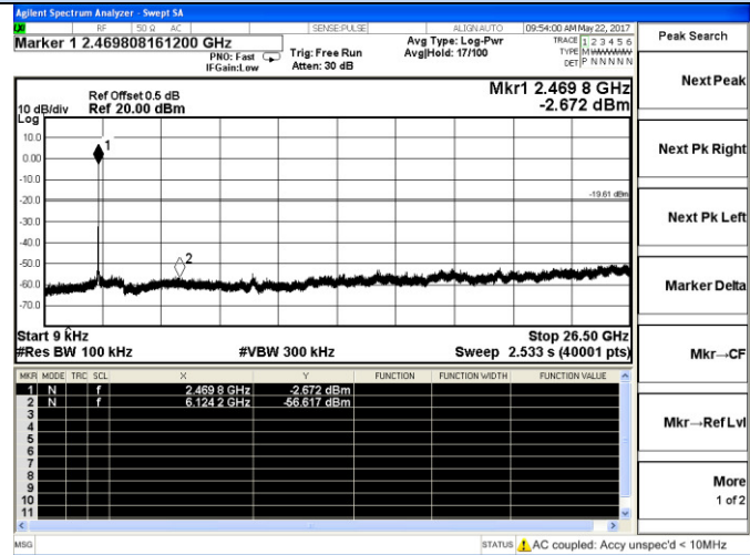
9 KHz – 26.5 GHz
