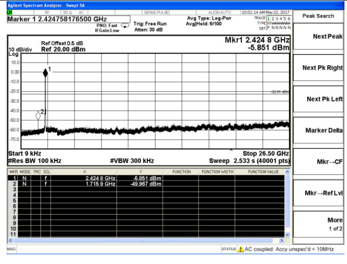
9 KHz – 26.5 GHz
