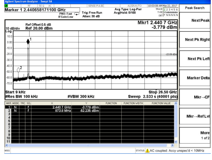
9 KHz – 26.5 GHz
