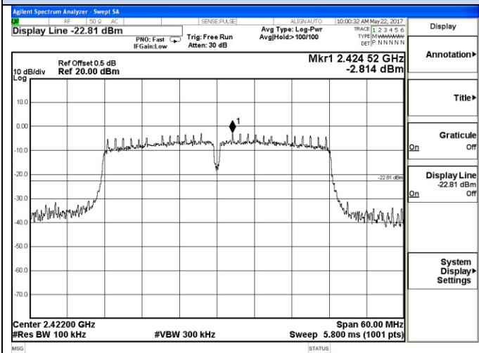
2392 – 2452 MHz
