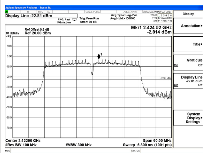
2392 – 2452 MHz
