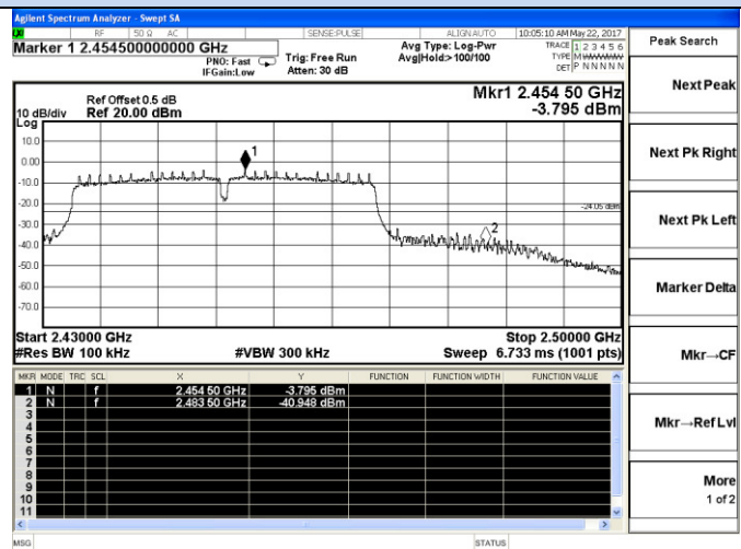
Channel 9 / 2452 MHz
