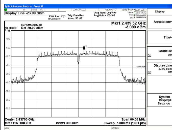
2407 – 2467 MHz
