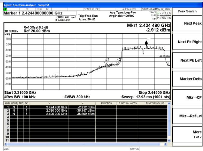
Channel 3 / 2422 MHz
