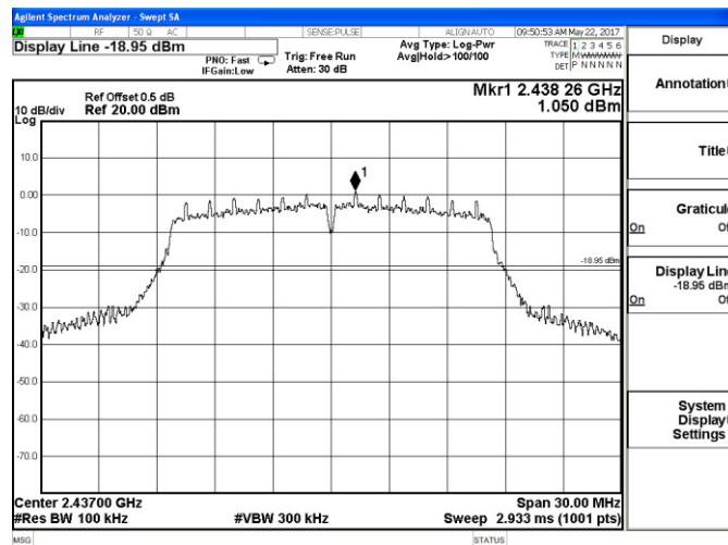
Channel 6 / 2437 MHz
