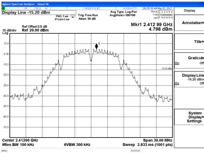
Channel 1 / 2412 MHz
