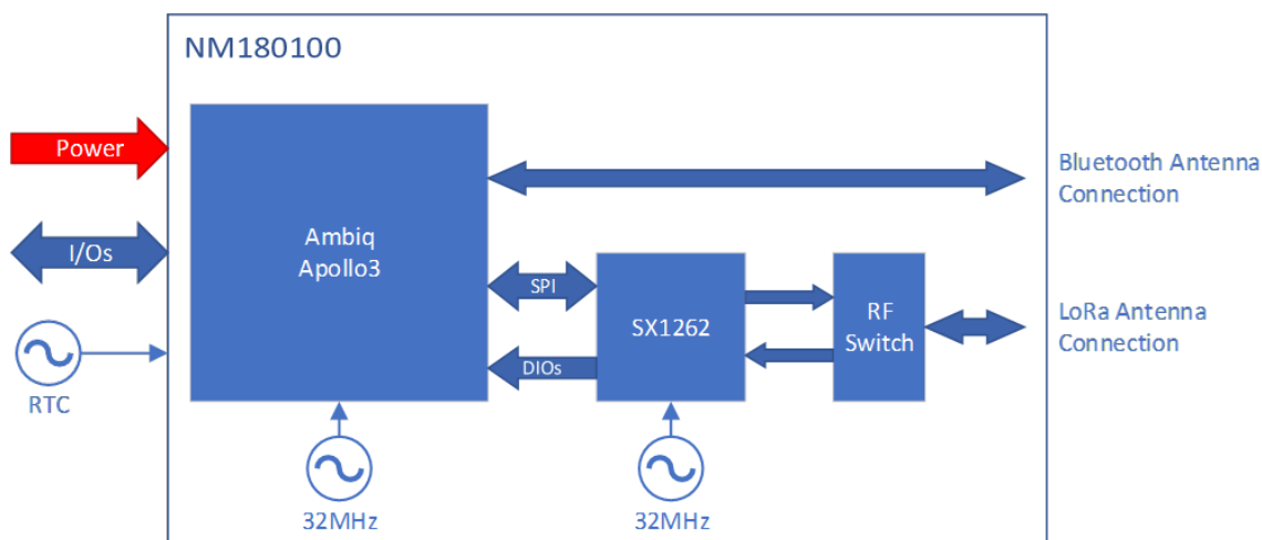
Figure 1 NM module block diagram
