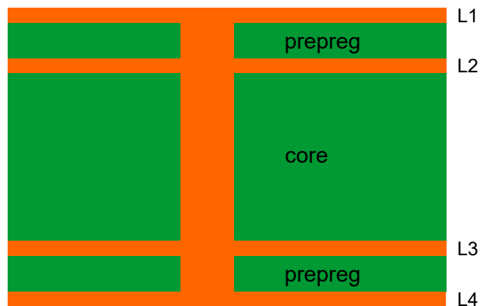
Figure 3 PCB stack-up used in the evaluation board.
