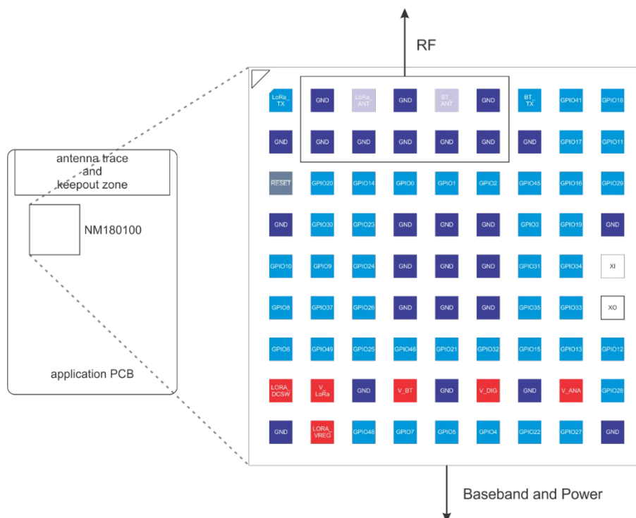
Figure 4 NM180100 placement and signal routing guidelines
