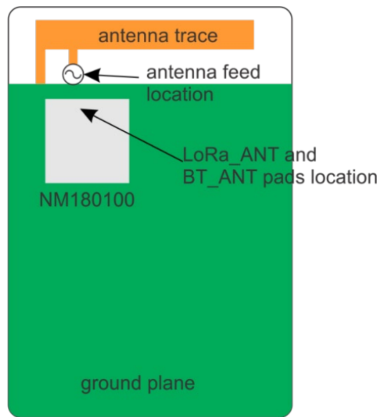
Figure 5 Antenna feed point and the relative placement of the NM180100.
