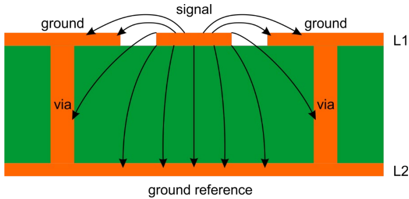
Figure 7 Grounded co-planar wave guide with via stitching and the electric field distribution.
