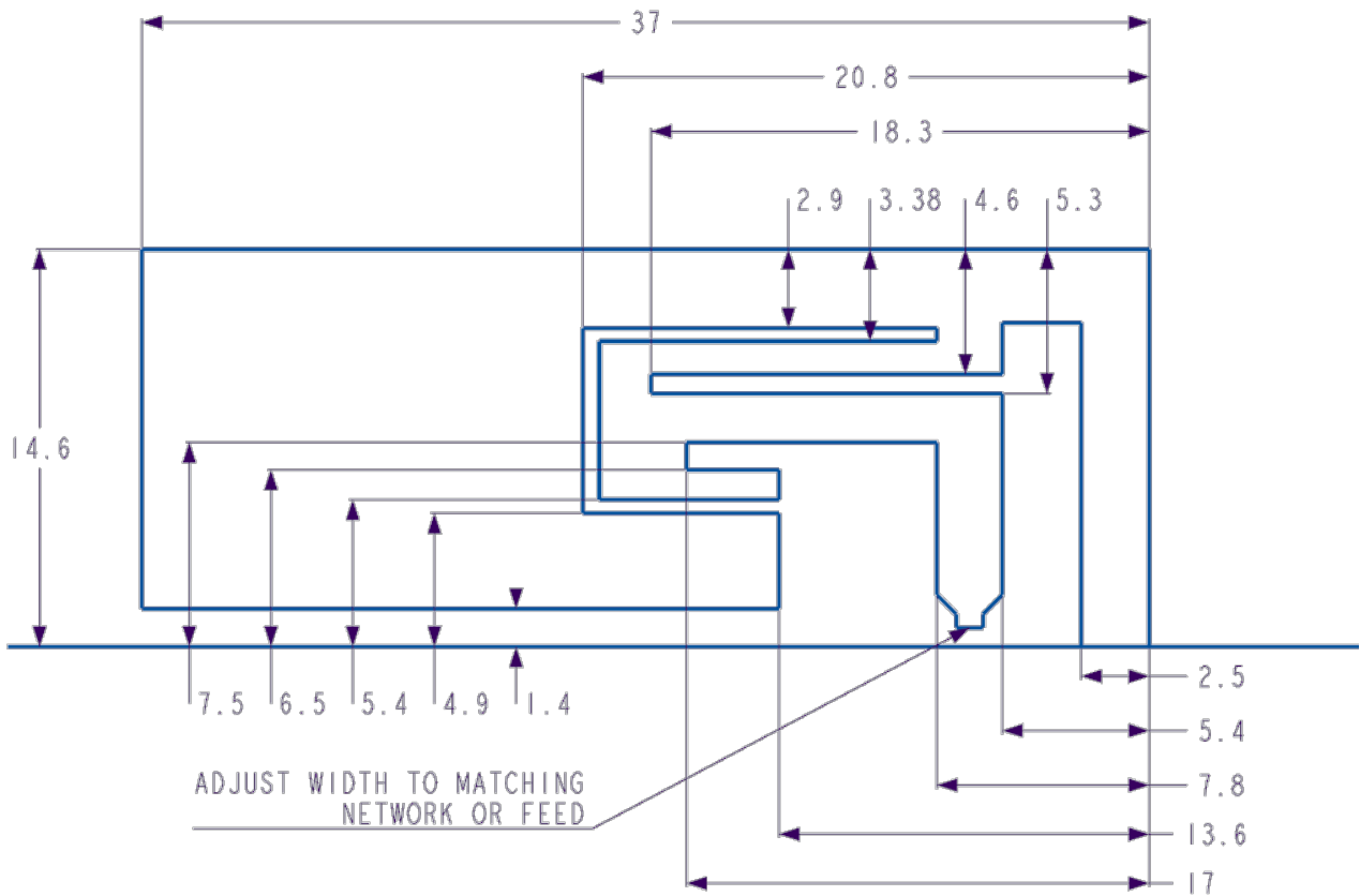
Figure 8 Reference antenna dimensions. Units are in mm unless otherwise stated.
