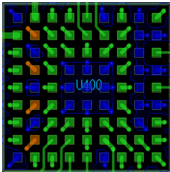
Figure 2 NM180100 fanout in the evaluation board.
