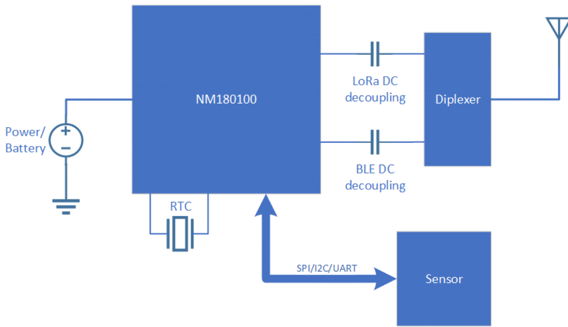
Figure 6 An example IoT sensor application implementation.
