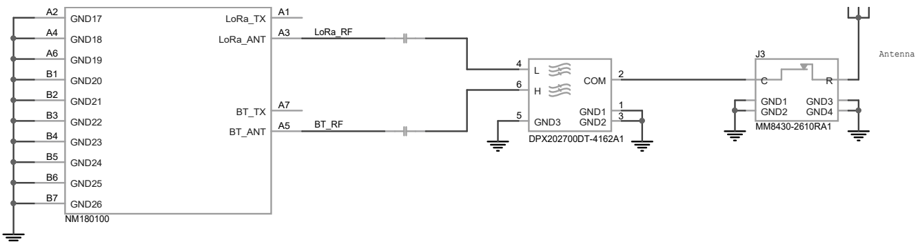
Figure 10 Single antenna switched RF coaxial connector (J3) placement.
