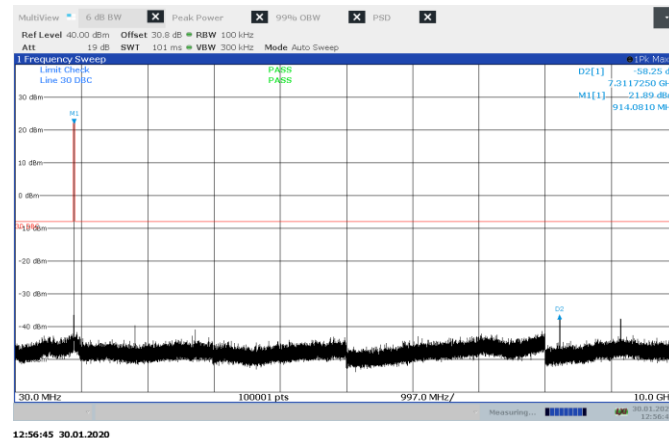
Figure 8.8-19: Conducted spurious emissions on high channel, 500 kHz BW
