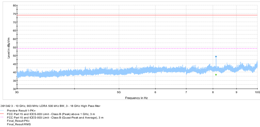
Figure 8.8-26: Radiated spurious emissions 3 – 10 GHz, 903 MHz LoRa 500 kHz BW
