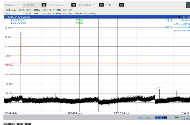
Figure 8.8-5: Conducted spurious emissions on high channel, 125 kHz BW
