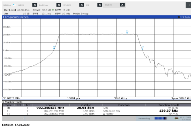
Figure 8.5-1: 20 dB bandwidth on low channel, 125 kHz BW
