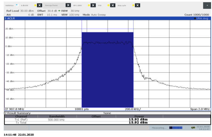
Figure 8.7-7: Output power on mid channel, 500 kHz BW
