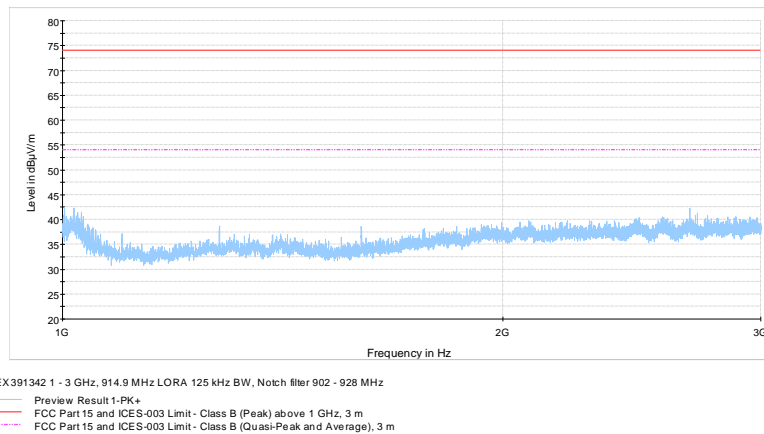
Figure 8.8-11: Radiated spurious emissions 1 - 3 GHz, 914.9 MHz LoRa 125 kHz BW
