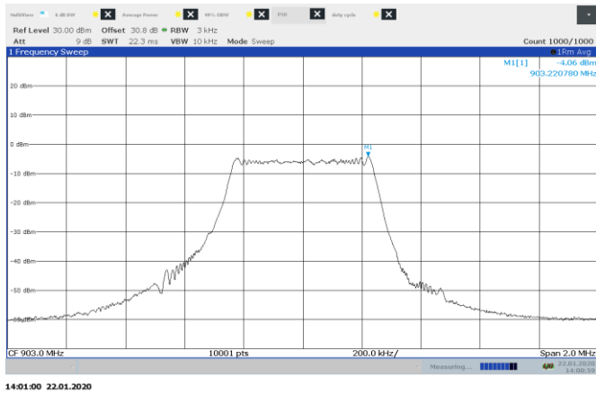
Figure 8.9-4: PSD on low channel, 500 kHz BW
