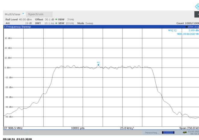
Figure 8.9-2: PSD on mid channel, 125 kHz BW
