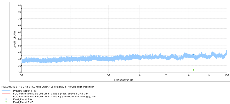
Figure 8.8-14: Radiated spurious emissions 3 - 10 GHz, 914.9 MHz LoRa 125 kHz BW
