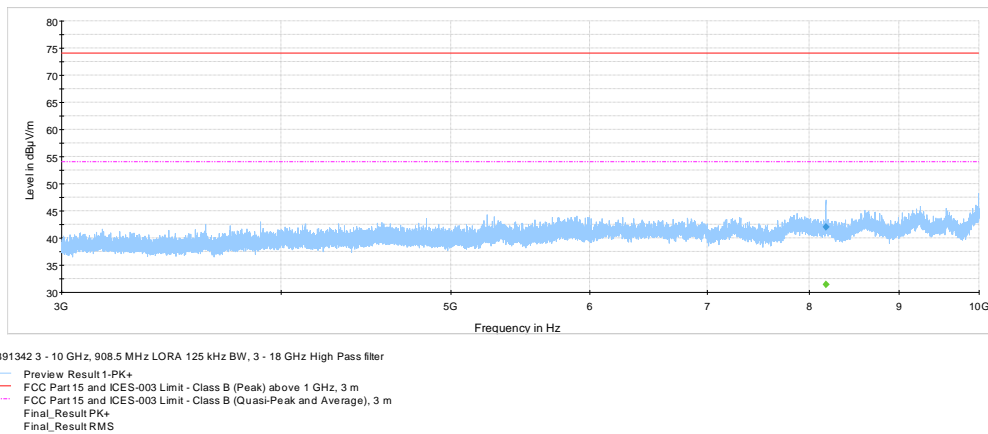
Figure 8.8-13: Radiated spurious emissions 3 - 10 GHz, 908.5 MHz LoRa 125 kHz BW
