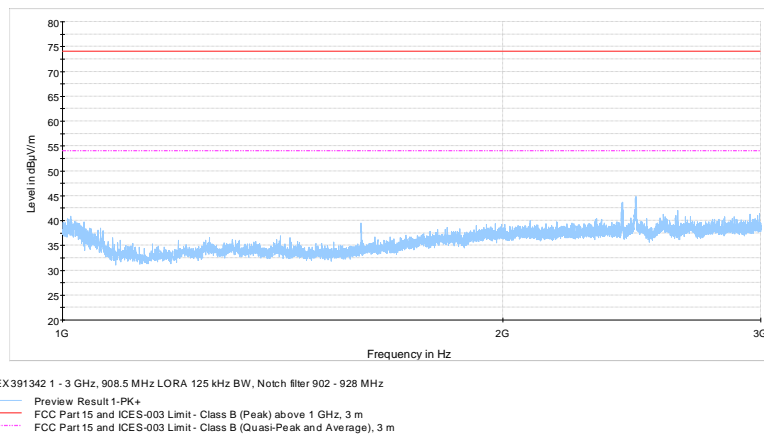
Figure 8.8-10: Radiated spurious emissions 1 - 3 GHz, 908.5 MHz LoRa 125 kHz BW
