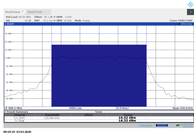
Figure 8.7-3: Output power on mid channel, 125 kHz BW
