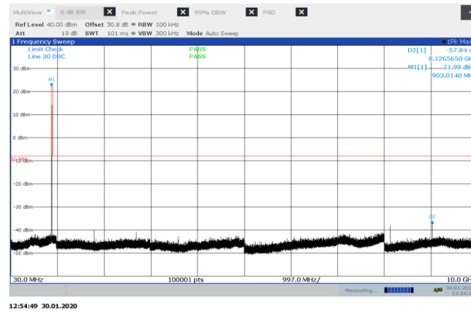
Figure 8.8-17: Conducted spurious emissions on low channel, 500 kHz BW
