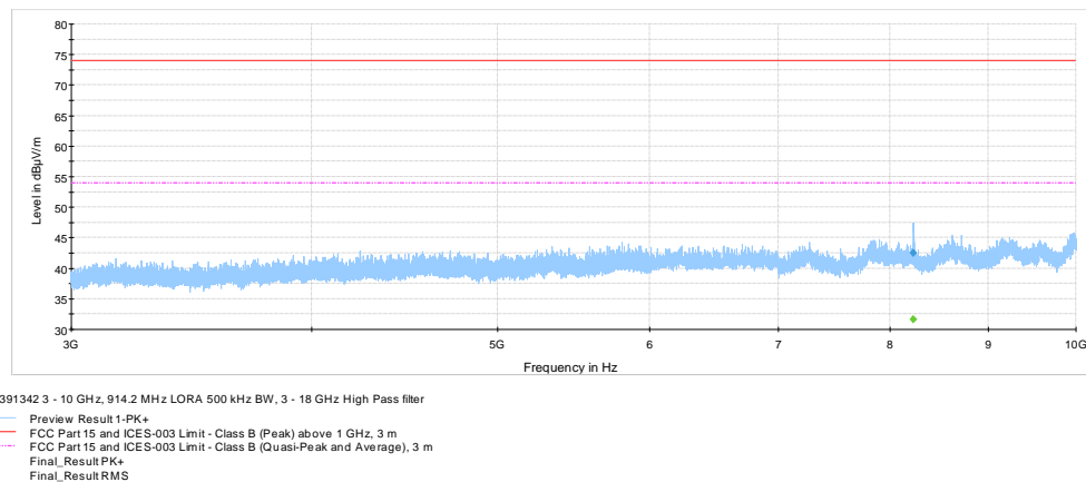
Figure 8.8-28: Radiated spurious emissions 3 – 10 GHz, 914.2 MHz LoRa 500 kHz BW
