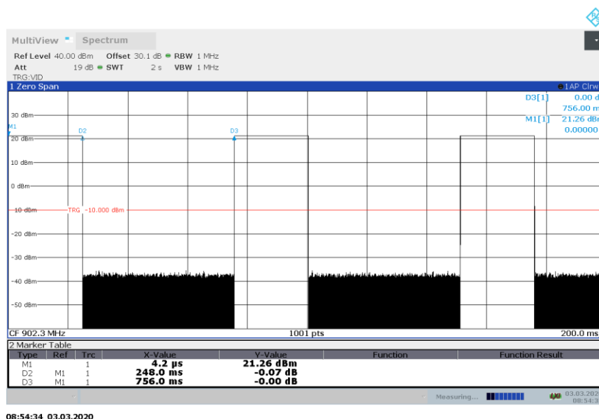
Figure 8.7-1: Duty cycle on low channel, 125 kHz BW
