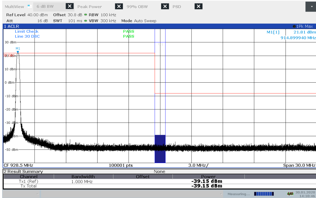
Figure 8.8-1: Conducted Band-edge low channel, 125 kHz BW
