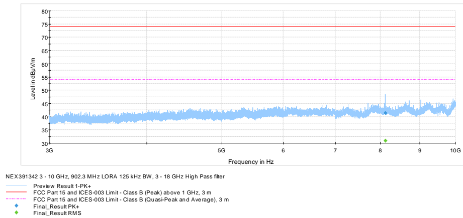
Figure 8.8-12: Radiated spurious emissions 3 - 10 GHz, 902.3 MHz LoRa 125 kHz BW
