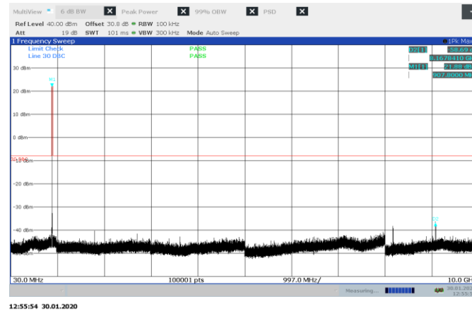
Figure 8.8-18: Conducted spurious emissions on mid channel, 500 kHz BW
