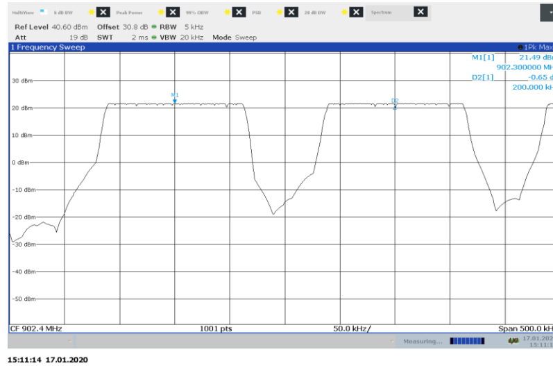
Figure 8.5-7: Carrier frequency separation
