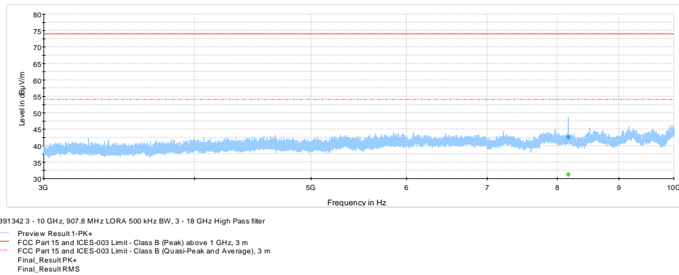
Figure 8.8-27: Radiated spurious emissions 3 – 10 GHz, 907.8 MHz LoRa 500 kHz BW
