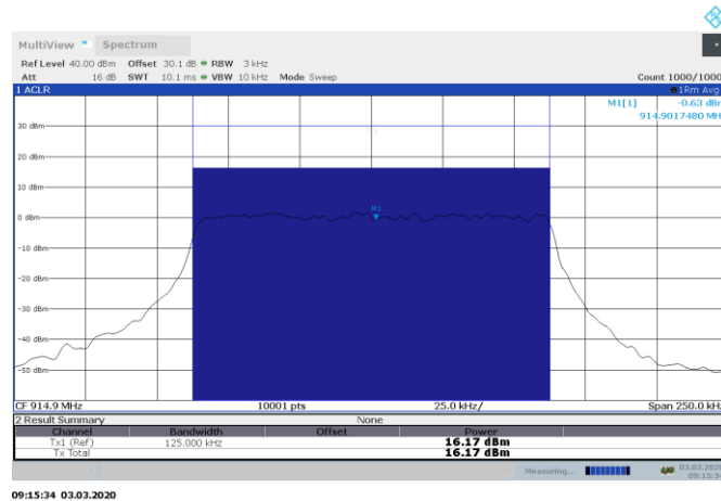
Figure 8.7-4: Output power on high channel, 125 kHz BW
