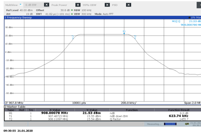
Figure 8.6-2: 6 dB bandwidth on mid channel, 500 kHz BW
