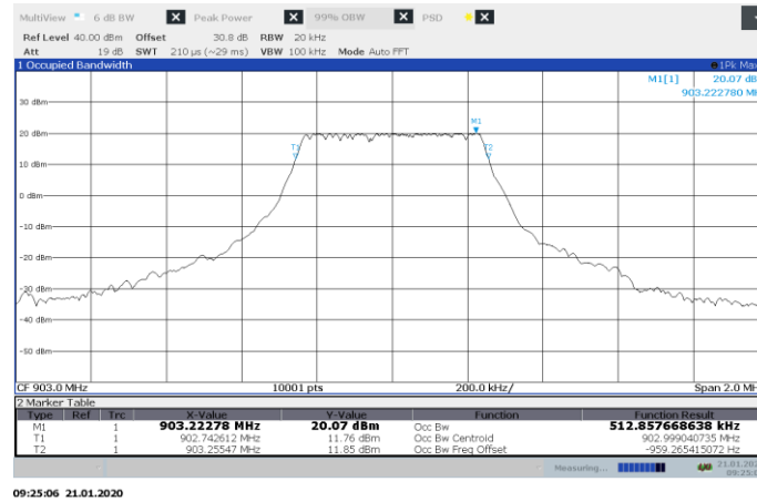
Figure 8.6-4: 99% OBW on low channel, 500 kHz BW
