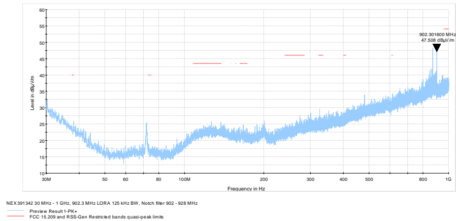
Figure 8.8-6: Radiated spurious emissions 30 MHz – 1 GHz, 902.3 MHz LORA 125 kHz BW
