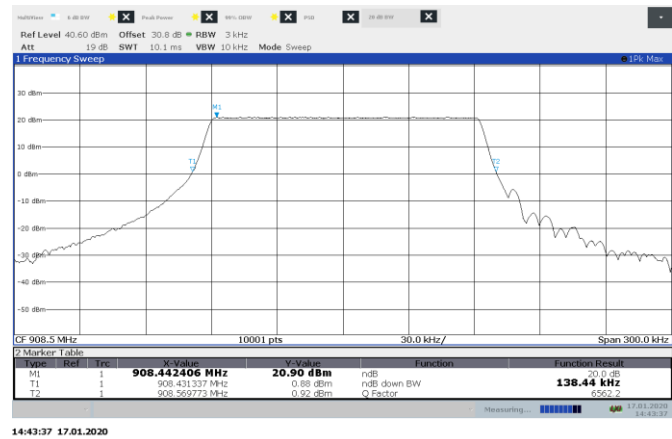
Figure 8.5-2: 20 dB bandwidth on mid channel, 125 kHz BW
