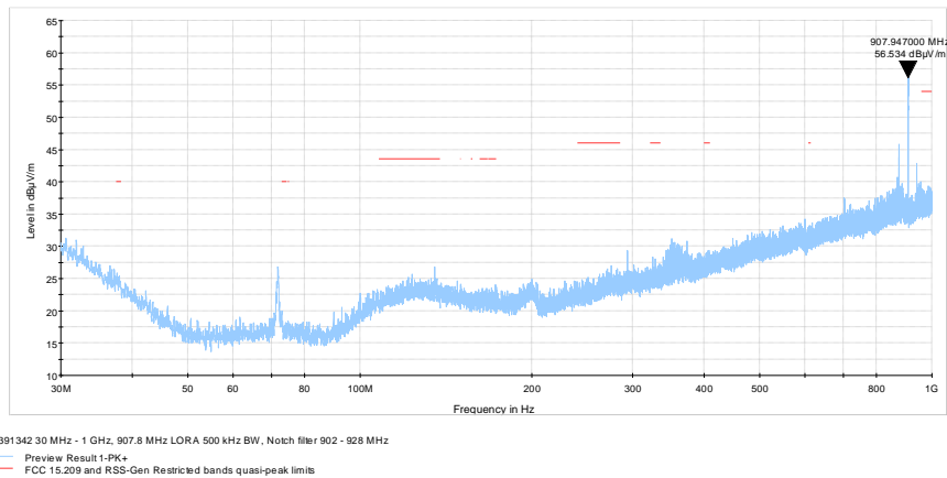
Figure 8.8-21: Radiated spurious emissions 30 MHz – 1 GHz, 907.8 MHz LoRa 500 kHz BW
