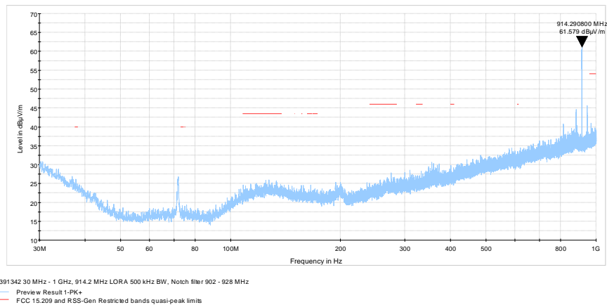
Figure 8.8-22: Radiated spurious emissions 30 MHz – 1 GHz, 914.2 MHz LoRa 500 kHz BW
