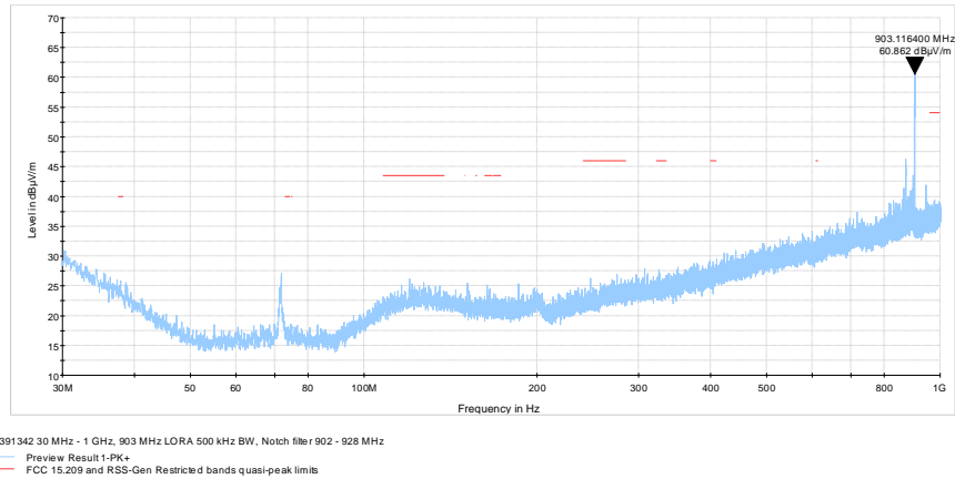
Figure 8.8-20: Radiated spurious emissions 30 MHz – 1 GHz, 903 MHz LoRa 500 kHz BW
