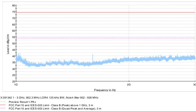
Figure 8.8-9: Radiated spurious emissions 1 - 3 GHz, 902.3 MHz LoRa 125 kHz BW
