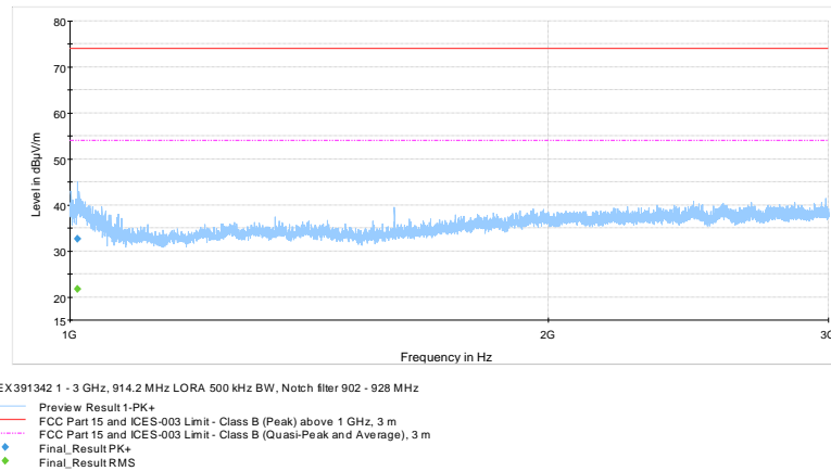
Figure 8.8-25: Radiated spurious emissions 1 - 3 GHz, 914.2 MHz LoRa 500 kHz BW
