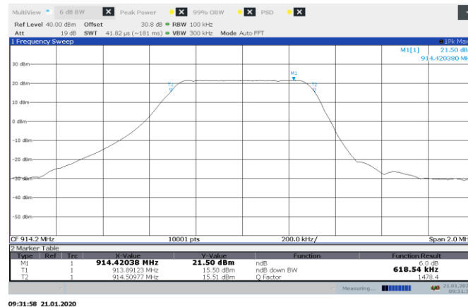
Figure 8.6-3: 6 dB bandwidth on high channel, 500 kHz BW
