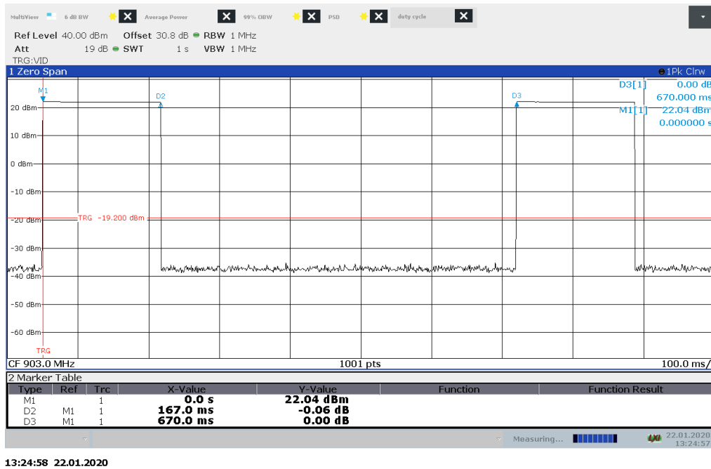
Figure 8.7-5: Duty cycle on low channel, 500 kHz BW
