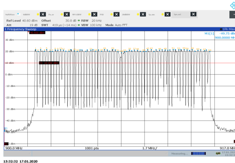
Figure 8.5-8: Number of hopping channels = 64
