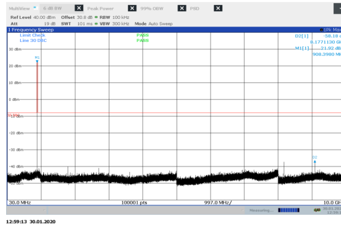
Figure 8.8-4: Conducted spurious emissions on mid channel, 125 kHz BW
