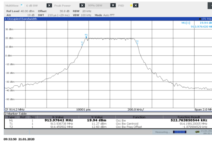
Figure 8.6-6: 99% OBW on high channel, 500 kHz BW
