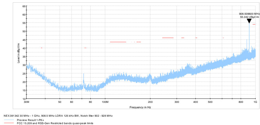
Figure 8.8-7: Radiated spurious emissions 30 MHz – 1 GHz, 908.5 MHz LoRa 125 kHz BW
