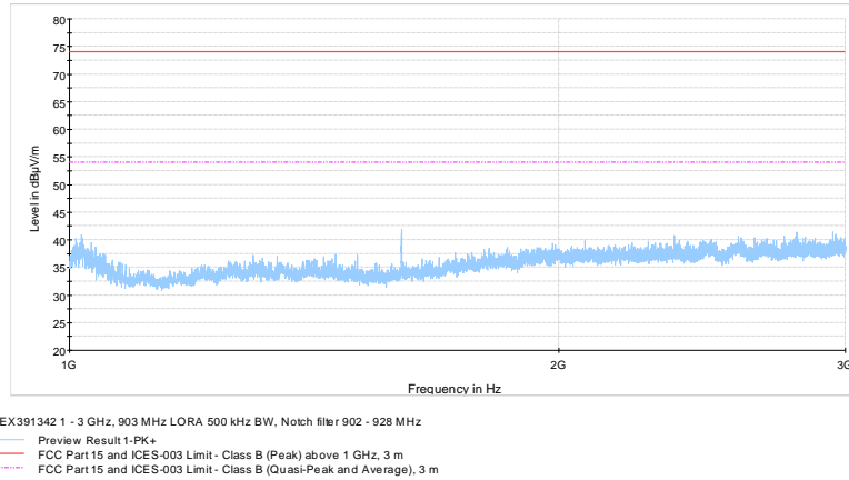
Figure 8.8-23: Radiated spurious emissions 1 - 3 GHz, 903 MHz LoRa 500 kHz BW
