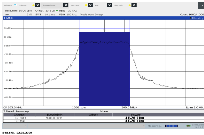
Figure 8.7-6: Output power on low channel, 500 kHz BW
