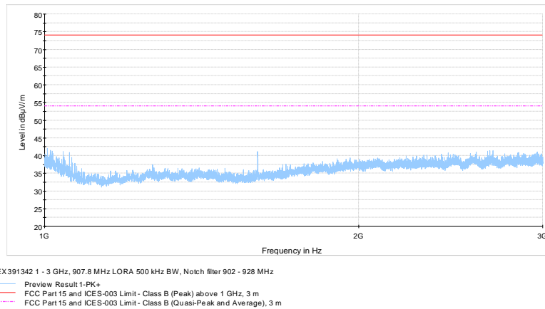
Figure 8.8-24: Radiated spurious emissions 1 - 3 GHz, 907.8 MHz LoRa 500 kHz BW
