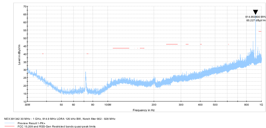
Figure 8.8-8: Radiated spurious emissions 30 MHz – 1 GHz, 914.9 MHz LoRa 125 kHz BW
