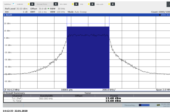
Figure 8.7-8: Output power on high channel, 500 kHz BW
