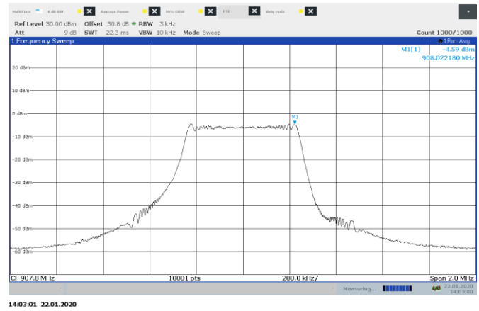
Figure 8.9-5: PSD on mid channel, 500 kHz BW
