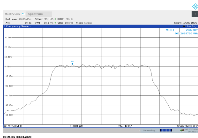
Figure 8.9-1: PSD on low channel, 125 kHz BW
