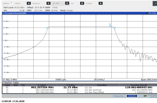
Figure 8.5-4: 99% OBW on low channel, 125 kHz BW
