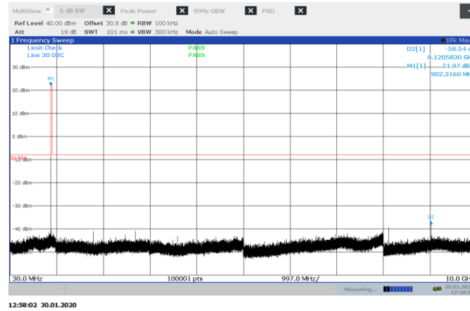
Figure 8.8-3: Conducted spurious emissions on low channel, 125 kHz BW
