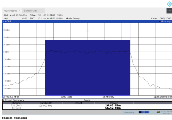
Figure 8.7-2: Output power on low channel, 125 kHz BW
