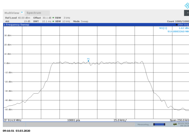
Figure 8.9-3: PSD on high channel, 125 kHz BW
