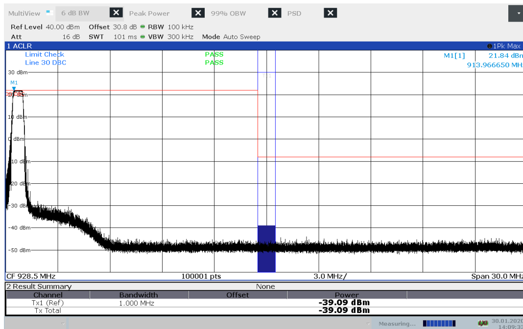
Figure 8.8-15: Conducted Band-edge low channel, 500 kHz BW
