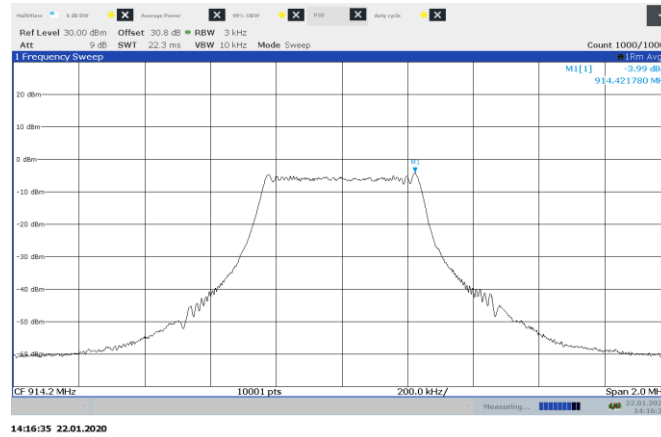
Figure 8.9-6: PSD on high channel, 500 kHz BW
