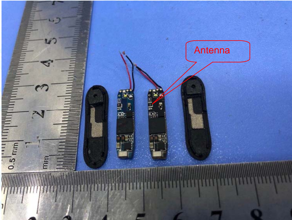
Photo 14 Appearance PCB
