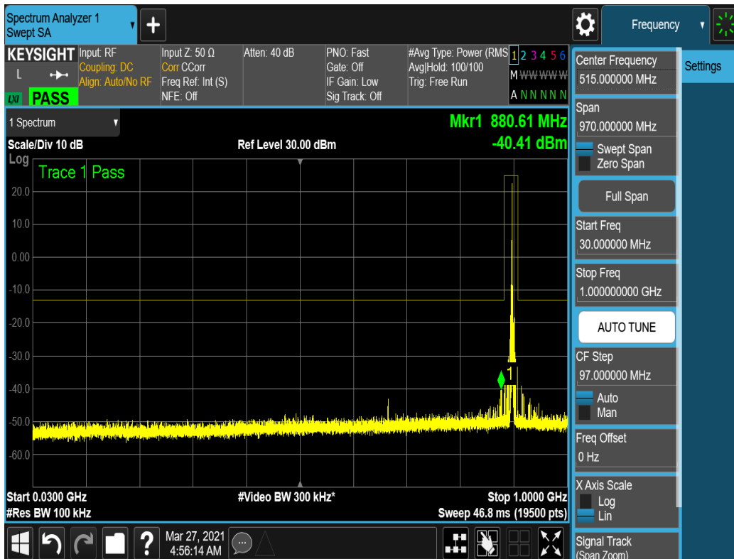
Plot 7-17. Conducted Spurious Plot – High Channel (1.4MHz, QPSK, 1RB, RB Offset 0)
