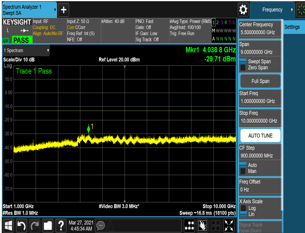
Plot 7-14. Conducted Spurious Plot – Mid Channel (1.4MHz, QPSK, 1RB, RB Offset 5)
