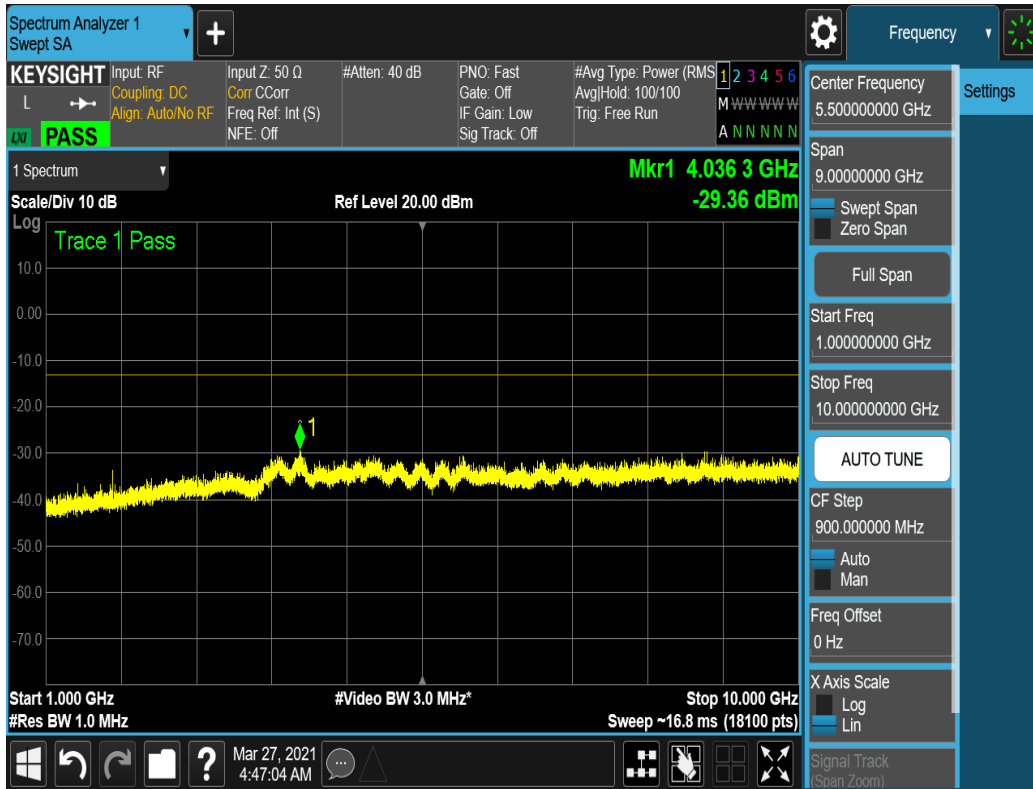
Plot 7-16. Conducted Spurious Plot – Low Channel (1.4MHz, QPSK, 1RB, RB Offset 0)
