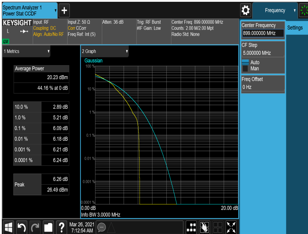
Plot 7-20. Peak to Average Ratio (3MHz, 16-QAM, RB 6, RB Offset 0, NB=0)
