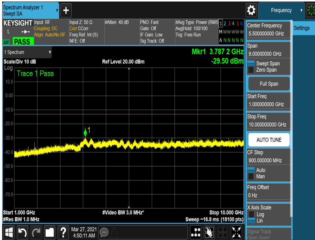
Plot 7-18. Conducted Spurious Plot – High Channel (1.4MHz, QPSK, 1RB, RB Offset 0)
