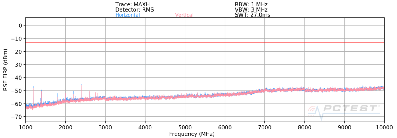
Plot 7-23. Radiated Spurious Plot (LTE Band 8- CAT-M1)
