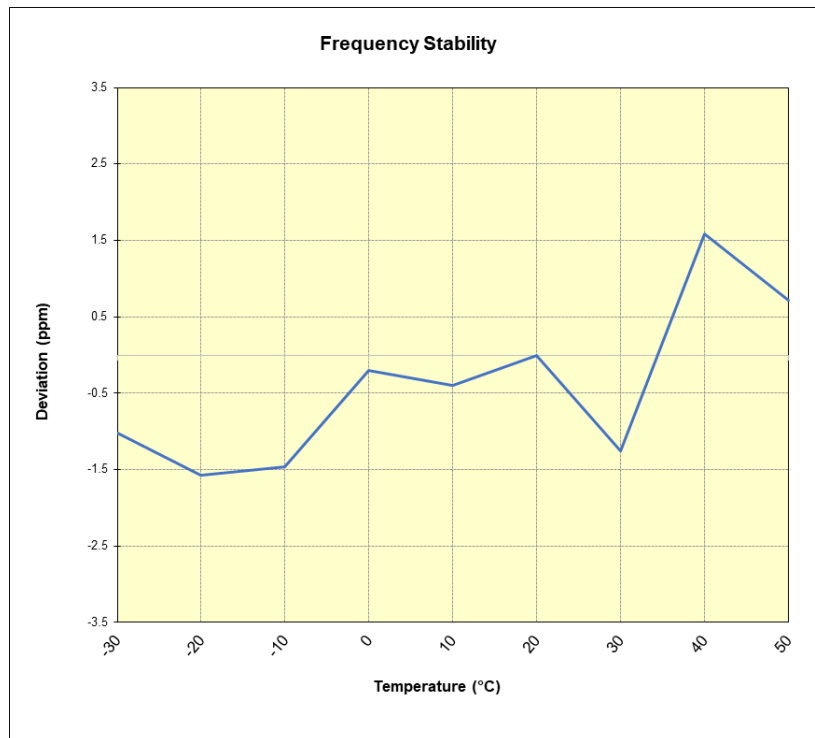
Plot 7-23. LTE Band 8 CAT-M1 Frequency Stability Chart
