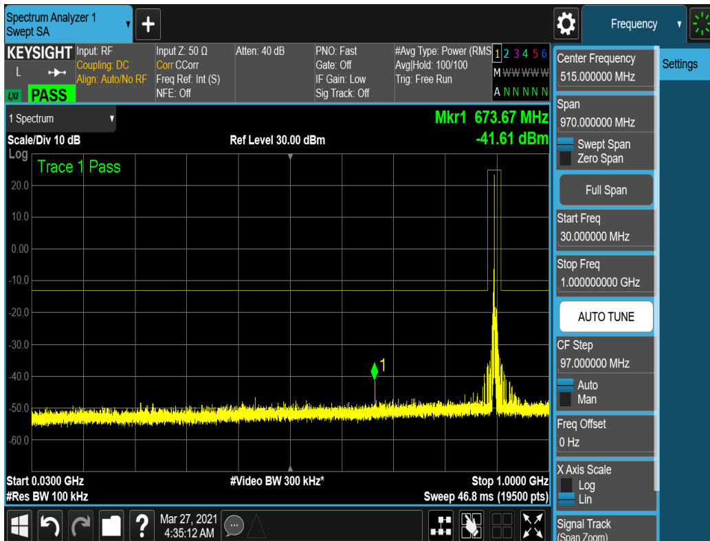
Plot 7-15. Conducted Spurious Plot – Low Channel (1.4MHz, QPSK, 1RB, RB Offset 0)
