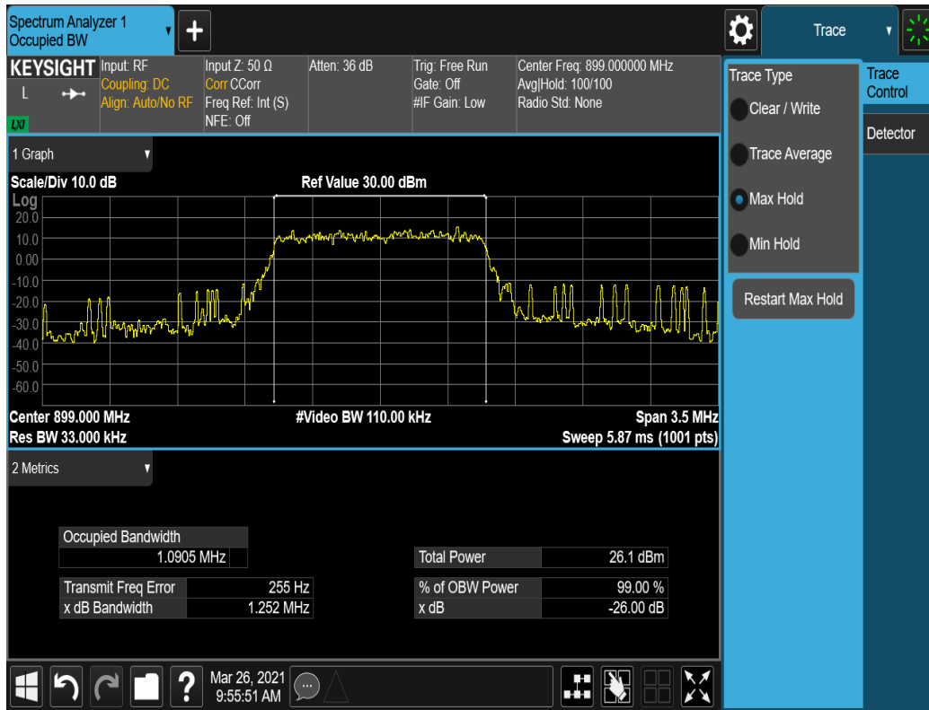
Plot 7-6. Occupied Bandwidth Plot (1.4MHz, 16QAM, RB 6, RB Offset 0, NB=0)
