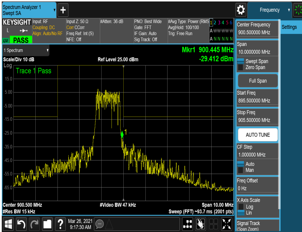
Plot 7-10. Upper Band Edge Plot (1.4MHz, QPSK, 6RB, RB Offset 0, NB=0)
