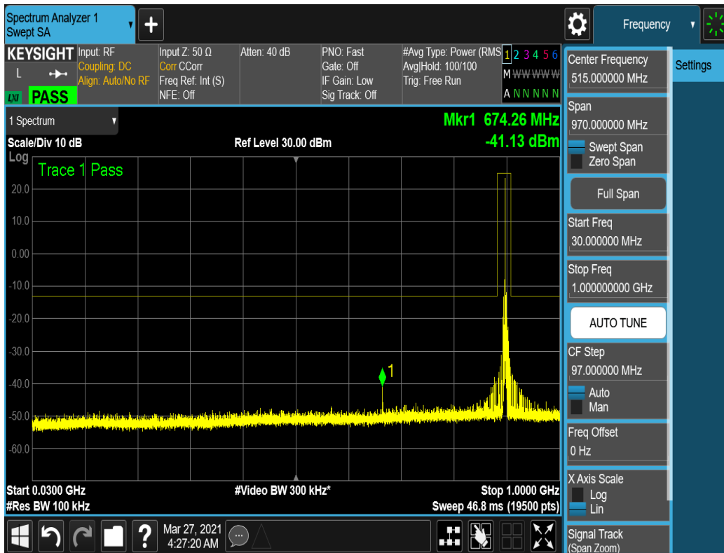
Plot 7-13. Conducted Spurious Plot – Mid Channel (1.4MHz, QPSK, 1RB, RB Offset 5)
