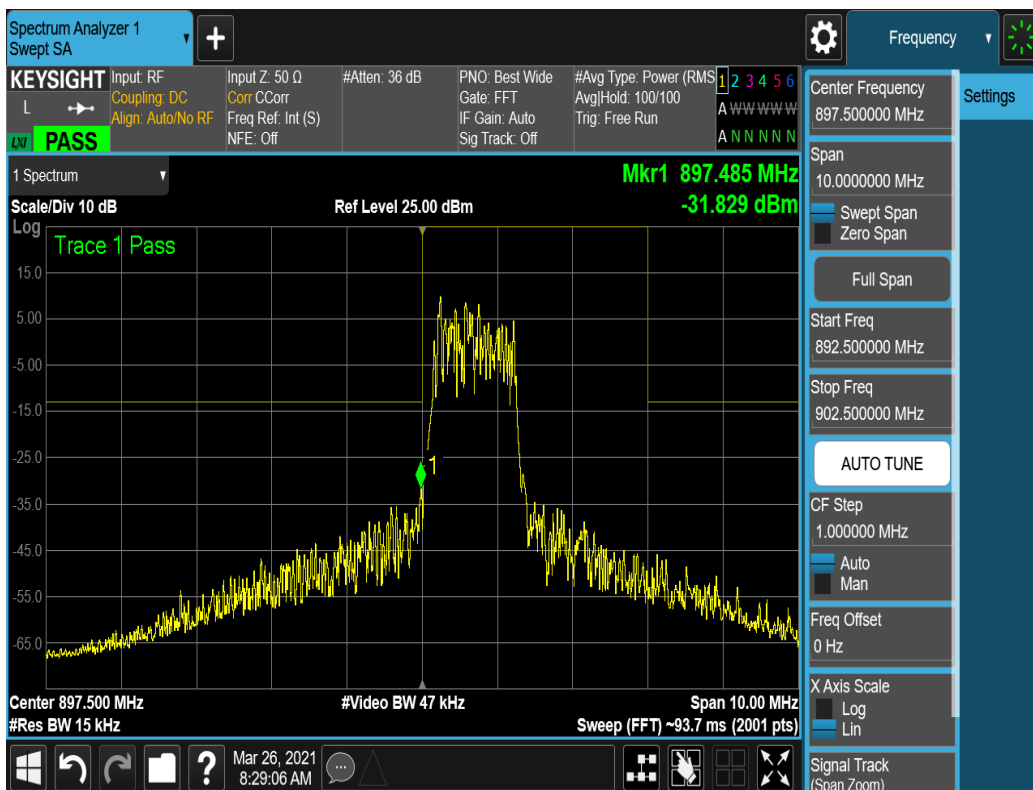
Plot 7-9. Lower Band Edge Plot (1.4MHz, QPSK, 6RB, RB Offset 0, NB=0)
