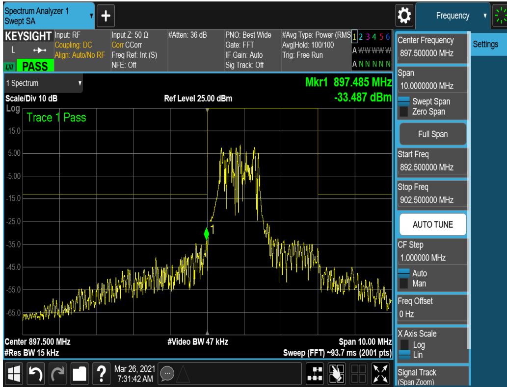
Plot 7-7. Lower Band Edge Plot (3MHz, QPSK, 6RB, RB Offset 0, NB=0)
