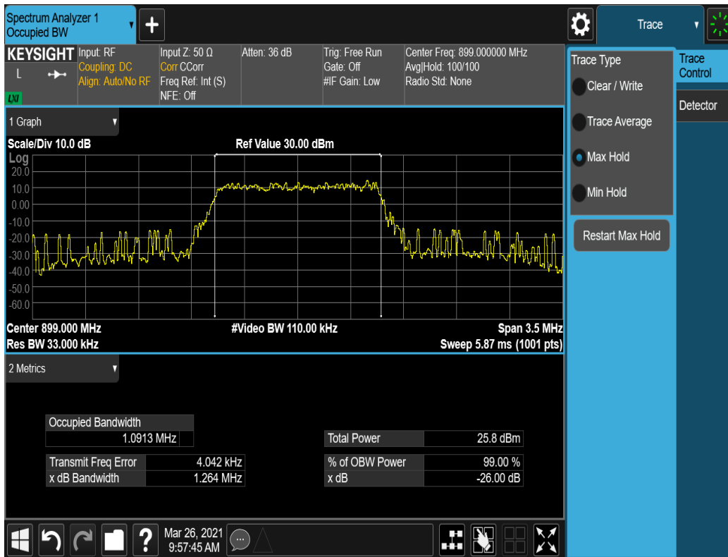
Plot 7-4. Occupied Bandwidth Plot (3MHz, 16QAM, RB 6, RB Offset 0, NB=1)
