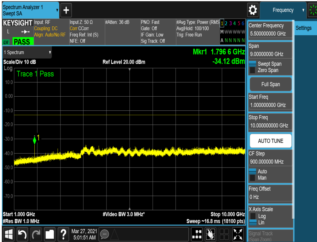
Plot 7-12. Conducted Spurious Plot – Mid Channel (3MHz, QPSK, 1RB, RB Offset 3)
