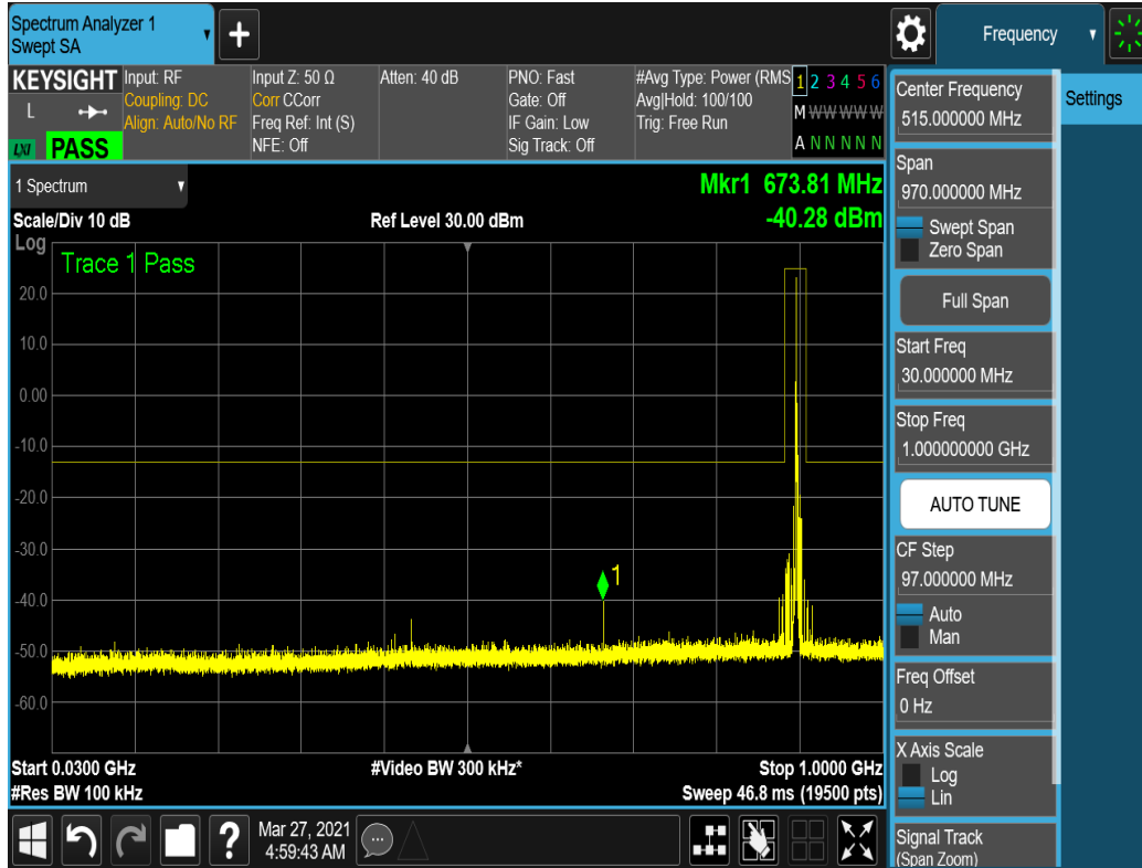
Plot 7-11. Conducted Spurious Plot – Mid Channel (3MHz, QPSK, 1RB, RB Offset 3)
