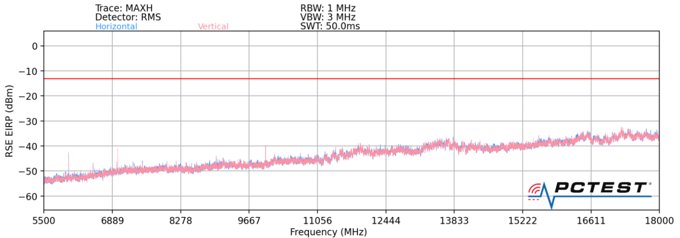
Plot 7-8. Radiated Spurious Plot (LTE Band 8 / LTE Band 13 / LTE B12)
