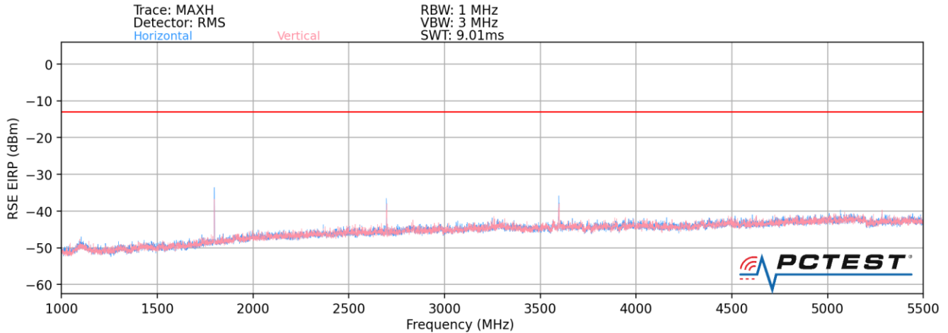
Plot 7-7. Radiated Spurious Plot (LTE Band 8 / LTE Band 13 / LTE B12)
