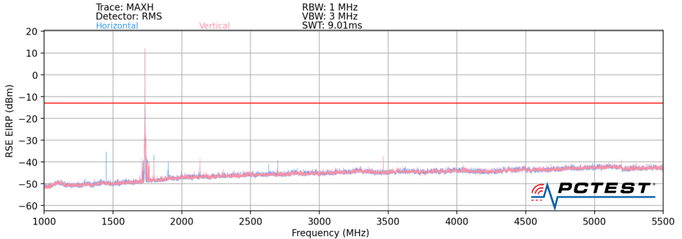
Plot 7-25. Radiated Spurious Plot (LTE Band 4 / LTE Band 8 / LTE Band 12)
