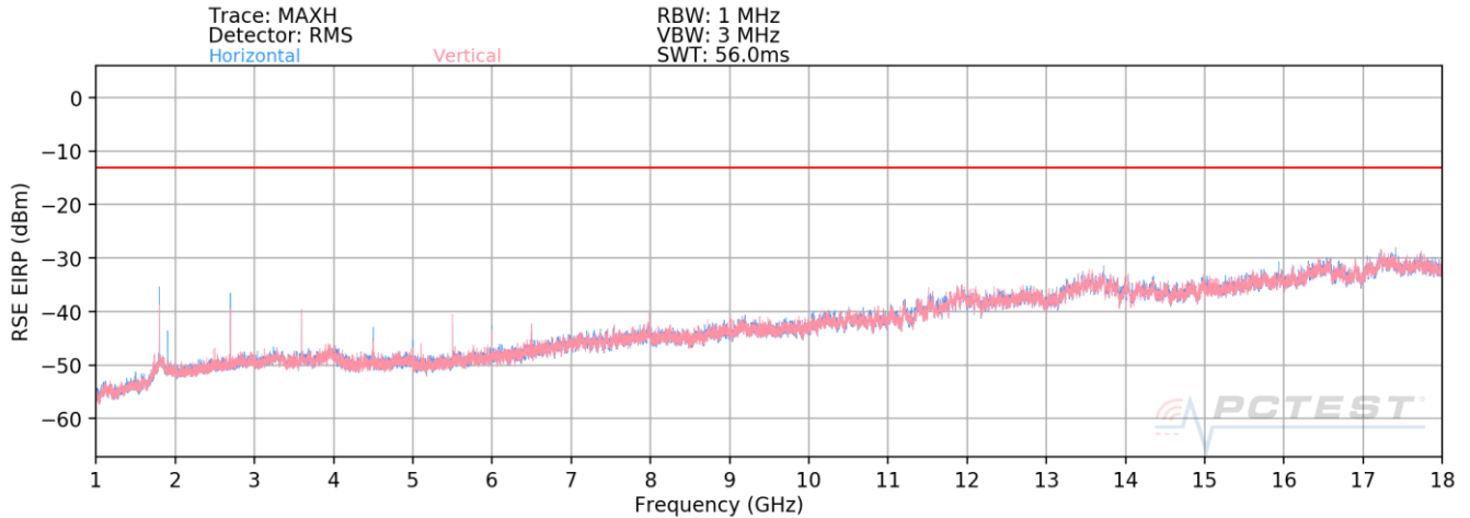
Plot 7-4. Radiated Spurious Plot (LTE Band 8 / LTE Band 8 / LTE B12)
