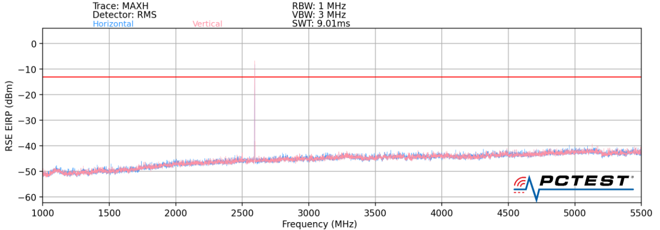
Plot 7-23. Radiated Spurious Plot (LTE Band 12 / LTE Band 8 / LTE Band 41)
