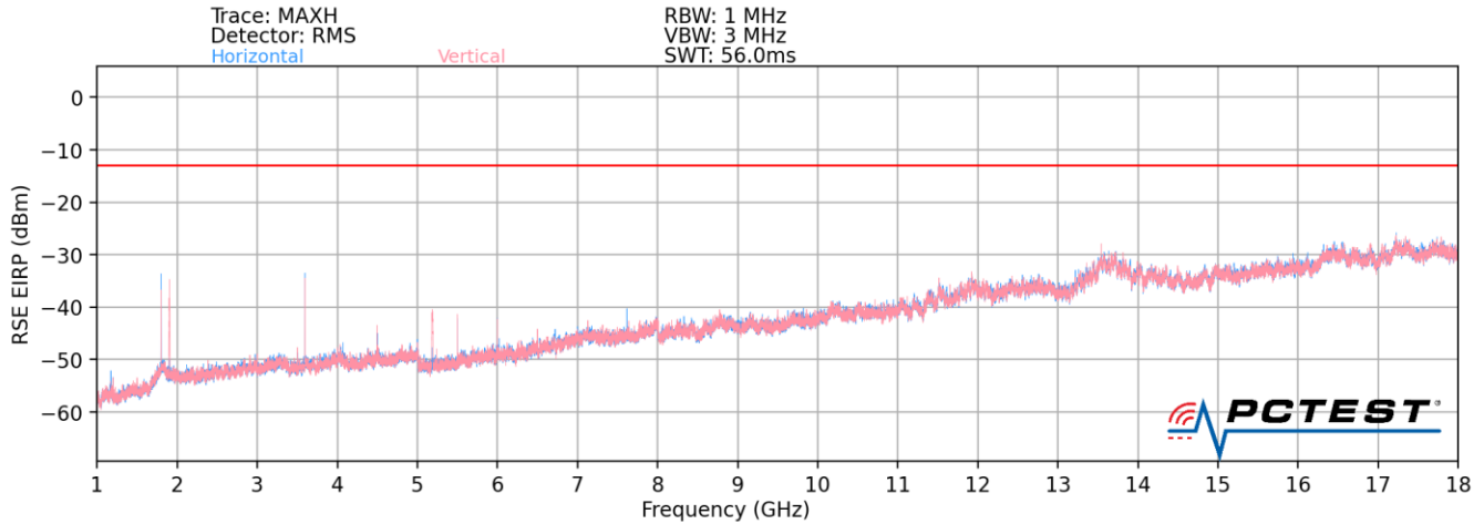
Plot 7-21. Radiated Spurious Plot (LTE Band 8 / LTE Band 41 / LTE Band 7)
