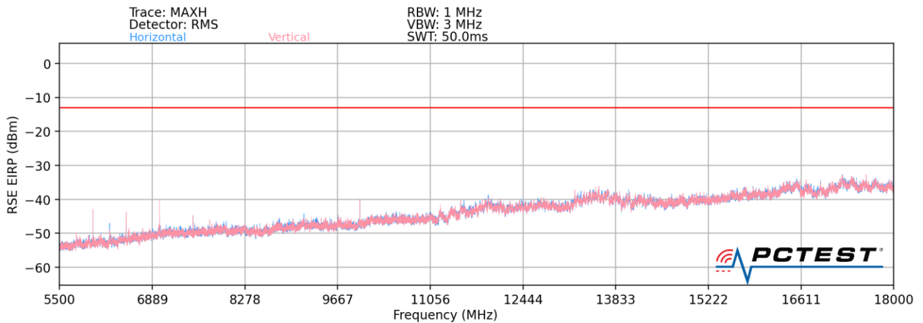
Plot 7-12. Radiated Spurious Plot (LTE Band 8 / LTE Band 13 / LTE Band 41)
