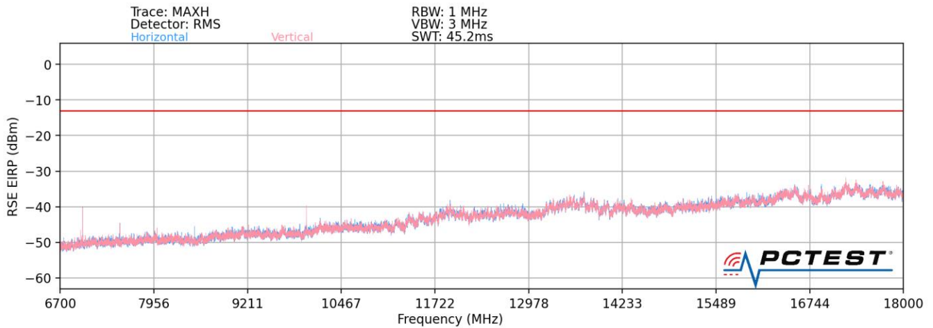
Plot 7-10. Radiated Spurious Plot (LTE Band 8 / LTE Band 13 / LTE B4)
