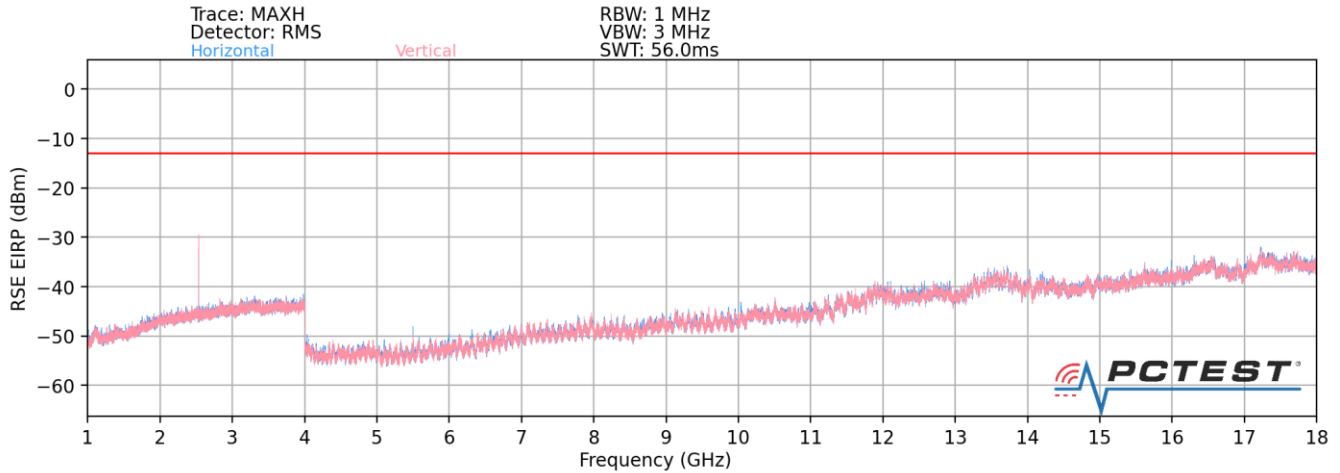
Plot 7-3. Radiated Spurious Plot (LTE Band 8 / LTE Band 8 / LTE B7)
