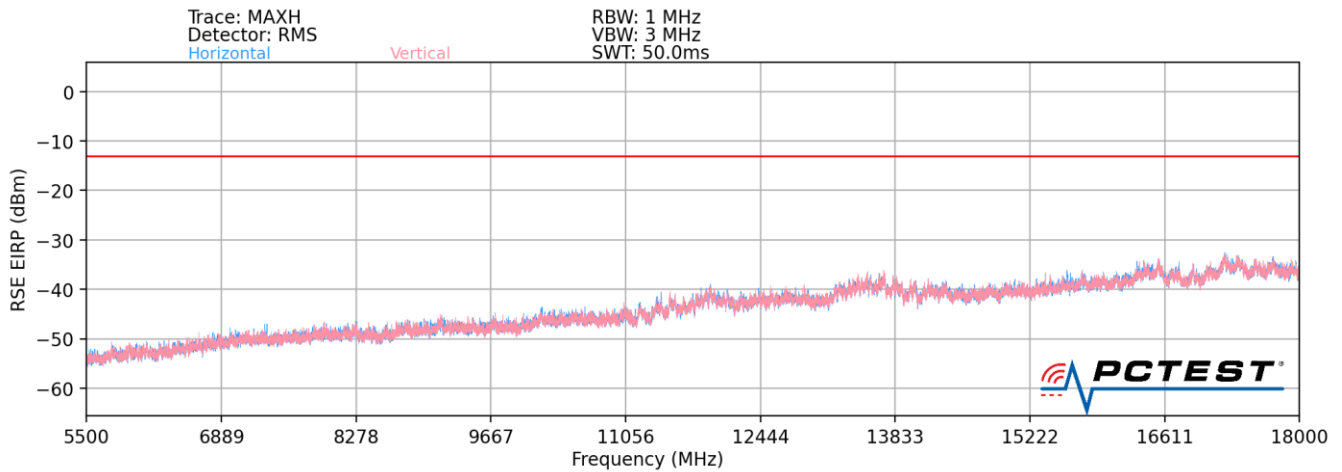
Plot 7-26. Radiated Spurious Plot (LTE Band 4 / LTE Band 8 / LTE Band 12)
