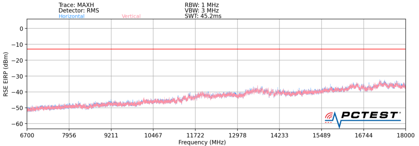
Plot 7-30. Radiated Spurious Plot (LTE Band 4 / LTE Band 8 / LTE Band 41)
