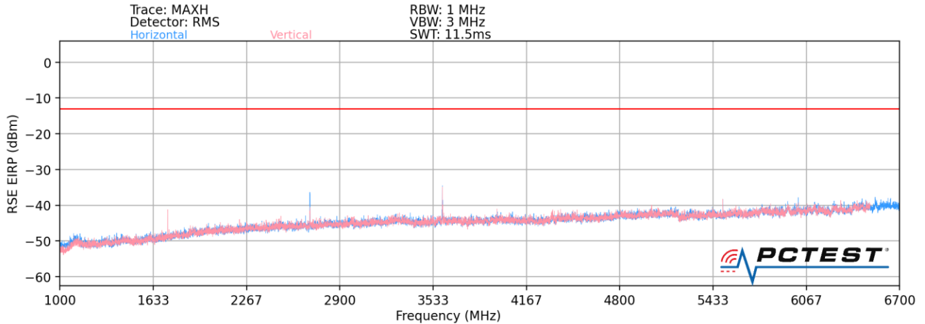
Plot 7-9. Radiated Spurious Plot (LTE Band 8 / LTE Band 13 / LTE B4)
