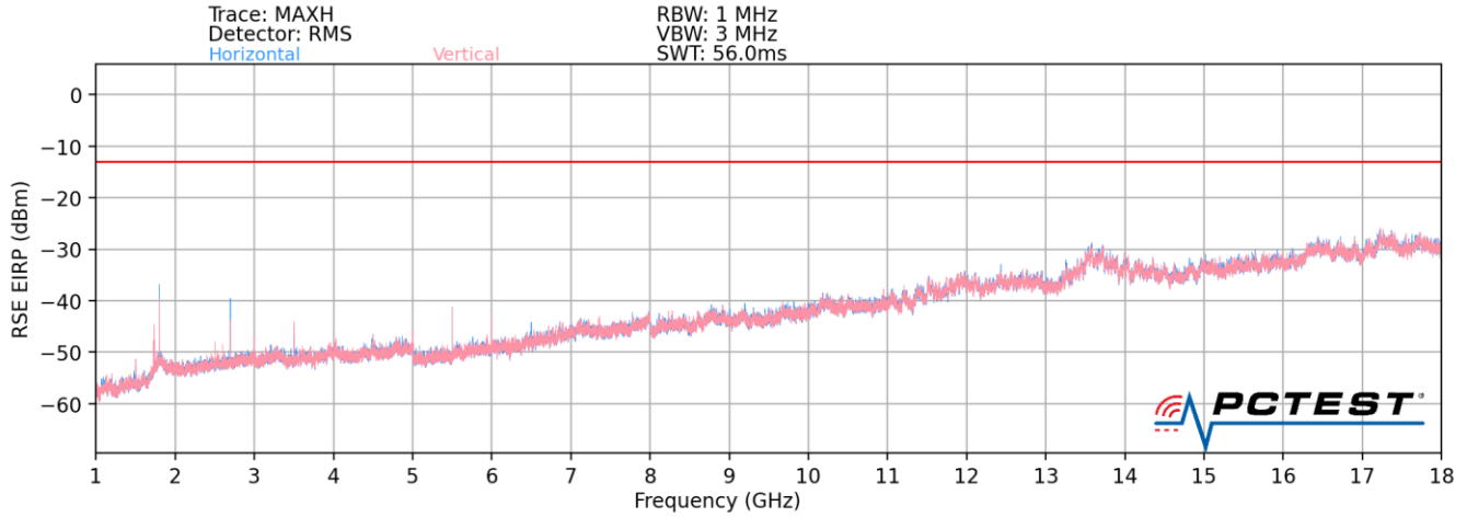
Plot 7-22. Radiated Spurious Plot (LTE Band 12 / LTE Band 8 / LTE Band 12)
