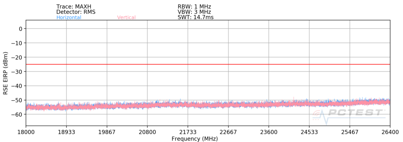
Plot 7-13. Radiated Spurious Plot (LTE Band 8 / LTE Band 13 / LTE Band 41)
