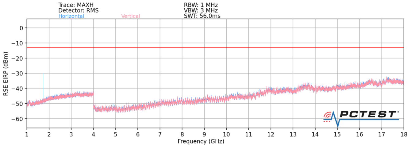
Plot 7-5. Radiated Spurious Plot (LTE Band 8 / LTE Band 8 / LTE B4)
