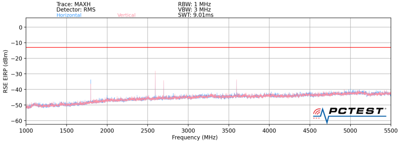
Plot 7-11. Radiated Spurious Plot (LTE Band 8 / LTE Band 13 / LTE Band 41)
