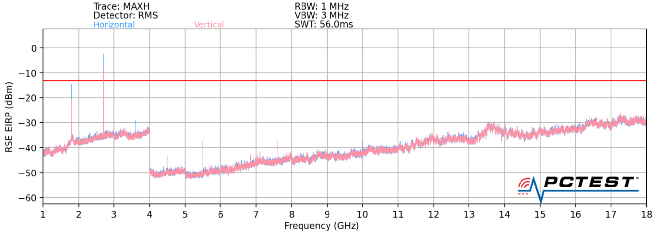
Plot 7-16. Radiated Spurious Plot (LTE Band 8 / LTE Band 4 / LTE Band 41)
