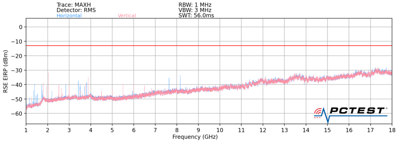
Plot 7-14. Radiated Spurious Plot (LTE Band 8 / LTE Band 4 / LTE Band 12)
