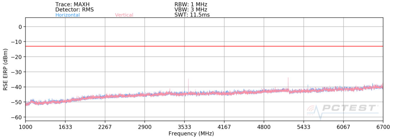
Plot 7-19. Radiated Spurious Plot (LTE Band 8 / LTE Band 41 / LTE Band 4)
