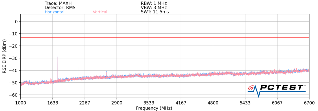
Plot 7-27. Radiated Spurious Plot (LTE Band 4 / LTE Band 8 / LTE Band 4)
