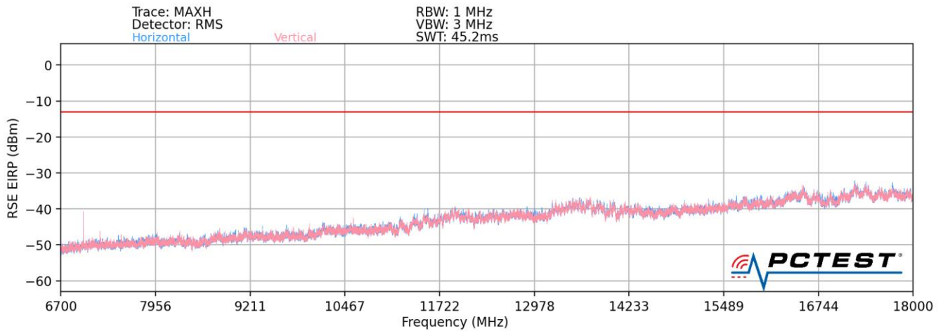
Plot 7-20. Radiated Spurious Plot (LTE Band 8 / LTE Band 41 / LTE Band 4)
