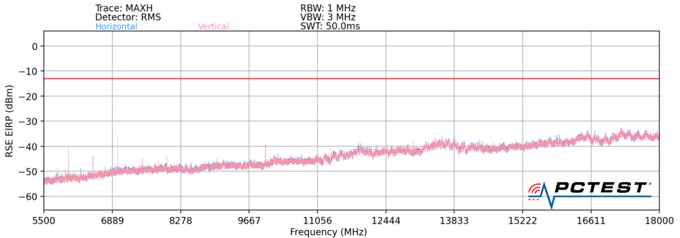
Plot 7-18. Radiated Spurious Plot (LTE Band 8 / LTE Band 41 / LTE Band 12)
