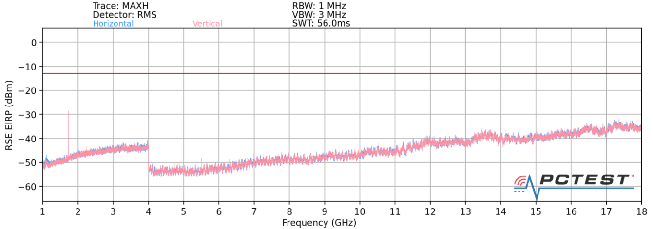
Plot 7-2. Radiated Spurious Plot (LTE Band 8 / LTE Band 8 / LTE B4)
