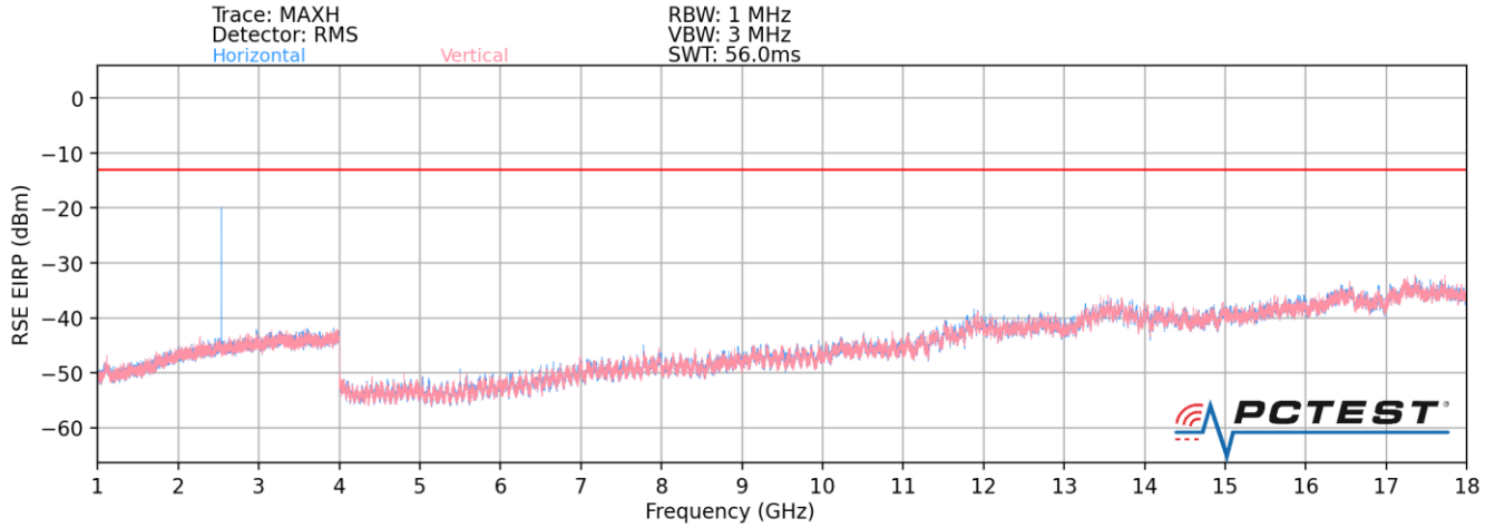
Plot 7-6. Radiated Spurious Plot (LTE Band 8 / LTE Band 8 / LTE B7)
