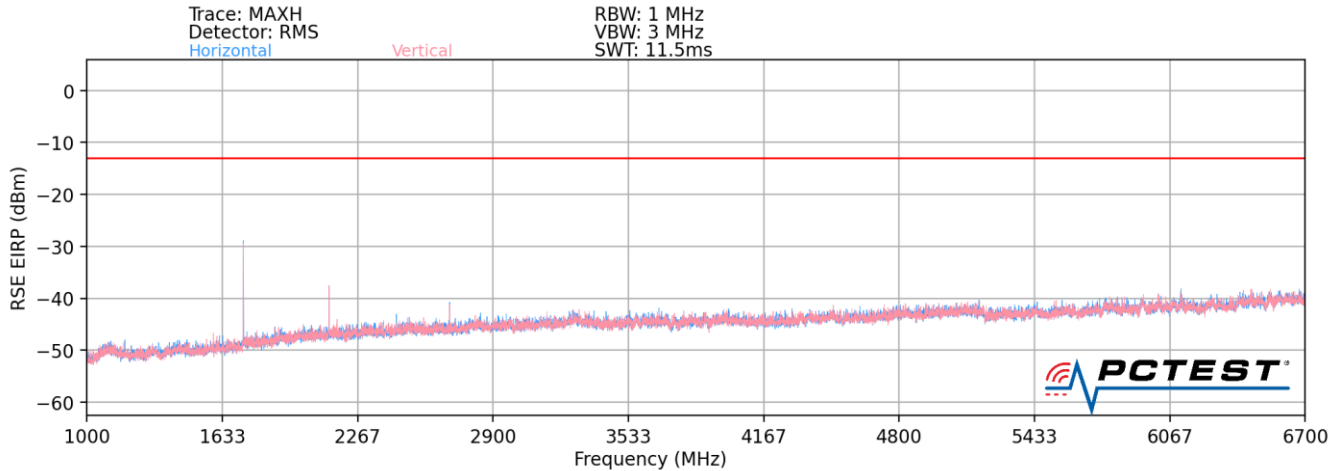
Plot 7-29. Radiated Spurious Plot (LTE Band 4 / LTE Band 8 / LTE Band 41)
