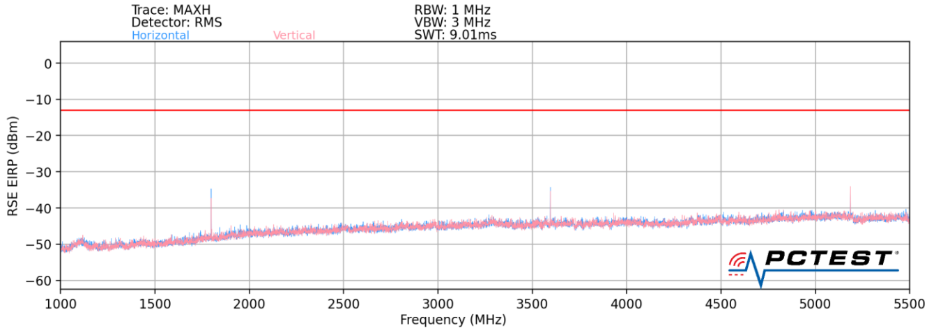
Plot 7-17. Radiated Spurious Plot (LTE Band 8 / LTE Band 41 / LTE Band 12)
