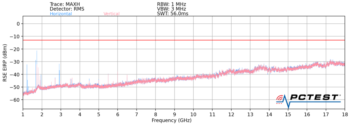
Plot 7-15. Radiated Spurious Plot (LTE Band 8 / LTE Band 4 / LTE Band 4)
