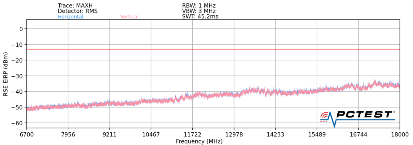
Plot 7-28. Radiated Spurious Plot (LTE Band 4 / LTE Band 8 / LTE Band 4)
