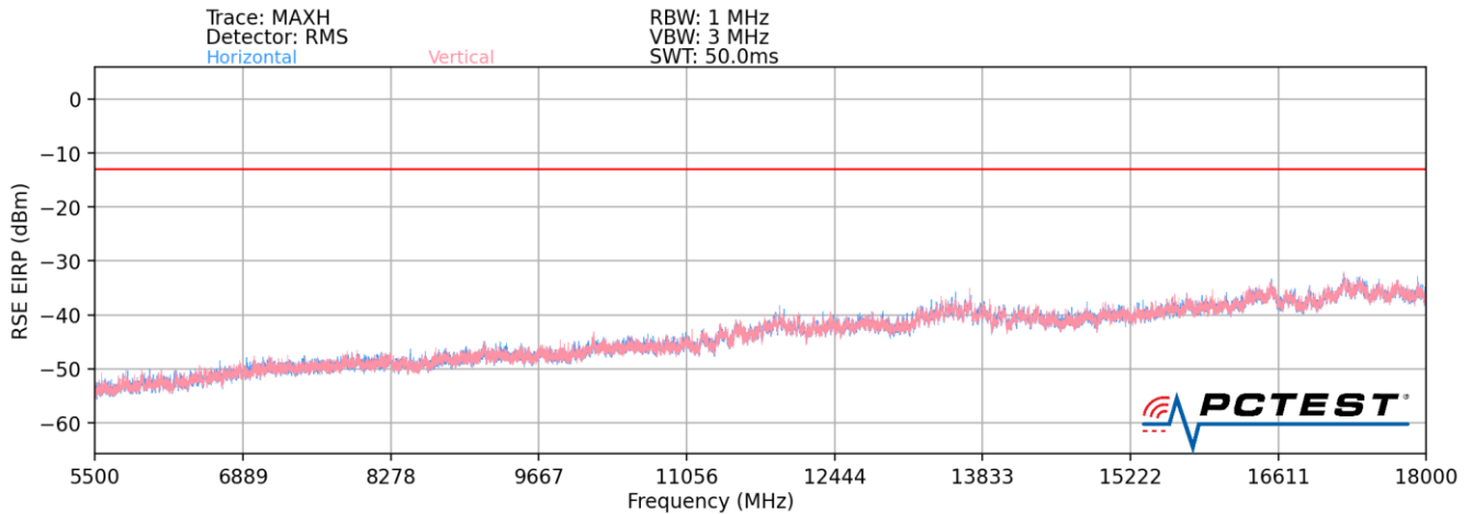
Plot 7-24. Radiated Spurious Plot (LTE Band 12 / LTE Band 8 / LTE Band 41)
