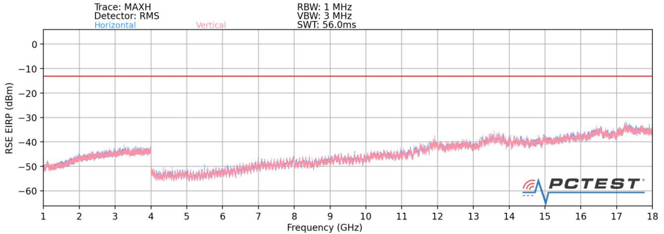
Plot 7-1. Radiated Spurious Plot (LTE Band 8 / LTE Band 8 / LTE B12)
