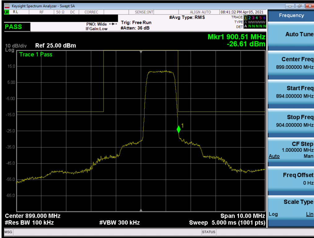
Plot 7-8. Upper Band Edge Plot (1.4 MHz, QPSK, 6 RB, 0 Offset)
