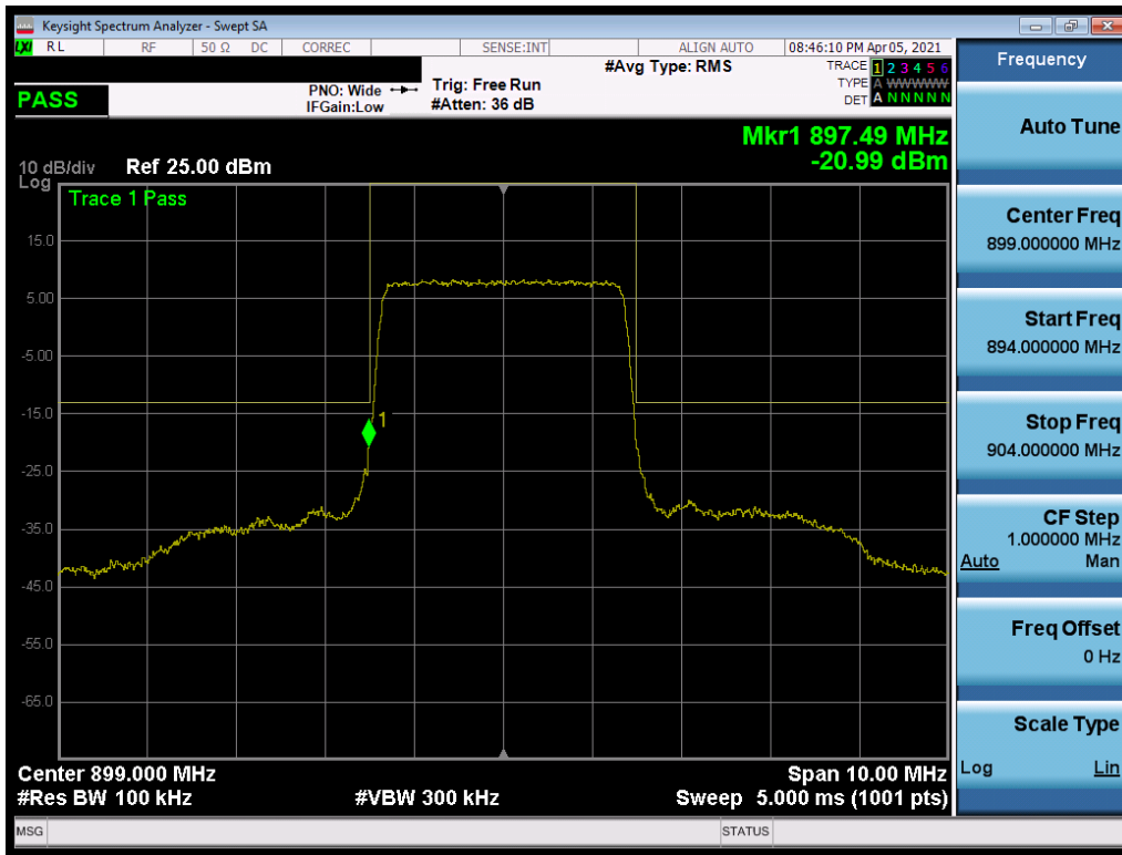
Plot 7-5. Lower Band Edge Plot (3 MHz, QPSK, 15 RB, 0 Offset)
