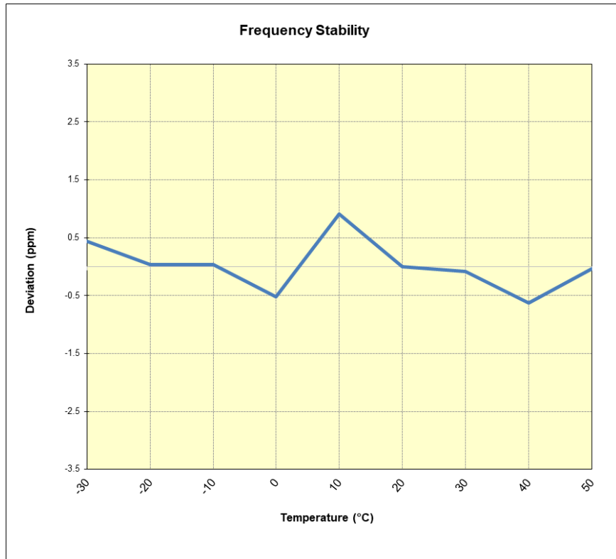
Plot 7-18. LTE Band 8 Frequency Stability Chart
