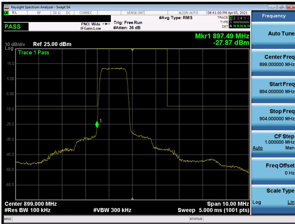
Plot 7-7. Lower Band Edge Plot (1.4 MHz, QPSK, 6 RB, 0 Offset)
