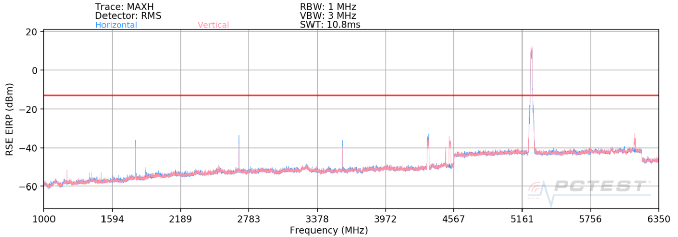
Plot 7-12. Radiated Spurious Plot (LTE Band 8 (rad) / LTE Band 12 (cond) / 5GHz)
