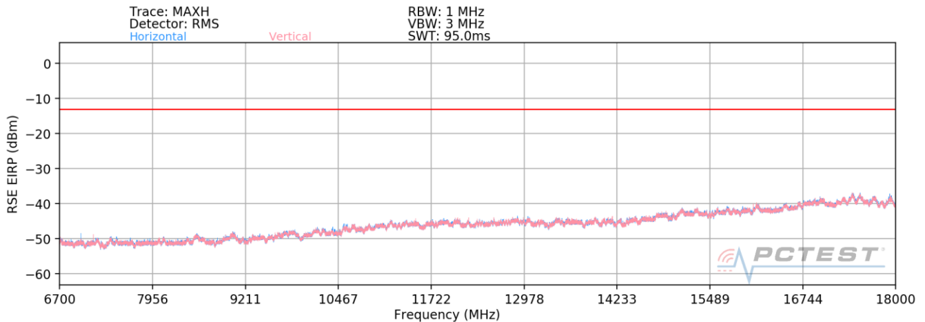
Plot 7-17. Radiated Spurious Plot (LTE Band 8 (rad) / LTE Band 4 (cond) / 5GHz)
