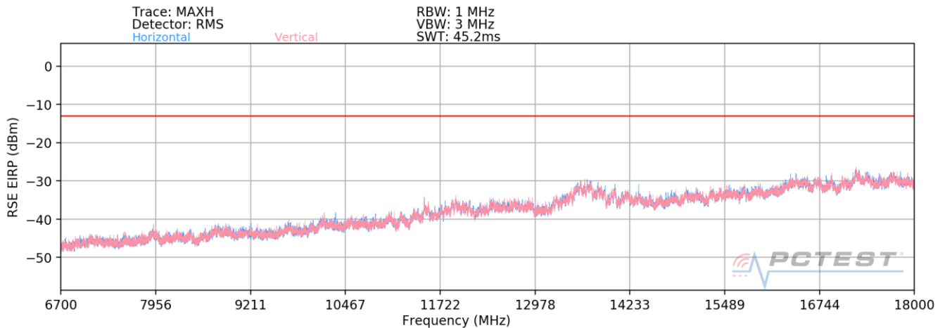
Plot 7-29. Radiated Spurious Plot (LTE Band 4 (cond) / LTE Band 8 (rad) / 5GHz)
