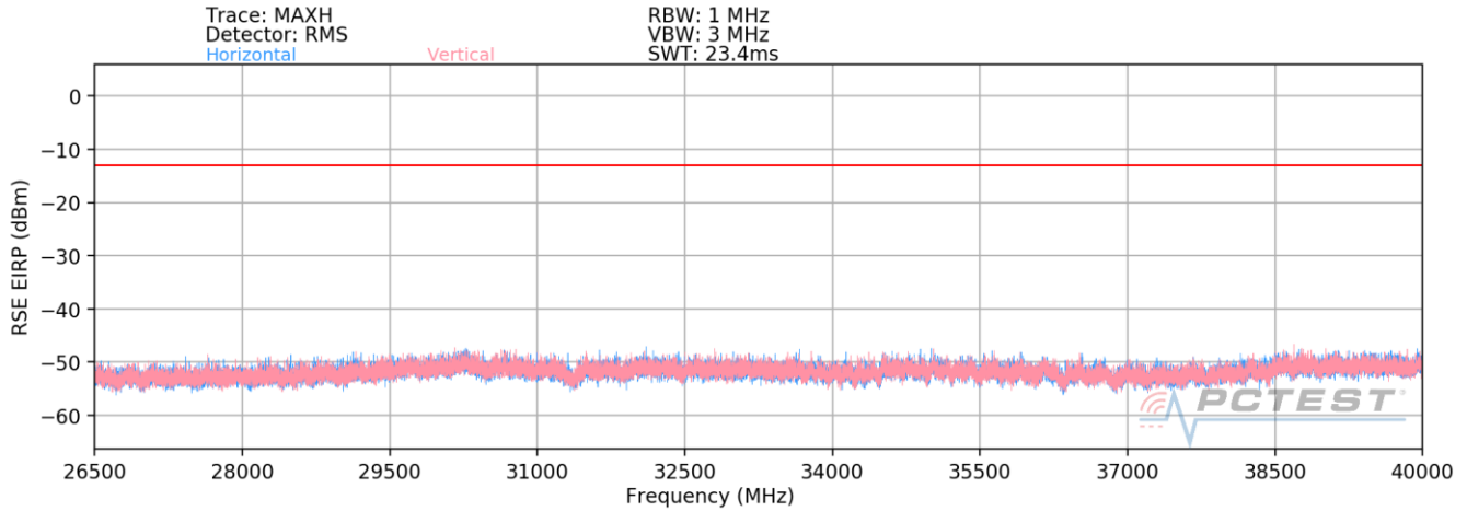
Plot 7-7. Radiated Spurious Plot (LTE Band 8 / LTE Band 8 / 5GHz)
