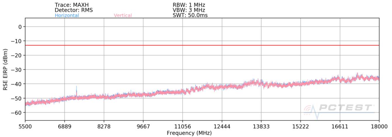
Plot 7-23. Radiated Spurious Plot (LTE Band 12 (cond) / LTE Band 8 (rad) / 2.4GHz)
