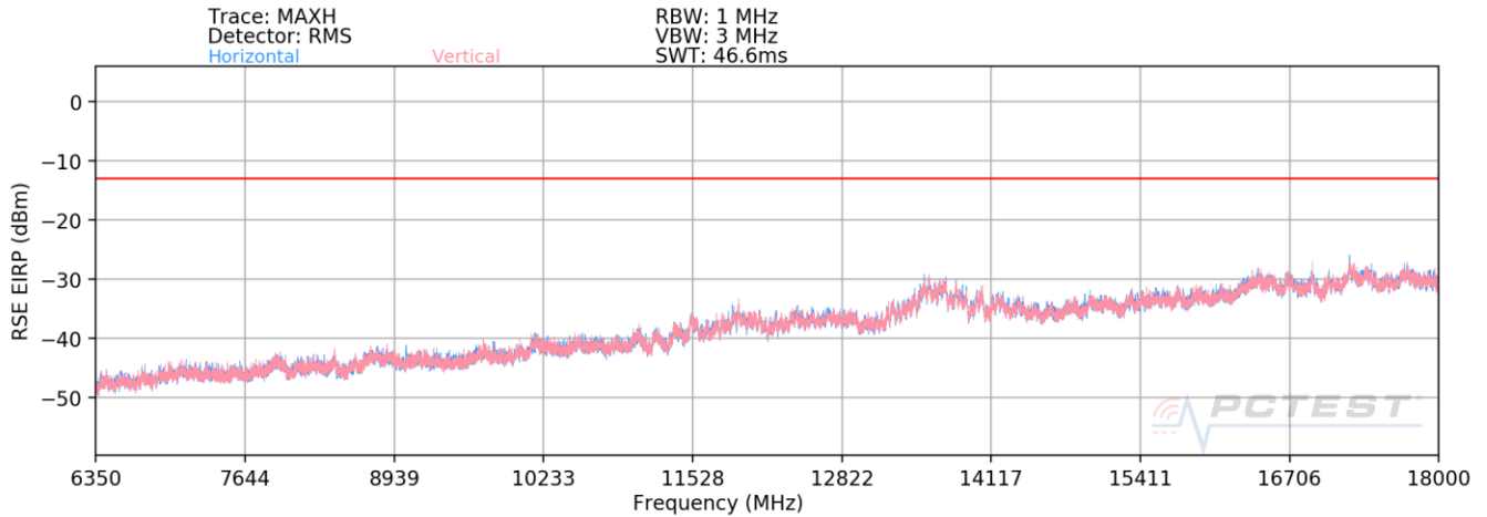
Plot 7-13. Radiated Spurious Plot (LTE Band 8 (rad) / LTE Band 12 (cond) / 5GHz)
