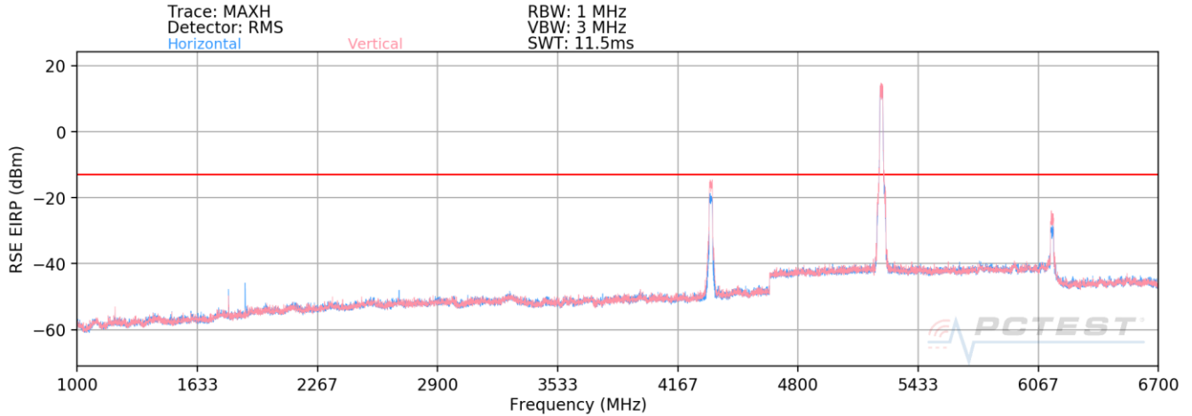
Plot 7-4. Radiated Spurious Plot (LTE Band 8 / LTE Band 8 / 5GHz)
