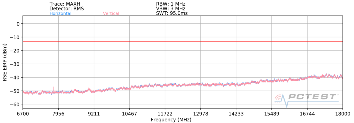
Plot 7-21. Radiated Spurious Plot (LTE Band 8 (rad) / LTE Band 41 (cond) / 5GHz)
