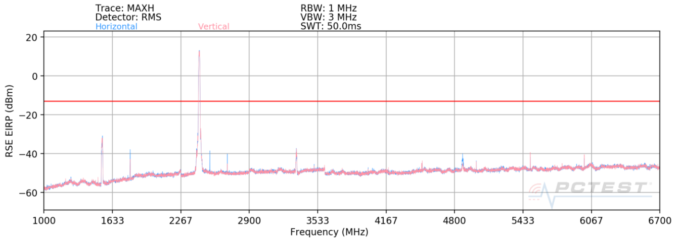
Plot 7-18. Radiated Spurious Plot (LTE Band 8 (rad) / LTE Band 7 (cond) / 2.4GHz)
