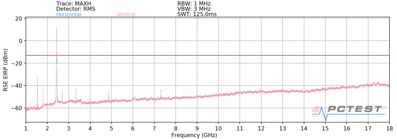
Plot 7-3. Radiated Spurious Plot (LTE Band 8 / LTE Band 8 / 2.4GHz)
