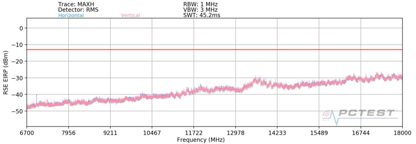
Plot 7-27. Radiated Spurious Plot (LTE Band 4 (cond) / LTE Band 8 (rad) / 2.4GHz)
