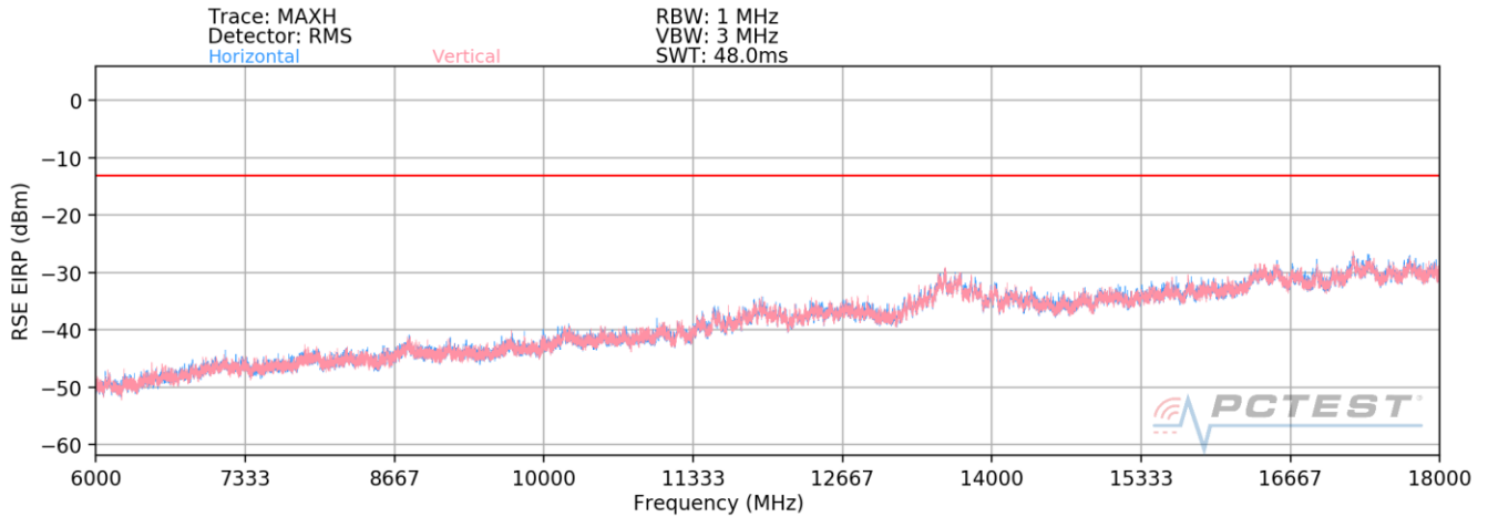
Plot 7-11. Radiated Spurious Plot (LTE Band 8 / LTE Band 13 / 2.4GHz)
