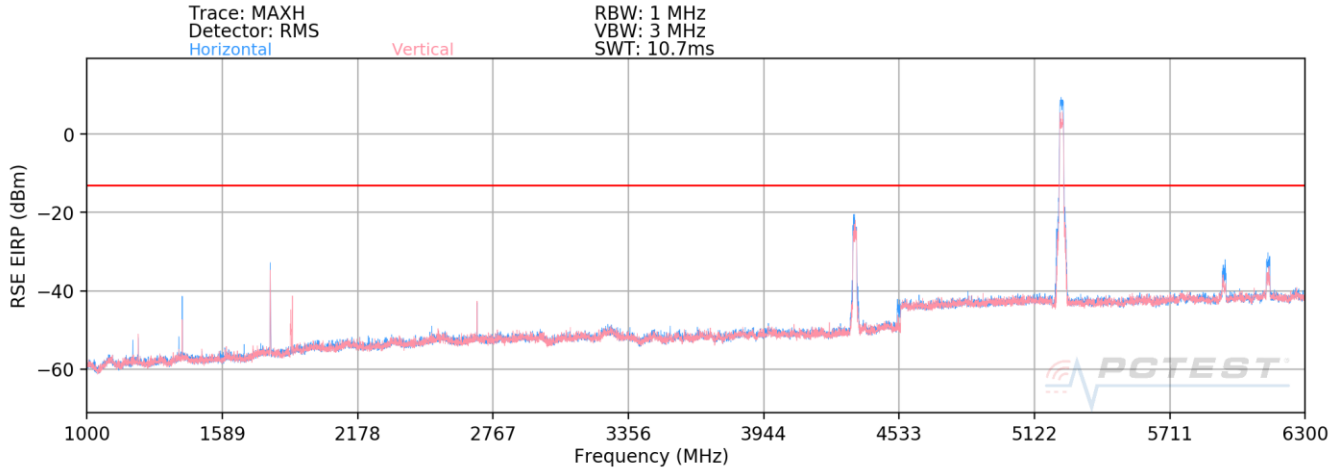
Plot 7-24. Radiated Spurious Plot (LTE Band 12 (cond) / LTE Band 8 (rad) / 5GHz)
