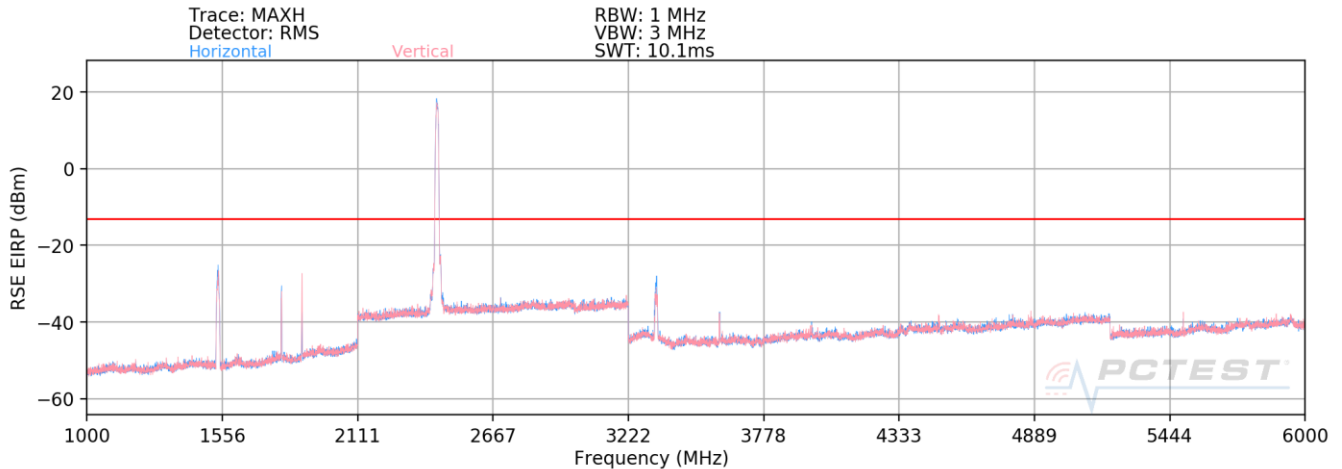
Plot 7-14. Radiated Spurious Plot (LTE Band 8 (rad) / LTE Band 25 (cond) / 2.4GHz)
