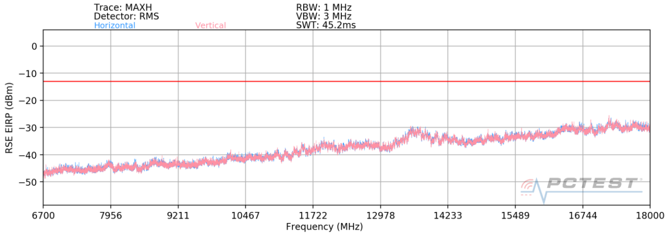
Plot 7-5. Radiated Spurious Plot (LTE Band 8 / LTE Band 8 / 5GHz)
