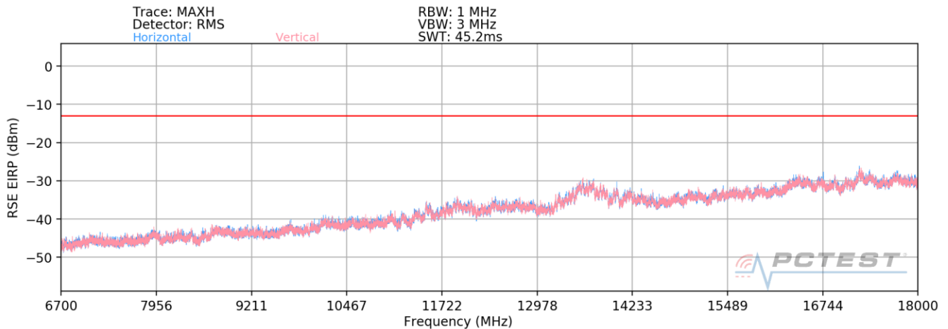
Plot 7-9. Radiated Spurious Plot (LTE Band 8 / LTE Band 8 / 5GHz)
