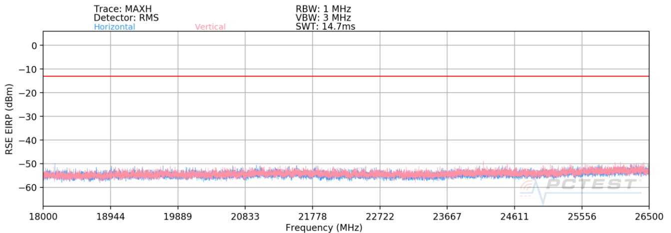
Plot 7-6. Radiated Spurious Plot (LTE Band 8 / LTE Band 8 / 5GHz)
