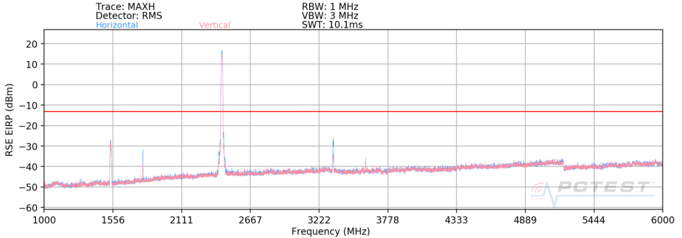
Plot 7-10. Radiated Spurious Plot (LTE Band 8 / LTE Band 13 / 2.4GHz)
