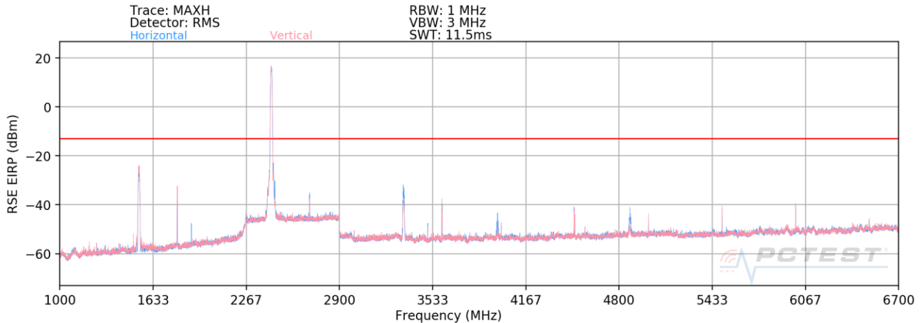
Plot 7-1. Radiated Spurious Plot (LTE Band 8 / LTE Band 8 / 2.4GHz)
