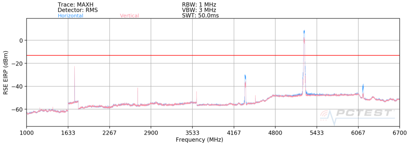
Plot 7-16. Radiated Spurious Plot (LTE Band 8 (rad) / LTE Band 4 (cond) / 5GHz)
