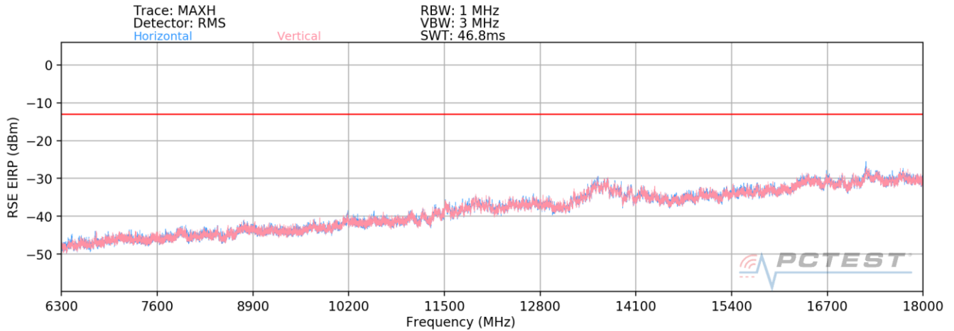
Plot 7-25. Radiated Spurious Plot (LTE Band 12 (cond) / LTE Band 8 (rad) / 5GHz)
