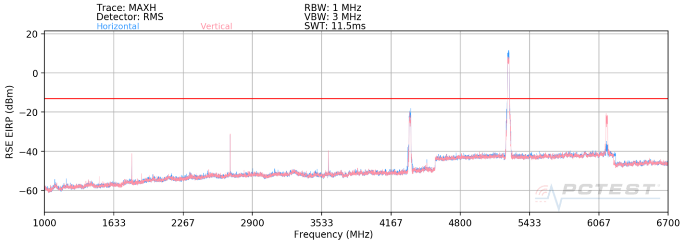
Plot 7-8. Radiated Spurious Plot (LTE Band 8 / LTE Band 8 / 5GHz)
