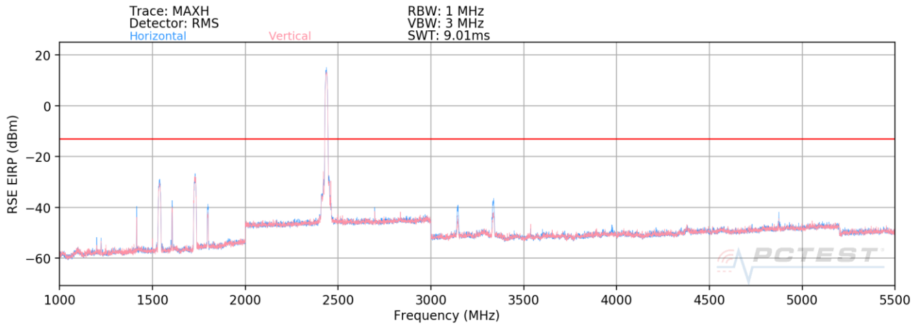
Plot 7-22. Radiated Spurious Plot (LTE Band 12 (cond) / LTE Band 8 (rad) / 2.4GHz)
