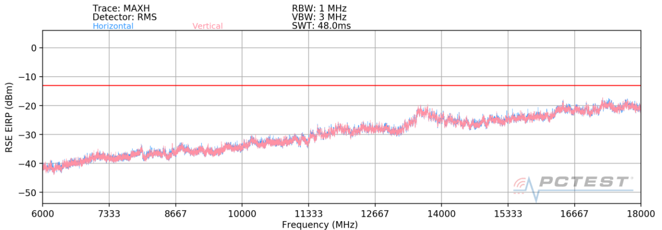
Plot 7-15. Radiated Spurious Plot (LTE Band 8 (rad) / LTE Band 25 (cond) / 2.4GHz)
