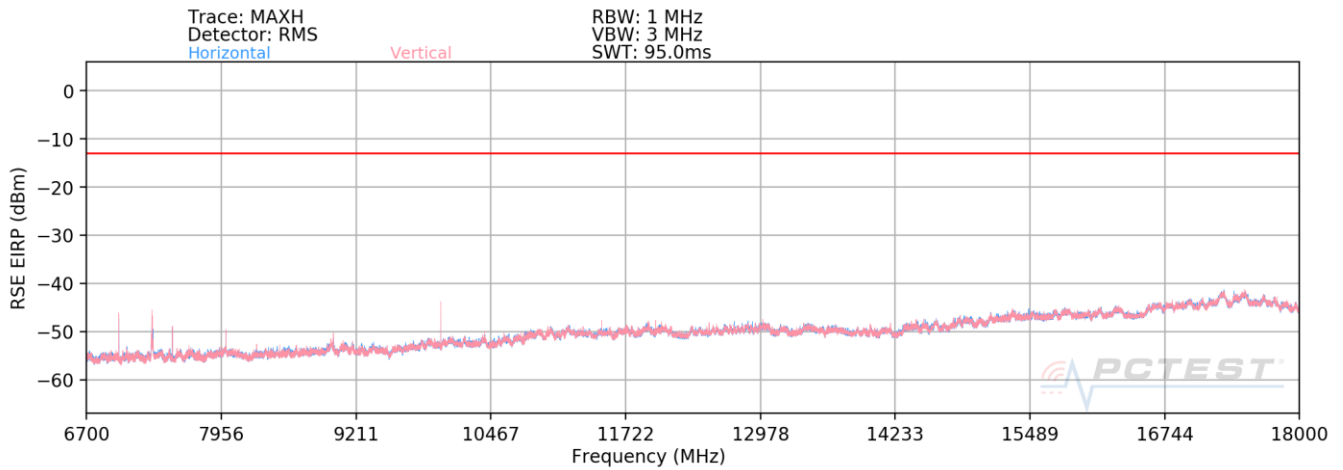
Plot 7-19. Radiated Spurious Plot (LTE Band 8 (rad) / LTE Band 7 (cond) / 2.4GHz)
