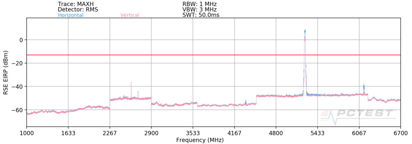
Plot 7-20. Radiated Spurious Plot (LTE Band 8 (rad) / LTE Band 41 (cond) / 5GHz)
