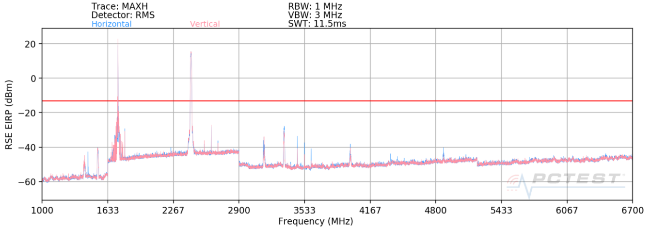
Plot 7-26. Radiated Spurious Plot (LTE Band 4 (cond) / LTE Band 8 (rad) / 2.4GHz)
