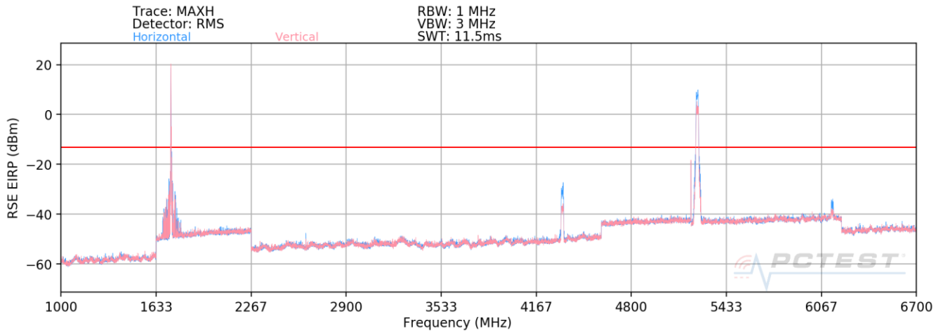
Plot 7-28. Radiated Spurious Plot (LTE Band 4 (cond) / LTE Band 8 (rad) / 5GHz)
