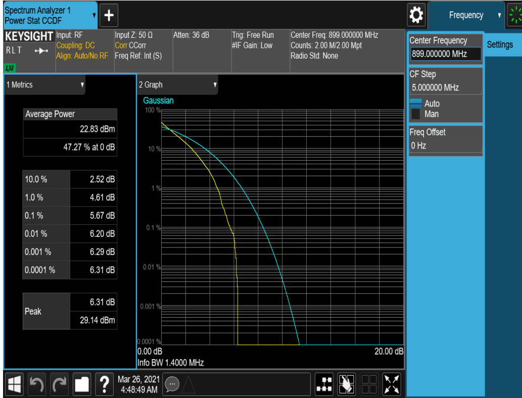
Plot 7-15. Peak to Average Ratio (1.4 MHz, QPSK, 6 RB, 0 Offset)
