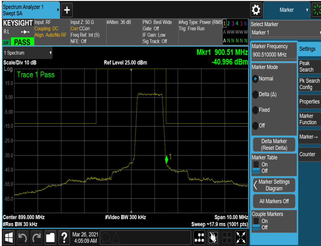
Plot 7-8. Upper Band Edge Plot (1.4 MHz, QPSK, 6 RB, 0 Offset)
