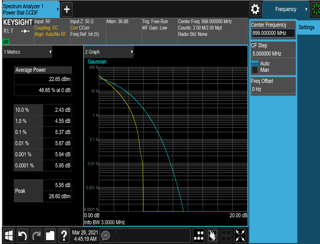
Plot 7-13. Peak to Average Ratio (3 MHz, QPSK, 15 RB, 0 Offset)
