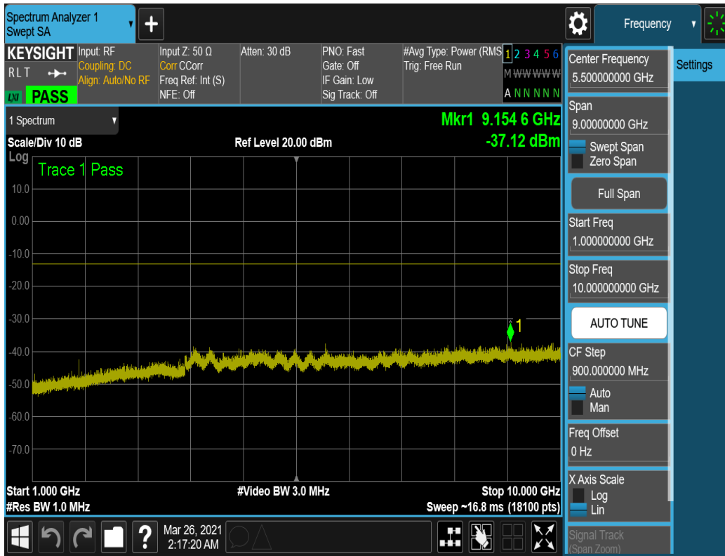
Plot 7-12. Conducted Spurious Plot – Mid Channel (3 MHz, QPSK, 1 RB, 14 Offset)
