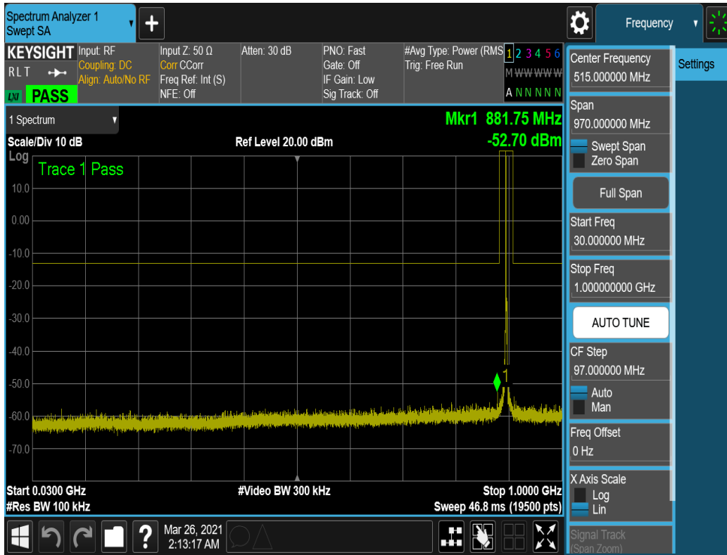
Plot 7-9. Conducted Spurious Plot – Mid Channel (3 MHz, QPSK, 1 RB, 0 Offset)
