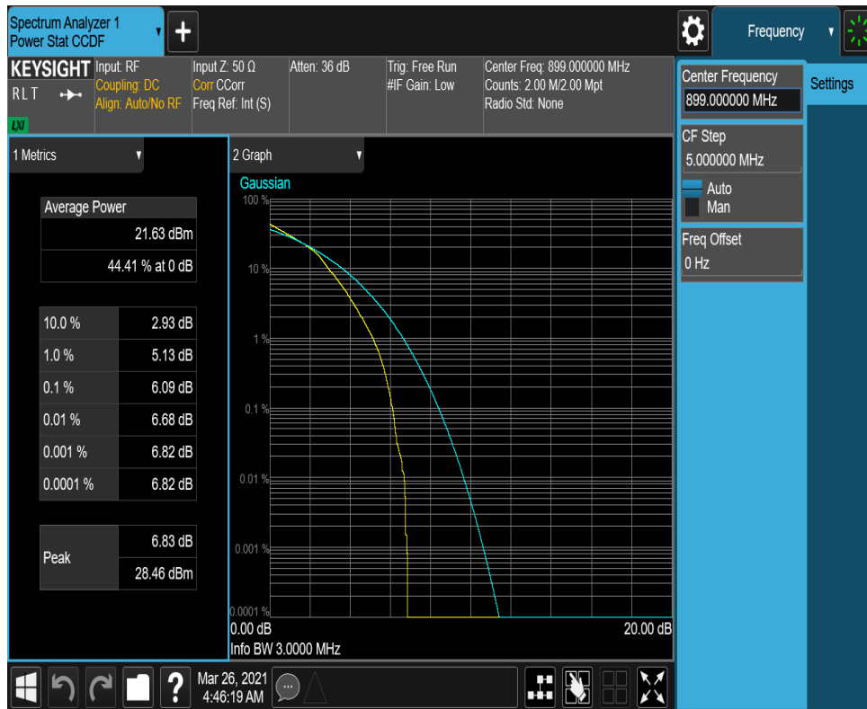
Plot 7-14. Peak to Average Ratio (3 MHz, 16QAM, 15 RB, 0 Offset)
