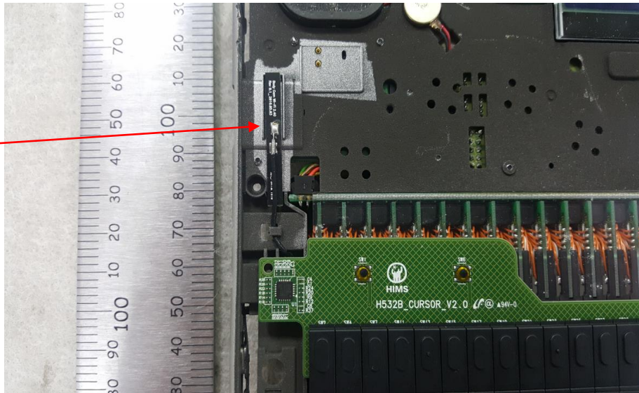
Bluetooth Module 1 ANT, Bluetooth Low Energy
