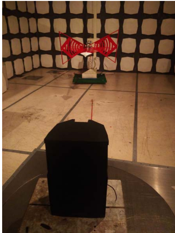
RE 30MHz-1GHz
