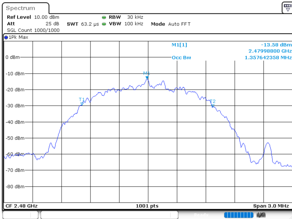
-20 dB BW NVNT 3-DH5 2480MHz Ant2
