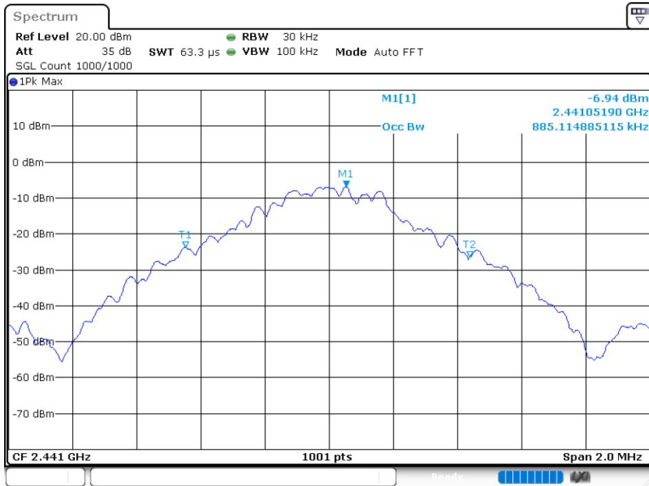
-20 dB BW NVNT 1-DH5 2441MHz Ant2
