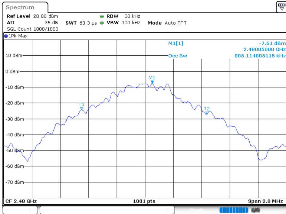
-20 dB BW NVNT 1-DH5 2480MHz Ant2
