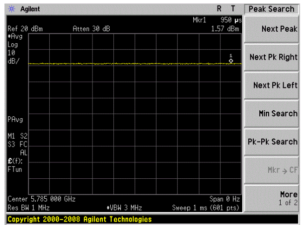
(802.11 AC20) channel 157
