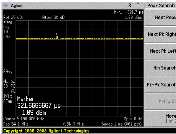
(802.11 AC40) channel 38
