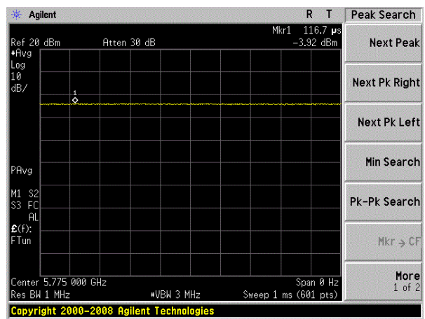
(802.11 AC80) channel 155
